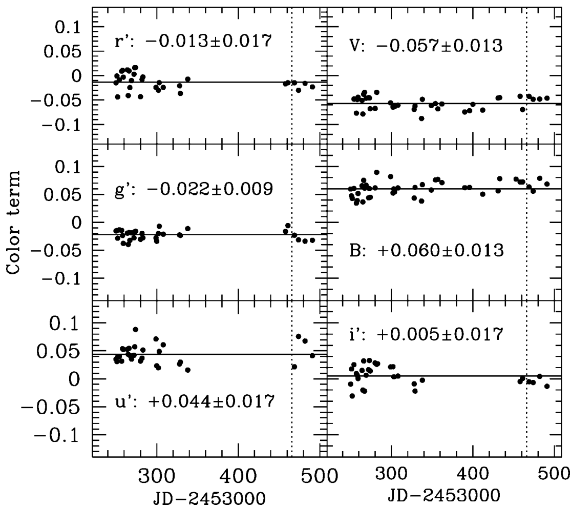
FIG. 4.—Color terms for the u'g'r'i'BV filters as a function of time. The average color term is plotted with a horizontal line, and its numerical value is indicated in each panel, along with the rms scatter. The vertical dotted line shows the time when the primary mirror of the 1 m telescope was washed.
