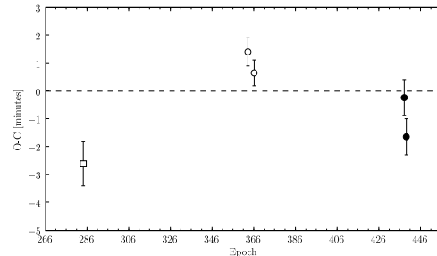
FIG. 3.— Observed-minus-calculated times (in minutes) for the transits of planet OGLE-TR-111b in front of its host star. The filled circles are the new transits presented in this work, the empty circles are from W07 and the empty square is the transit presented by Minniti et al. (2007), which has been reprocessed for this work.
