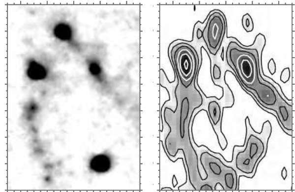
Fig. 4. Comparison between the VISIR narrow band 12.8\mu\text{m} filter image (left) and the 3.5cm map (right) by Morganti et al. (1999) for a 10''\times 14'' region including the AGN (bottom source on the left image), the three embedded YMCs and the MIR/cm ring. North is up, East is to the left. The ticks along the axis are drawn with 0.5'' intervals.
