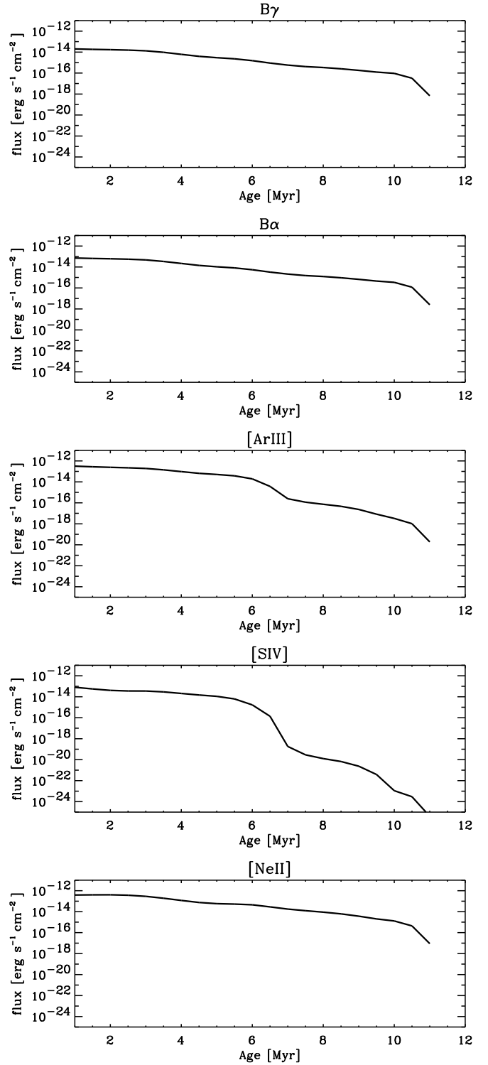
Fig. 15. Predicted line fluxes for the model described in Sec. 4.2. From top to bottom: B_{\gamma} , B_{\alpha} , [ArIII], [SIV] and [NeII]. The X-axis displays the age in Myr and the Y-axis provides the line flux, at the distance of NGC1365, corresponding to a 10^6 M_{\odot} cluster
