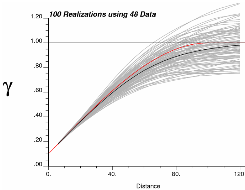
Figure 3 Post-simulation check for variogram reproduction based on 100 realizations using 48 data. The red variogram shows the input model, the black line shows the average variogram of the simulated realizations, and the gray lines correspond to the variogram from each of the 100 realizations.
