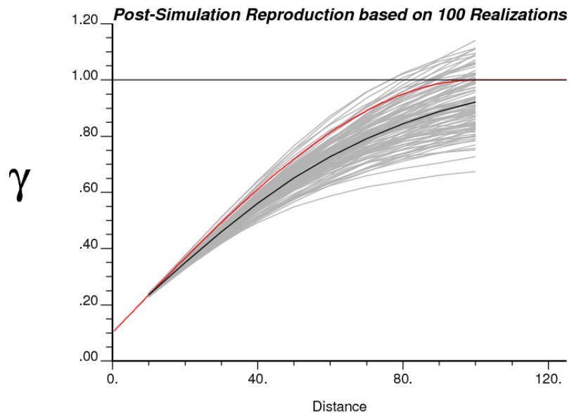
Figure 2 Post-simulation check for variogram reproduction based on 100 realizations. The red variogram shows the input model, the black line shows the average variogram of the simulated realizations, and the gray lines correspond to the variogram from each of the 100 realizations.
