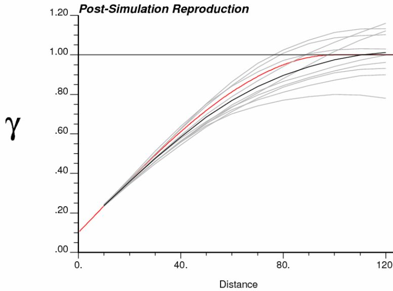
Figure 1 Post-simulation check for variogram reproduction based on 10 realizations. The red variogram shows the input model, the black line shows the average variogram of the simulated realizations, and the gray lines correspond to the variogram from each of the 10 realizations.
