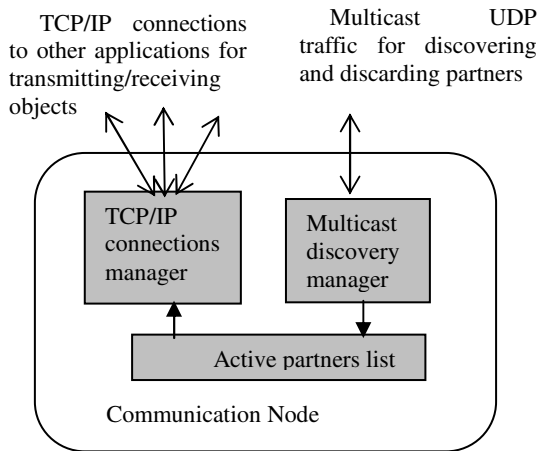
Fig. 1. The communication node
