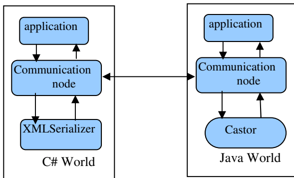
Fig. 2. Serializing and transmitting objects
