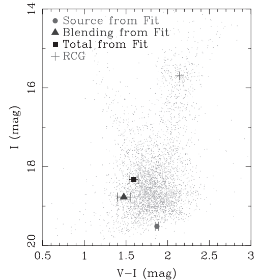
Figure 3. OGLE ( V - I, I ) color-magnitude diagram around OGLE-2007-BLG-368. The filled circle and triangle indicate the source and blended light from the fit, respectively. The filled square represents the total flux of the source and blend. Here the errors in I are too small to be visible. The cross indicates the center of the RCG.
