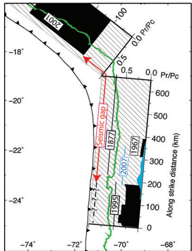
Figure 8. Seismic potency deficit along strike in the North Chile–South Peru subduction zone after the Tocopilla earthquake. Striped area represents interseismic potency cumulated (Pc) since 1877 in the North Chile gap and 1968 in the South Peru gap for a 100 per cent locking of the thrust interface between the Nazca and South American plates during the interseismic period and 6.4 \text{ cm yr}^{-1} of convergence rate (Angermann et al. , 1999). Blue area represents the seismic potency released (Pr) during the 2007 Tocopilla main shock, its two M_w \geq 6 aftershocks on 2007 November 15 and the two post-seismic periods studied (cGPS-post1 and cGPS-post2). Black areas represent the seismic potency released during other M_w \geq 7 earthquakes occurred in the region (see Fig. 1). Note that several M_w \geq 7 in the region of Antofagasta ( M_w 7.5 1987, M_w 7.0 1988, M_w 7.2 1988 and M_w 7.1 1998) are included in the Pr estimation, although they are not labelled. In the case of the 1995 Antofagasta, 2001 Arequipa and 2007 Tocopilla earthquakes, the seismic potency released during the post-seismic period is also included (20 per cent of the coseismic moment for the M_w 8.1 Antofagasta earthquake, Chlieh et al. 2004; Pritchard & Simons 2006; 40 per cent of the coseismic moment for the M_w 8.4 Arequipa earthquake, Ruegg et al. 2001; Melbourne et al. 2002; Pritchard 2003; 5 per cent of the coseismic moment for the 2007 Tocopilla earthquake, this work). Question marks indicate that the potency cumulated before the 1995 earthquake is uncertain in this region Coastline (green line) and trench (barbed line) have been superposed as reference.
