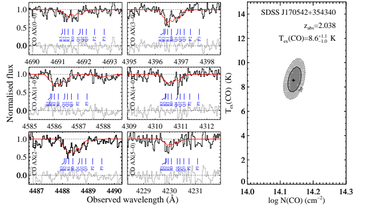
Fig. 3. Same as Fig. 2 for the system at z_{\text{abs}} = 2.038 toward SDSS J170542+354340 (best-fit model: \log N=14.14 , T_{\text{ex}}=8.6 \text{ K} ).
