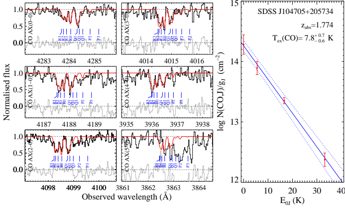
Fig. 1. Left: A^1\Pi(v') \leftarrow X^1\Sigma^+(v=0) electronic bands of CO detected at z_{\text{abs}} = 1.774 toward the quasar SDSS J104705+205734. The modelled profile is over-plotted in red with the fitting residuals shown in grey. Short vertical lines indicate the branch ('R', 'P' or 'Q') and the rotational level of the transition ( J=0-3 ). Right: The corresponding excitation diagram of CO gives the column density of the rotational levels J weighted by their quantum degeneracy ( g_j ) versus the energy of these levels relative to the ground state. The excitation temperature is directly given by -1/(a \ln 10) where a is the slope of the linear fit (solid blue line, with 1\sigma errors represented by the dotted curves).
