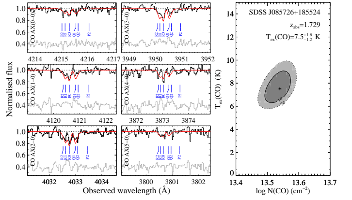
Fig. 2. Left: The CO electronic absorptions from the system at z_{\text{abs}} = 1.729 toward SDSS J085726+185524 are plotted together with the best-fit model ( \log N=13.54 , T_{\text{ex}}=7.5 \text{ K} , red profile). Right: Confidence contours (solid: 1\sigma , dotted: 2\sigma ) for the excitation temperature vs the total CO column density.
