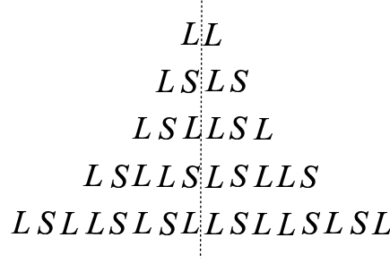
Figure 4.1: The Fibonacci tiling
