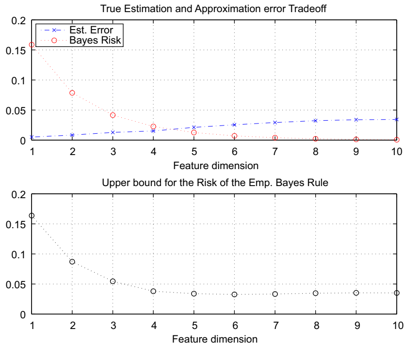
Fig. 2. Same description as Fig. 1. These results were obtained for N=10,000 i.i.d. realizations of the class conditional densities.
