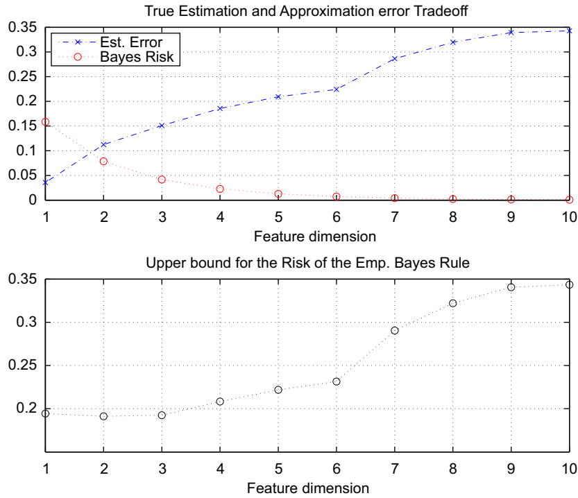
Fig. 1. The top figure reports the trend of the estimation error \Delta g_{MAP}(\hat{P}_{X_i|Y}) and the approximation error L_{X_i} as a function of the space dimensionality, for a dimensionally embedded space sequence. The bottom figure shows the sum of the two error terms, i.e., \Delta g_{MAP}(\hat{P}_{X_i|Y}) + L_{X_i} , as a function of the space dimensionality. These results were obtained for N=100 i.i.d. realizations of the class conditional densities.
