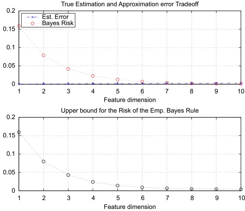
Fig. 3. Same description as Fig. 1. These results were obtained for N=1,000,000 i.i.d. realizations of the class conditional densities.
