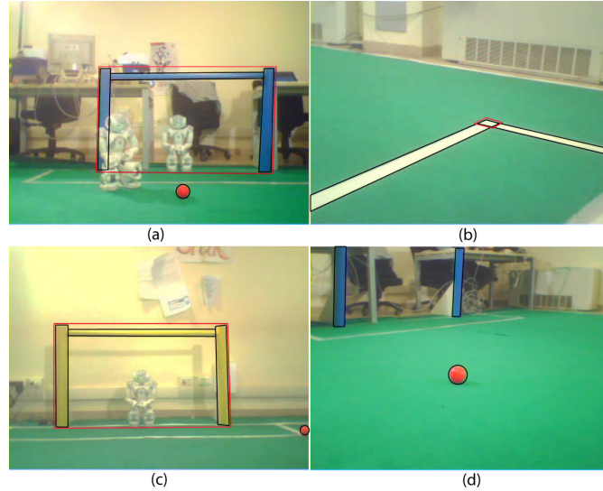
Fig. 2. Labeling objects of interest. (a),(c) both entire goals and its parts are labeled using quadrilaterals, as well as lines and corners (b); (d) ellipses are used to label the ball
