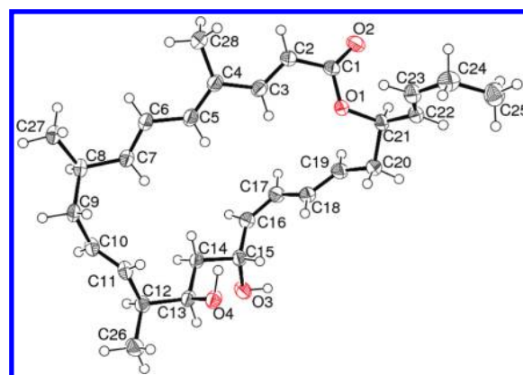
Figure 3. Molecular structure of 1 showing 50% displacement ellipsoids.
