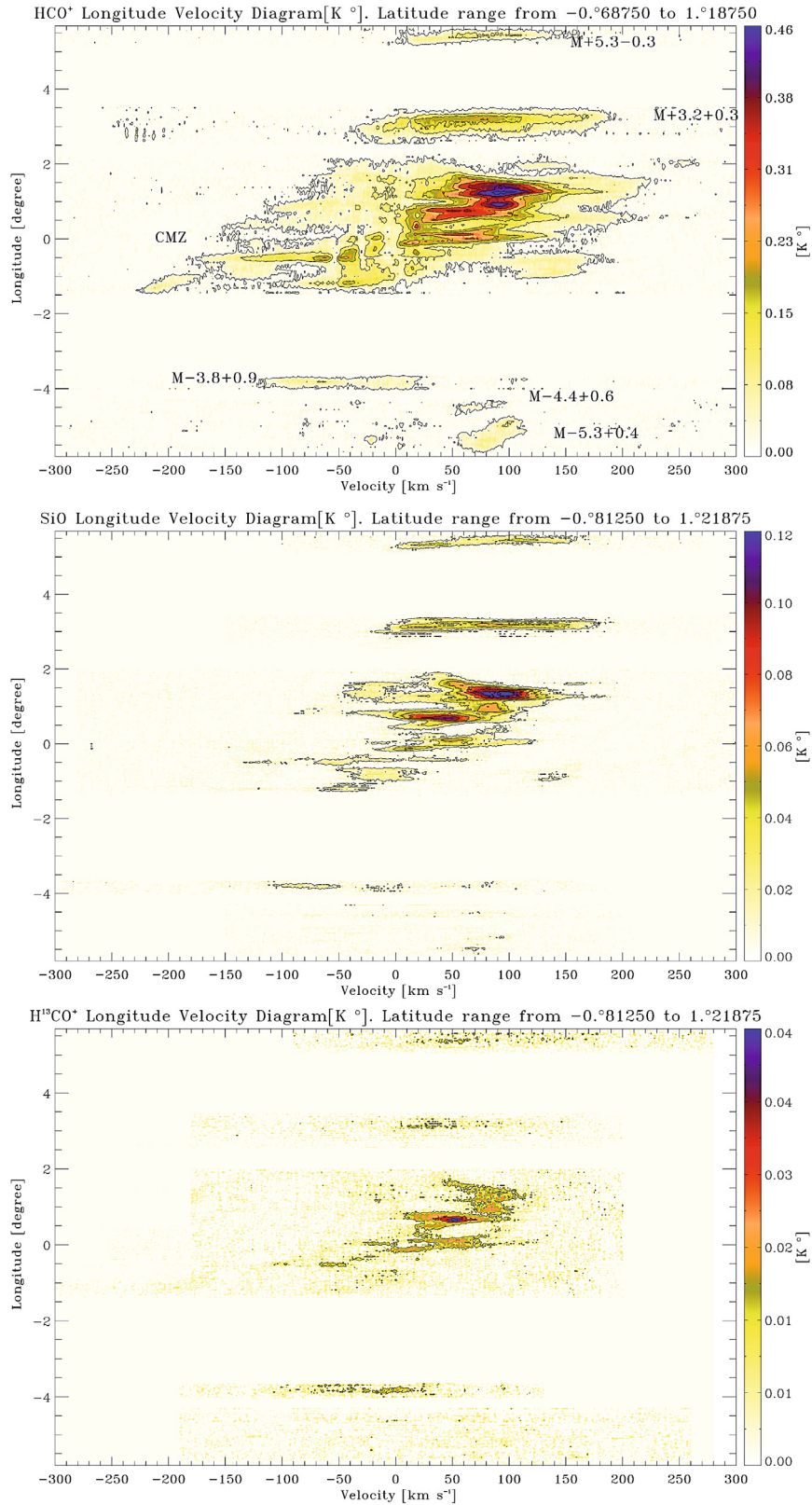
Fig. 3. Top: longitude-velocity diagram of HCO + emission from the CMZ and PMZ covering the whole survey in the latitude range between b = -0^{\circ}6875 to b = 1^{\circ}1875 . The contour levels start at 0.021 K ( 3\sigma ), and increase in steps of 0.058 K ( 8\sigma ). Middle: longitude-velocity diagram of SiO emission from the CMZ and PMZ covering the whole survey in the latitude range between b = -0^{\circ}8125 to b = 1^{\circ}21875 . The contour levels start at 0.01 K ( 3\sigma ), and increase in steps of 0.018 K ( 5\sigma ). Bottom: longitude-velocity diagram of H 13 CO + emission from the CMZ and PMZ covering the whole survey in the latitude range between b = -0^{\circ}8125 to b = 1^{\circ}21875 . The contour levels start at 0.009 K ( 3\sigma ), and increase in steps of 0.016 K ( 5\sigma ).
