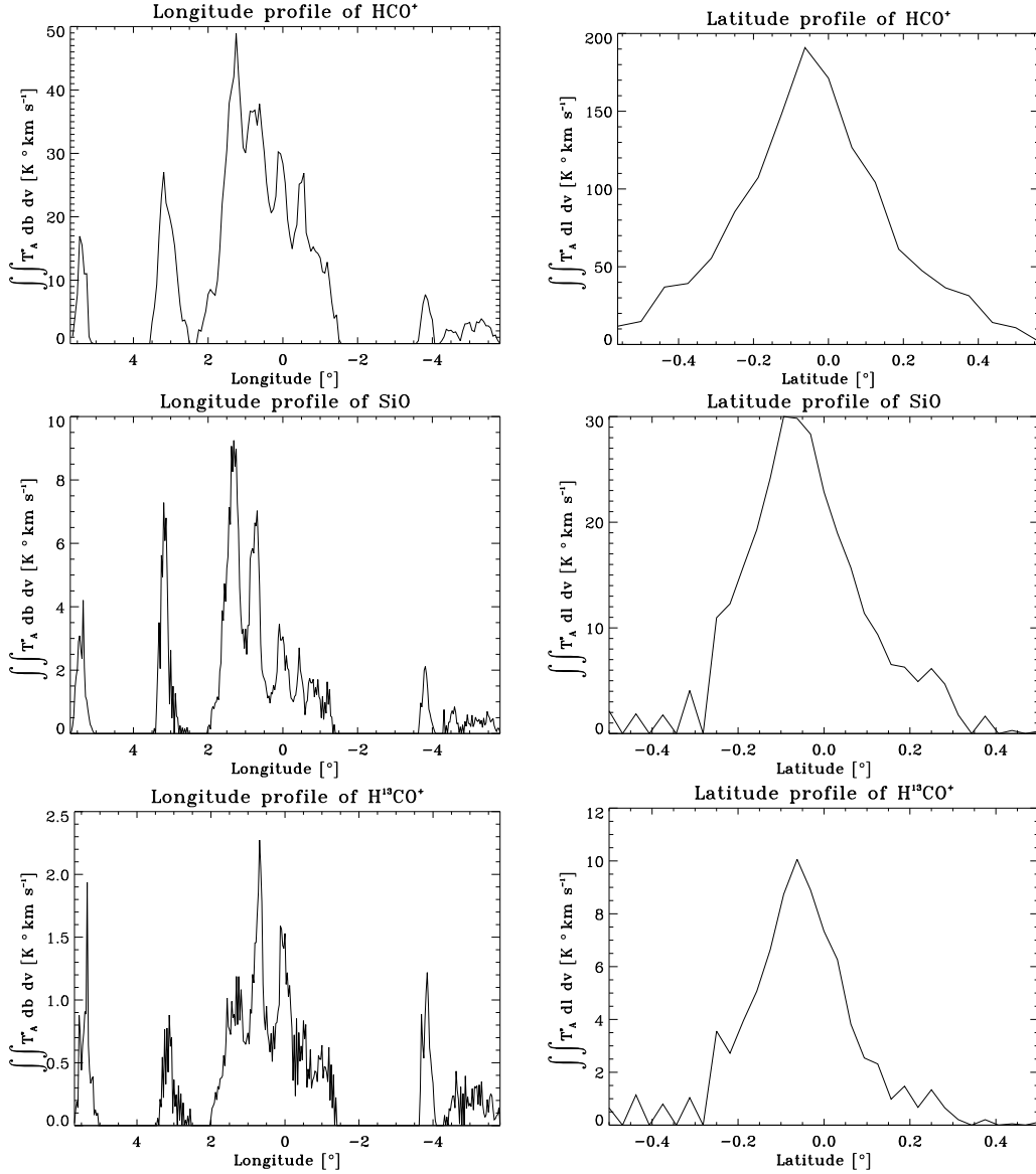
Fig. 4. Left: longitude profile for the entire latitude range observed in \text{HCO}^+ ( top ), \text{SiO} ( middle ) and \text{H}^{13}\text{CO}^+ ( bottom ) emission. Right: latitude profile for entire longitude range observed of the CMZ ( -1:5 < l < 2:25 ) in \text{HCO}^+ ( top ), \text{SiO} ( middle ) and \text{H}^{13}\text{CO}^+ ( bottom ) emission.
