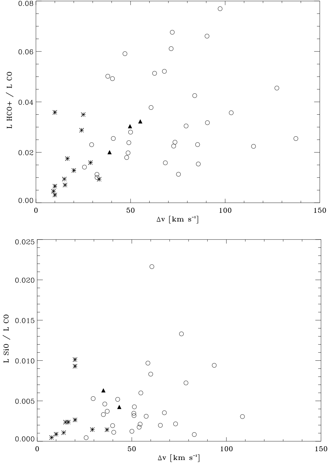
Fig. 10. Relationship between the luminosity ratio HCO + to CO ( top ) and the HCO + velocity width, and the luminosity ratio SiO to CO ( bottom ) and the SiO velocity width for each molecular cloud of the survey. Open circles denote Galactic center clouds, an asterisk the disk clouds, and filled triangles are clouds that probably are in an intermediate region, influenced by a bar, and that present large linewidth, probably due the strong Galactic center tidal forces in this region. There is a cloud (number 35 in SiO) with a large linewidth ( \sim 35 km s -1 ) in the bottom plot. This cloud is also not considered in our analysis owing to the poor fit (see Fig. E.8).
