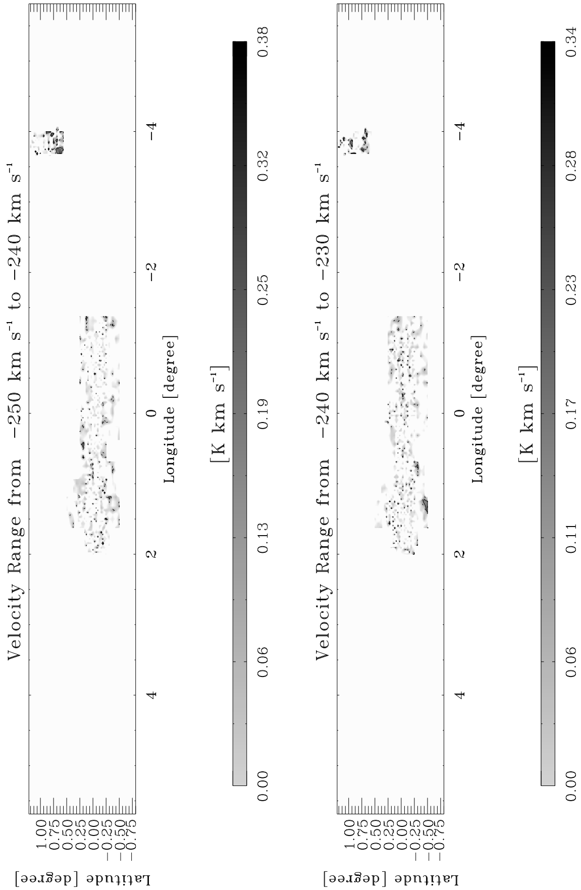
Fig. C1.1. The integrated intensity of the Galactic center region in \text{SiO} (1–0) in velocity intervals of 10 \text{ km s}^{-1} width. The solid contour levels start at 0.2 \text{ K} , which is the 3\sigma -level, and increase in steps of 0.66 \text{ K km s}^{-1} ( 10\sigma ). The dotted contour is at 0.13 \text{ K km s}^{-1} ( 2\sigma ).
