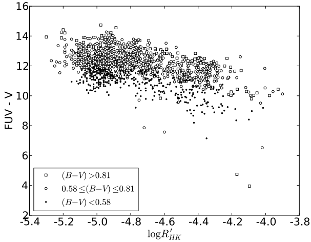
Fig. 2. FUV - V versus \log R'_{HK} for a sub-sample of 1360 stars.
