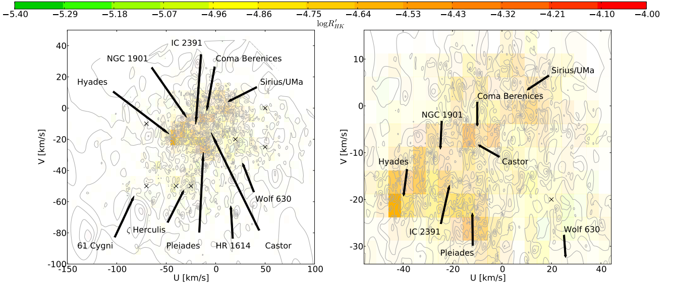
Fig. 3. Plot of the (U, V) velocity space showing contour levels of stellar activity ( \log R'_{\text{HK}} ) and the grid of boxes for the sample (left). The right panel shows a zoom of the central region where a higher density of stars is found. The transparency level indicates the density number of stars inside the boxes. The crosses mark the center of the Dehnen 7, 8, 9, 10, 11, 13, 14 groups.
