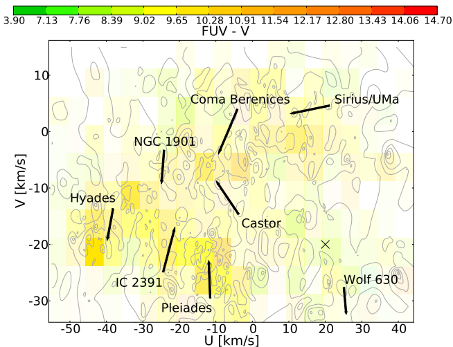
Fig. 4. Plot of the (U, V) region where a higher density of stars is found. Contour levels and grid of the FUV-V for a sample of 1360 stars are shown.
