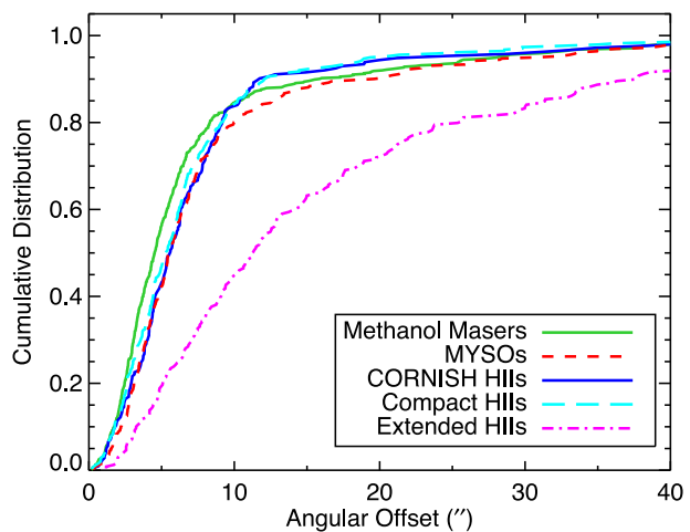
Figure 2. Left-hand panel: normalized source counts for the ATLASGAL–RMS matches are shown as a function of offset between their position and that of the peak of the submillimetre emission of their associated ATLASGAL source. We have truncated the x -axis of this plot at 40 arcsec as there are only 34 matches that have a larger angular separation ( \lesssim 80 arcsec) and the surface density effectively falls to zero. The bin size is 2 arcsec. Right-hand panel: cumulative distribution of angular offset of the methanol masers, MYSOs and H_{II} regions drawn from the MMB, AMGPS, CORNISH and RMS surveys.
