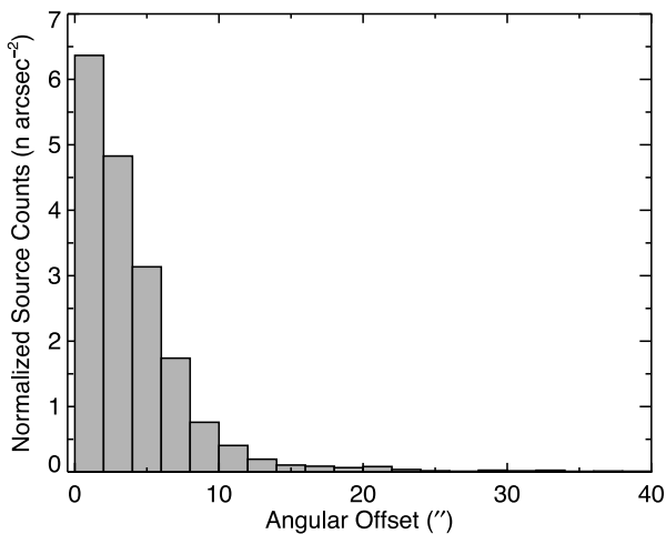
Figure 2. Left-hand panel: normalized source counts for the ATLASGAL–RMS matches are shown as a function of offset between their position and that of the peak of the submillimetre emission of their associated ATLASGAL source. We have truncated the x -axis of this plot at 40 arcsec as there are only 34 matches that have a larger angular separation ( \lesssim 80 arcsec) and the surface density effectively falls to zero. The bin size is 2 arcsec. Right-hand panel: cumulative distribution of angular offset of the methanol masers, MYSOs and H_{II} regions drawn from the MMB, AMGPS, CORNISH and RMS surveys.
