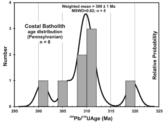
FIG. 5. Age probability plot for the Late Carboniferous Coastal Batholith granite to diorite samples between 30° and 40°S, Chile.
