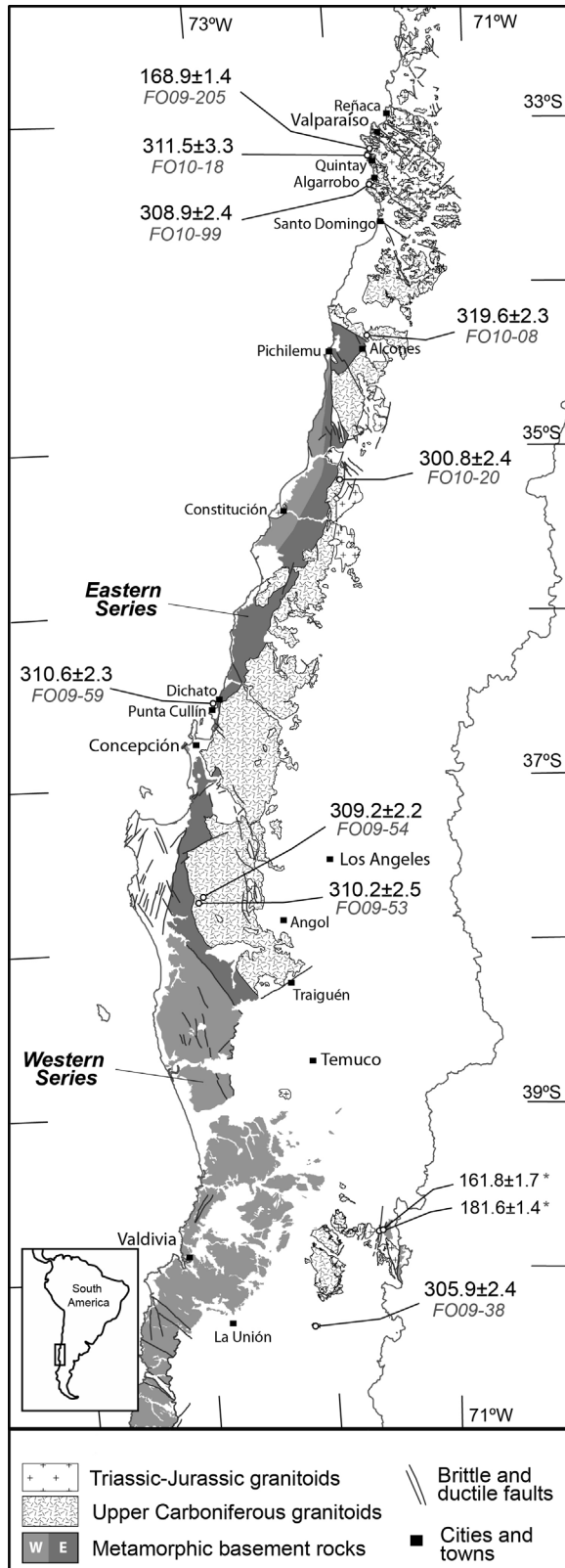
FIG. 1. Geological sketch map of central Chile between 33° and 40°S (modified from SERNAGEOMIN, 2003). Patterned zone represents the Coastal Batholith and rocks of the accretionary metamorphic prism. Additional age data are U-Pb zircon crystallization ages (*) of the plutonic protolith of gneisses from the main trace of the Liquiñe-Ofqui fault zone Hervé et al. , 2013).
