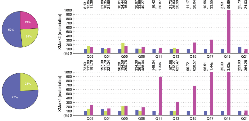
Fig. 16. Materialize : ratio of queries of group Structural for which each system obtained the best running times (left). Detailed performance analysis for a selection of queries over XMark2 and XMark4 (right).
