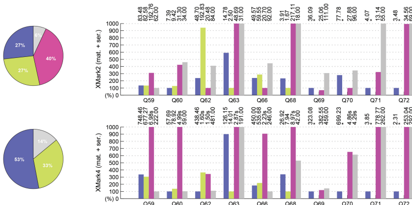
Fig. 26. Materialize + Serialize : ratio of queries of group Text for which each system obtained the best running times (left). Detailed performance analysis for a selection of queries over XMark2 and XMark4 (right).
