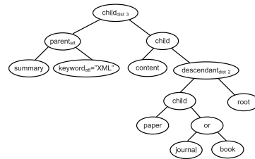
Fig. 6. Optimizations applied over a query parse tree until reaching the final query execution tree .
