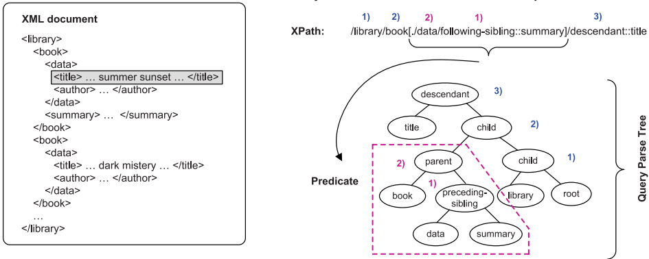
Fig. 5. Example of query parse tree.
