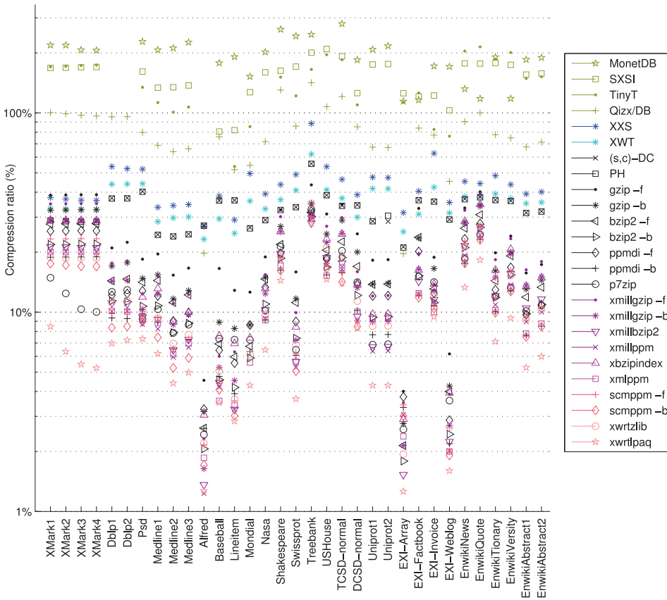
Fig. 10. Compression ratios achieved by our proposal (in blue), general text compressors (in black), XML conscious nonqueriable compressors (in pink), and queriable tools (in green) over different XML documents.
