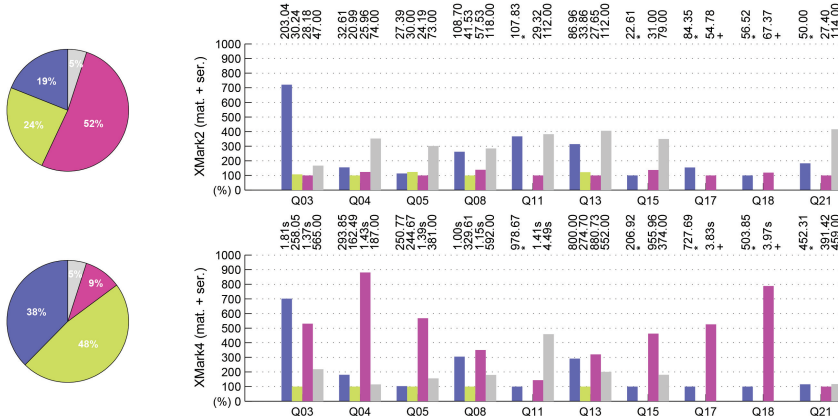
Fig. 17. Materialize + Serialize : ratio of queries of group Structural for which each system obtained the best running times (left). Detailed performance analysis for a selection of queries over XMark2 and XMark4 (right).
