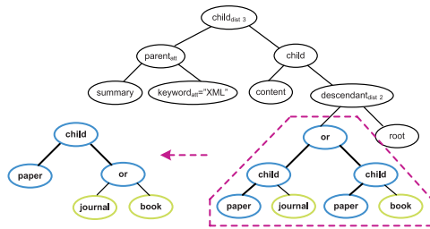
Fig. 6. Optimizations applied over a query parse tree until reaching the final query execution tree .
