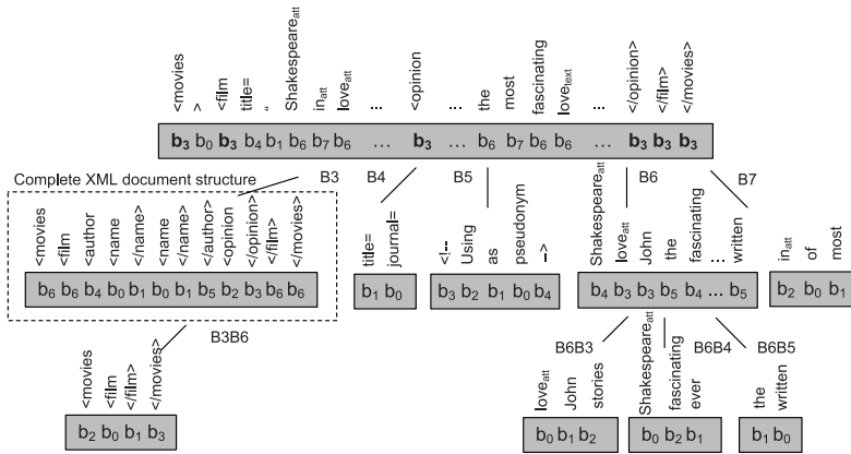
Fig. 2. Example of XWT structure built from an XML document.
