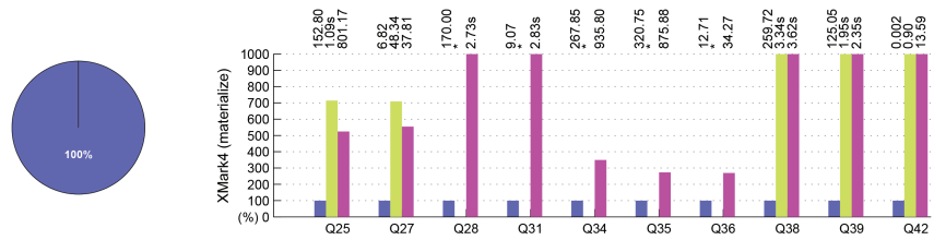
Fig. 19. Materialize : ratio of queries of group Wildcards for which each system obtained the best running times (left). Detailed performance analysis for a selection of queries over XMark4 (right).
