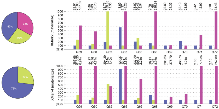
Fig. 25. Materialize : ratio of queries of group Text for which each system obtained the best running times (left). Detailed performance analysis for a selection of queries over XMark2 and XMark4 (right).
