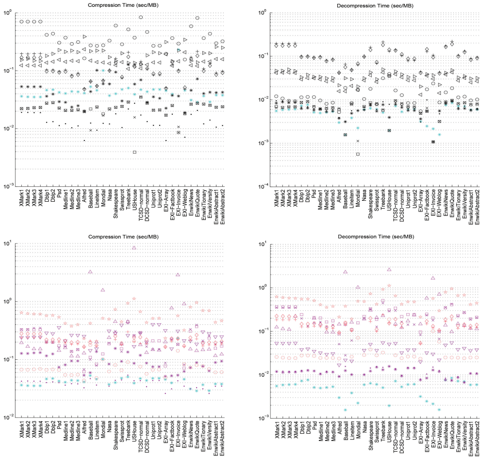
Fig. 11. Compression and decompression times. Comparison of XWT with general text compressors (top) and XML conscious nonqueriable compressors (bottom).
