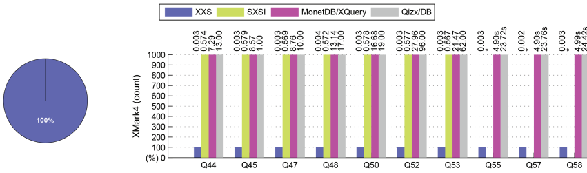
Fig. 21. Count : ratio of queries of group Names for which each system obtained the best running times (left). Detailed performance analysis for a selection of queries over XMark4 (right).
