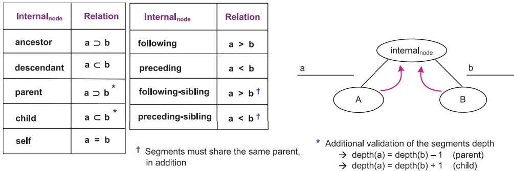
Fig. 7. Relations that compared segments must hold to satisfy the semantics of different XPath axes.
