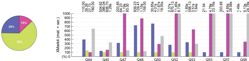
Fig. 23. Materialize + Serialize : ratio of queries of group Names for which each system obtained the best running times (left). Detailed performance analysis for a selection of queries over XMark4 (right).
