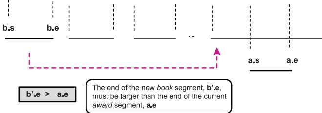
Fig. 9. Skipping of segments.
