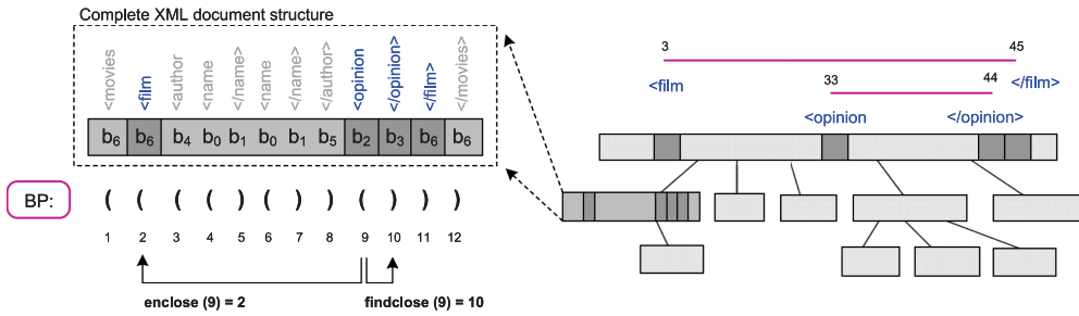
Fig. 3. Correspondence between the root of the XWT subtree storing the document structure and a balanced parentheses representation.
