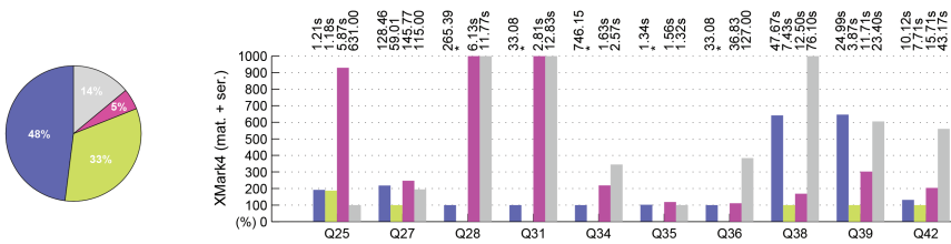
Fig. 20. Materialize + Serialize : ratio of queries of group Wildcards for which each system obtained the best running times (left). Detailed performance analysis for a selection of queries over XMark4 (right).
