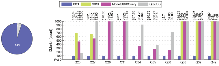
Fig. 18. Count : ratio of queries of group Wildcards for which each system obtained the best running times (left). Detailed performance analysis for a selection of queries over XMark4 (right).
