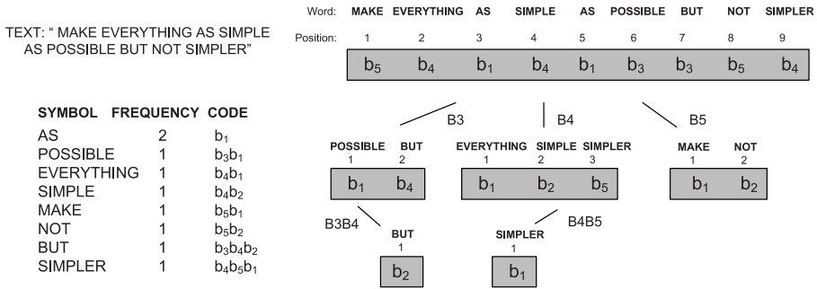
Fig. 1. Example of WTBC structure.
