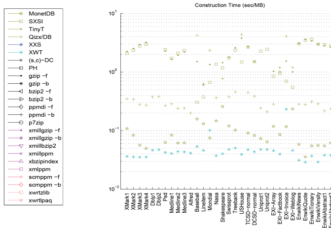
Fig. 12. Construction times of queriable solutions.
