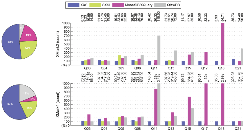
Fig. 15. Count : ratio of queries of group Structural for which each system obtained the best running times (left). Detailed performance analysis for a selection of queries over XMark2 and XMark4 (right).
