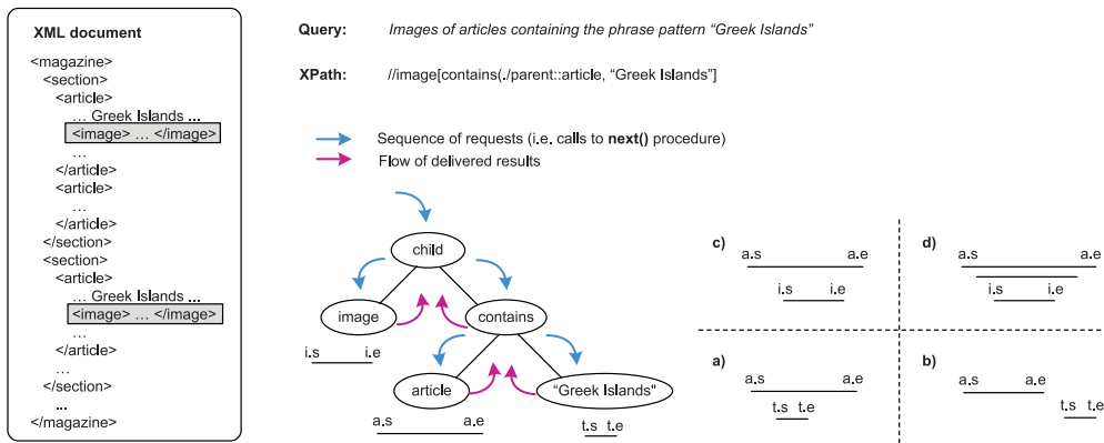
Fig. 8. General query evaluation scheme.
