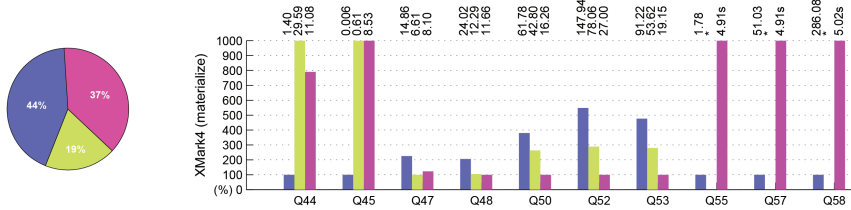
Fig. 22. Materialize : ratio of queries of group Names for which each system obtained the best running times (left). Detailed performance analysis for a selection of queries over XMark4 (right).
