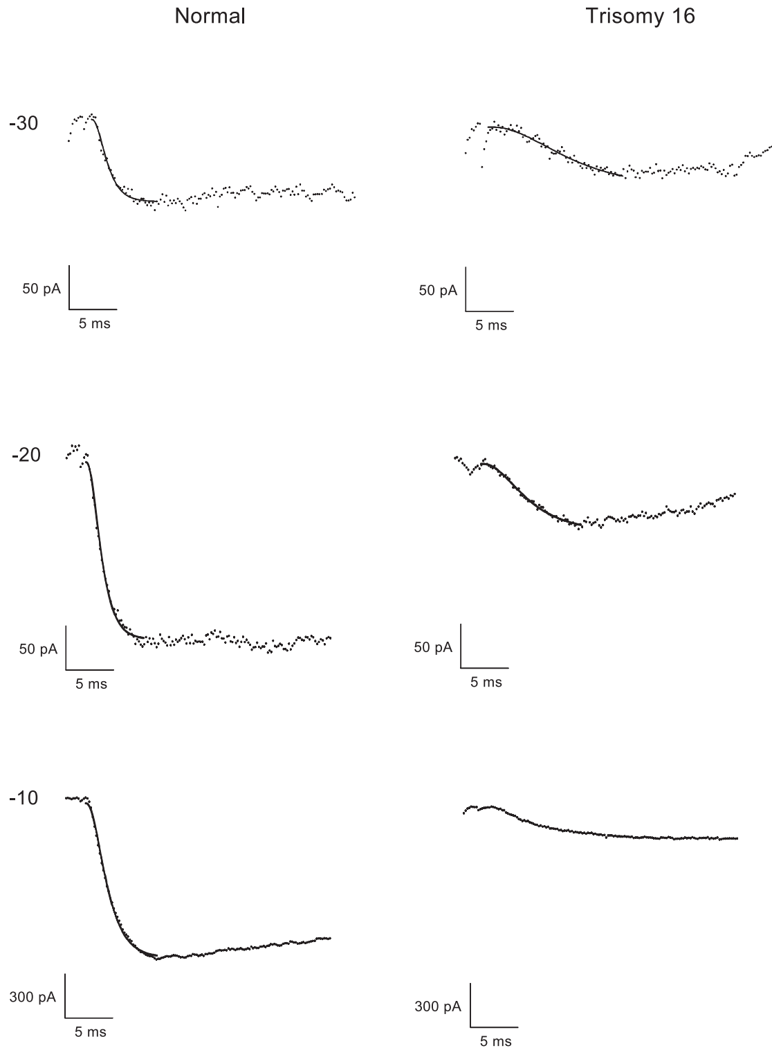
Figure 5. Exponential fits to the activation phase of \text{Ca}^{2+} currents in DRG neurons. Values noted represent membrane potential values, in mV. V_{\text{holding}} = -80 mV. The experimental trace is shown in dots; the fitted trace is superimposed in solid lines. The fitted region is taken from immediately after the small capacitive transient to the peak of the current. Note the slower time course in the trisomic condition.
