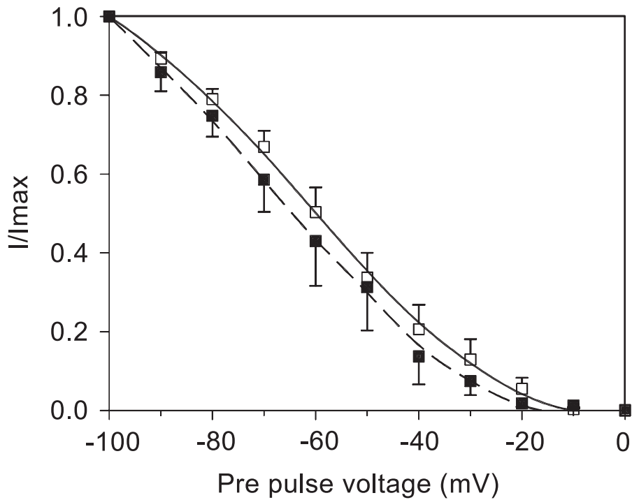
Figure 4. Voltage-dependent inactivation of \text{Ca}^{2+} currents. Values are normalized to peak current in each cell. No significant difference was observed at any pre-pulse potential level between the normal and trisomic condition. Points are means \pm S.E.M.
