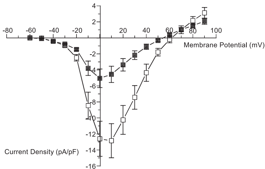
Figure 2. I-V curve of whole cell \text{Ca}^{2+} currents in normal and trisomic DRG neurons. Open squares represent normal cells ( n=18 ); closed squares represent Ts16 cells ( n=20 ). Points are means + S.E.M.
