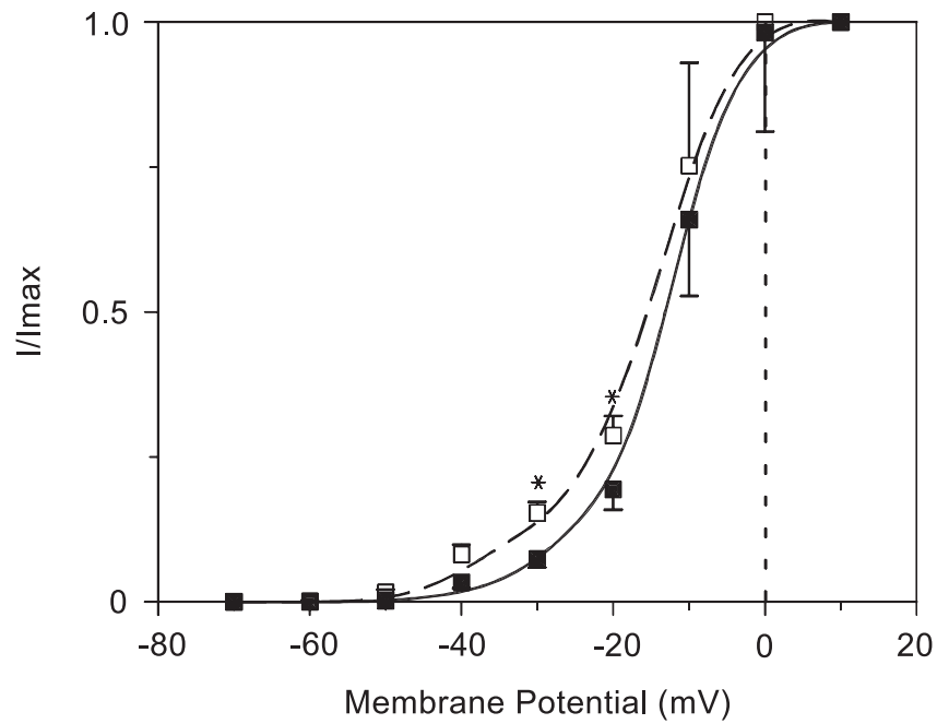
Figure 3. Voltage-dependent activation of \text{Ca}^{2+} currents. Values are normalized to peak current in each cell. Points are means \pm S.E.M. ( n=18 and 20 for normal and trisomic cells, respectively). * Significantly different for p<.05 .
