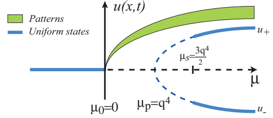
FIG. 7. (Color online) Bifurcation diagram of Swift-Hohenberg Eq. (21), where the darkened area accounts for the amplitude of the patterns. The continuous and dashed lines account for stable and unstable uniform states, respectively. \{\mu_0, \mu_p\} correspond to the spatial and the pitchfork bifurcations of the state u = 0 , respectively. \mu_s stands for the spatial bifurcation of the states u_{\pm} = \pm\sqrt{\mu - q^4} .
