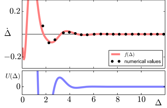
FIG. 10. (Color online) Kinematic law of the kink position as a result of size effect. Points are obtained numerically by considering a uniform distribution of initial conditions for a single kink, then numerically the system evolves in a brief moment of time, and finally the temporal variation of the kink position is calculated. The solid curve is obtained by using the integral form of the kinematic law of the kink position f(\Delta) = f_1' + f_2' + f_3' , using the expressions (27–29). The lower panel shows the potential U(\Delta) .
