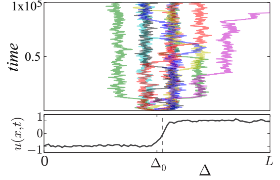
FIG. 12. (Color online) Stochastic dynamics of a kink state of the forcing real Ginzburg-Landau Eq. (33) with k = \pi/3 , a = 0.02 , and \eta = 0.02 . Different colors represent different trajectories of the kink solution. The bottom panel shows the profile of the kink at the initial time.
