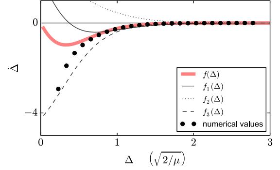
FIG. 4. (Color online) Kinematic law of the kink position as a result of size effect. Points are obtained numerically by considering a uniform distribution of initial conditions for a single kink, then numerically the system evolves during a brief moment of time, and finally the temporal variation of the kink position is calculated. The solid line is the analytical expression (13) with \eta = 0 , and f(\Delta) = f_1 + f_2 + f_3 .
