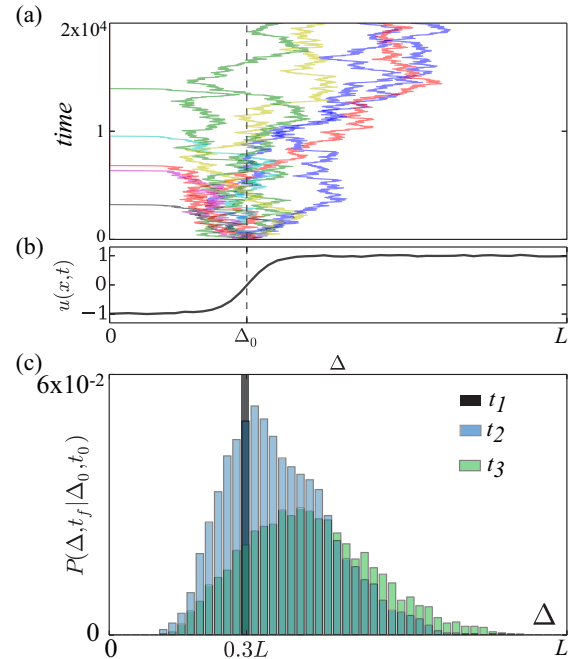
FIG. 3. (Color online) Stochastic dynamics of a kink state. (a) Numerical simulations of a single kink of Eq. (4) in a finite size system with specular boundary conditions, with \mu = 1 and \eta = 0.0018 and L = 25 , starting at the position \Delta = 0.3L . (b) The profile link at an initial moment. (c) Evolution of survival probability of a single kink for different instants of time, t_1 = 0 (black), t_2 = 20000 (blue), and t_3 = 40000 (green).
