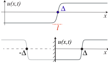
FIG. 2. (Color online) Domain solution between two symmetric states, kink solution (top), \{\Delta, l\} account for the position and the core of the kink. Bottom shows a kink and an antikink solution as consequence of the specular boundary condition.
