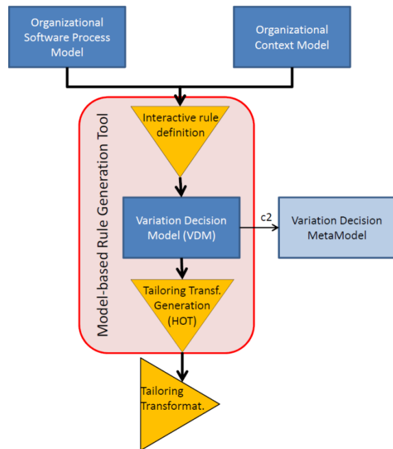
Figure 2: Architecture of the proposed heuristic.
