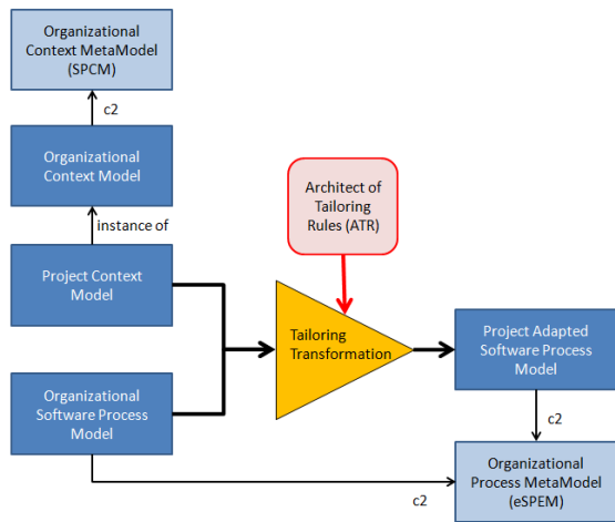
Figure 1: MDE-based software process tailoring.
