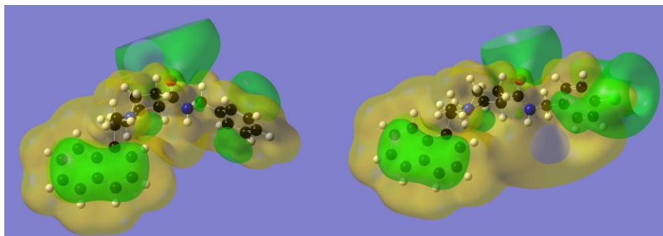
Figure 5. MEP of molecules 1 (left) and 13 (right). The green isovalue surface corresponds to negative MEP values (-0.01) and the yellow isovalue surface to positive MEP values (0.01).
