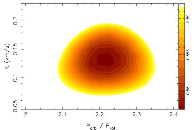
Figure 11. Variations of \chi^2 as a function of P_{\text{orb}}/P_{\text{rot}} and K , derived from the simultaneous modelling of the brightness features at the surface of V830 Tau and the orbital parameters of a close-in giant planet in circular orbit, following the new technique proposed by Petit et al. (2015). A clear minimum is obtained in the \chi^2 landscape, whose projection in a K versus P_{\text{orb}}/P_{\text{rot}} plane passing through the minimum is shown here, with the outer colour contour delimiting the 3\sigma (or 99.73 per cent) confidence region. This result suggests that a \simeq 1.4 M_{\text{Jup}} planet may be orbiting around V830 Tau. This figure is best viewed in colour.
