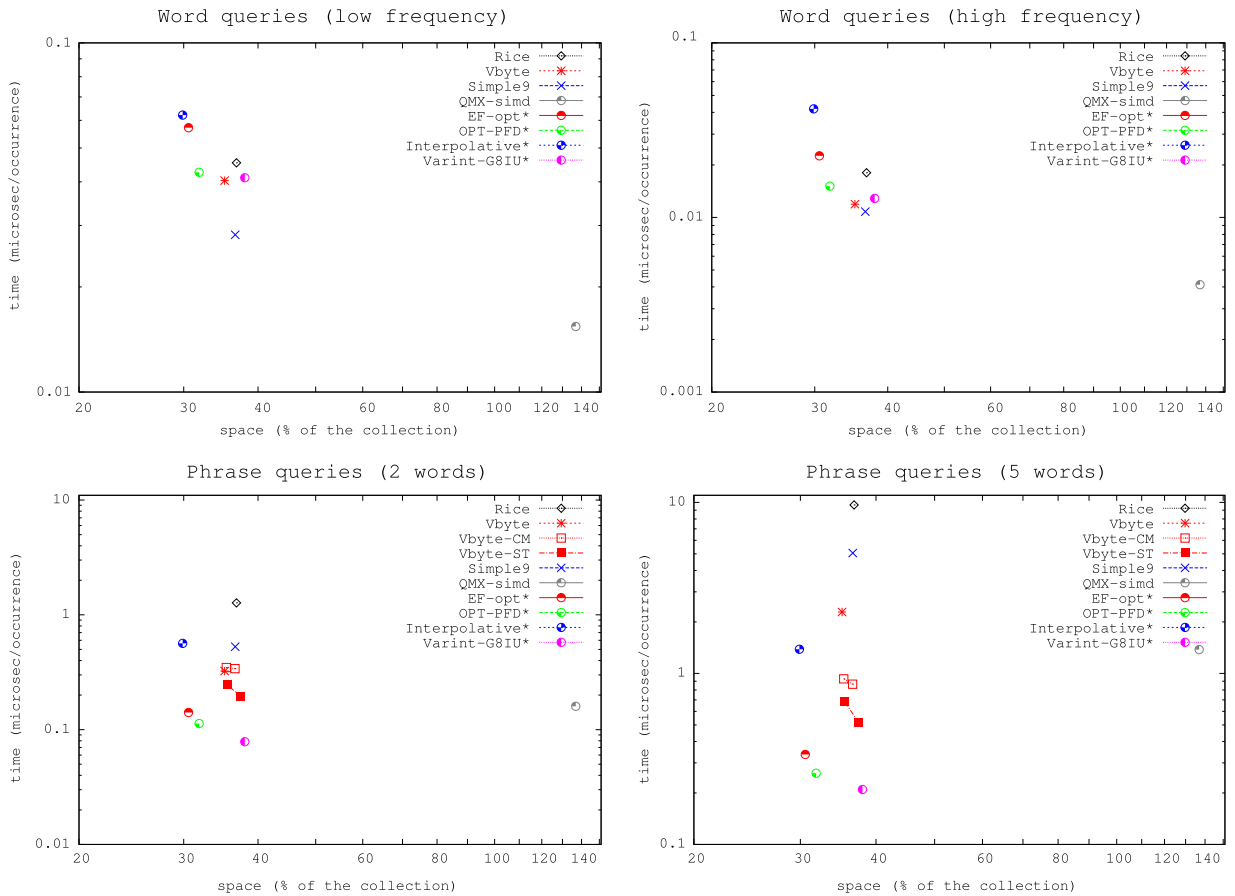
Fig. 6. Space/time tradeoffs for traditional representations of positional indexes. Logscale.
