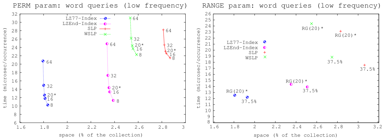
Fig. 7. Space/time tradeoffs for fine tuning on perm (left plot) and range (right plot) parameters.
