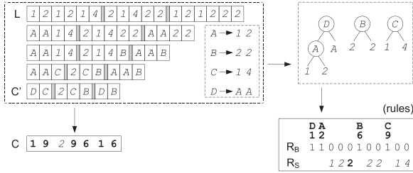
Fig. 1. Example of Re-Pair compression. Solid boxes ( C and rules ) enclose the data represented. Bold numbers (nonterminals) in the final C sequence and R_S refer to positions in R_B , whereas slanted ones (terminals) refer to original values. To distinguish them, the maximum offset u is added to the bold numbers.
