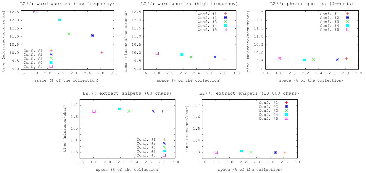
Fig. 8. Space/time tradeoffs for different LZ77-index configurations.
