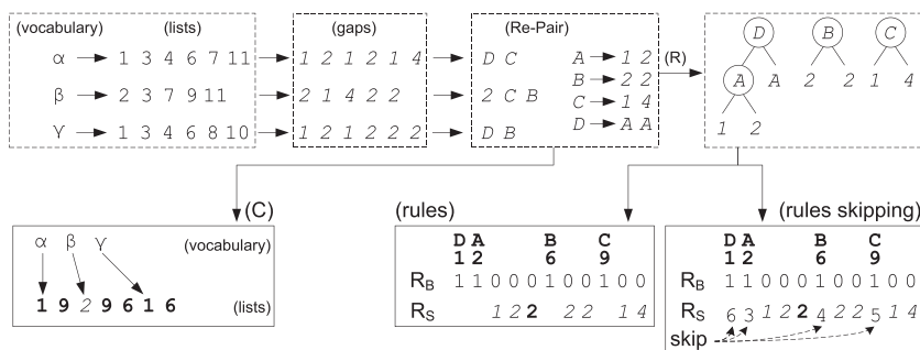
Fig. 2. Example of inverted lists compressed with our Re-Pair-based method. Solid boxes enclose the data we finally keep. We include both variants of compressed rules with data aligned to the 1s in R_B (skipping) or not. Again, bold numbers (nonterminals) in the lists and R_S refer to positions in R_B , whereas slanted ones (terminals) refer to gap values.
