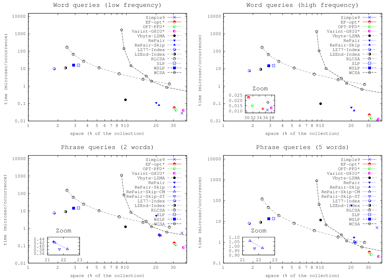
Fig. 9. Space/time tradeoffs for positional indexes. Logscale.
