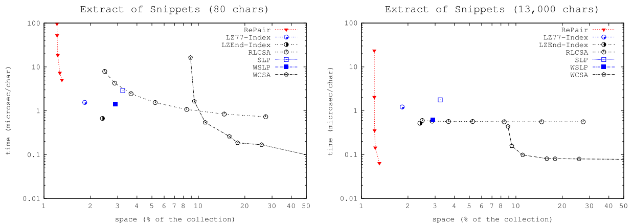
Fig. 10. Space/time tradeoffs for extraction. Logscale.
