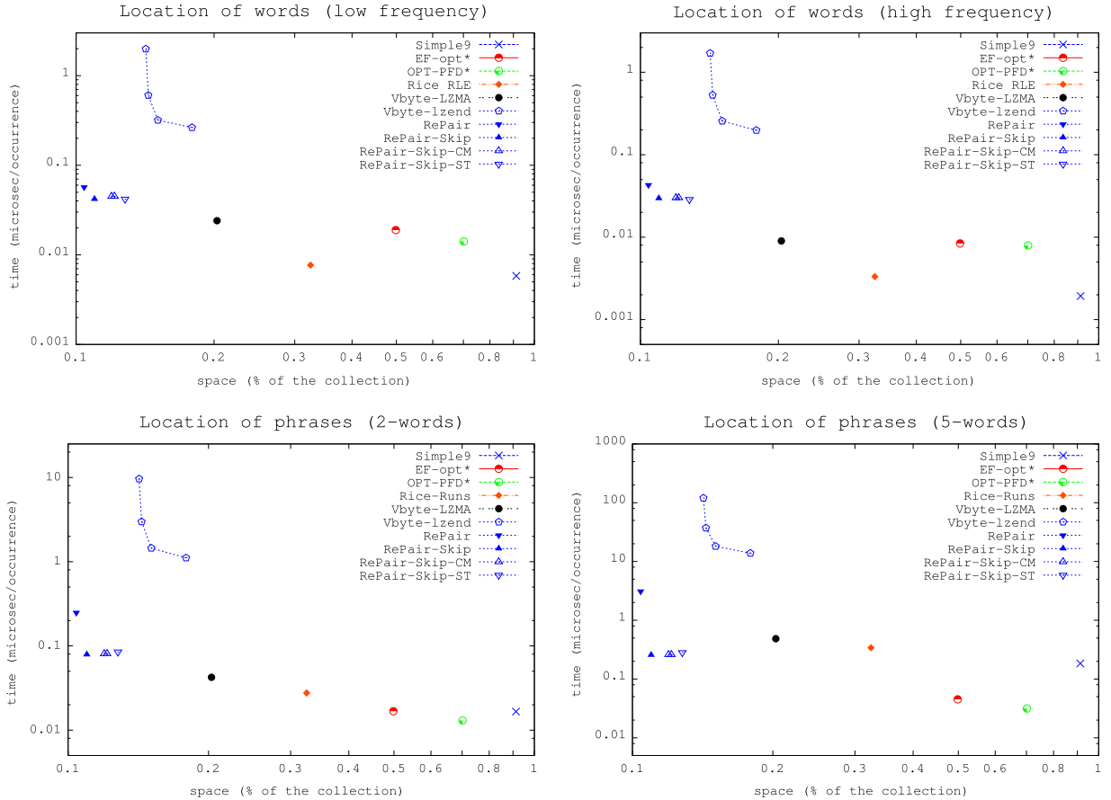
Fig. 4. Space/time tradeoffs for non-positional indexes, comparing the best classical techniques with our new ones. Logscale.
