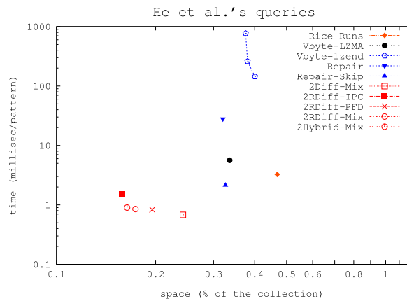
Fig. 5. Space/time tradeoffs for our best non-positional indexes and those of He et al. Logscale.
