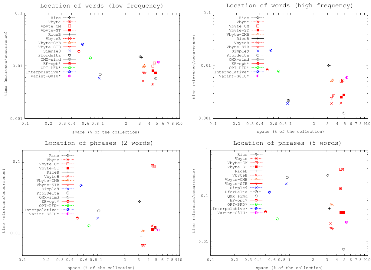
Fig. 3. Space/time tradeoffs for non-positional indexes using traditional techniques. Logscale.
