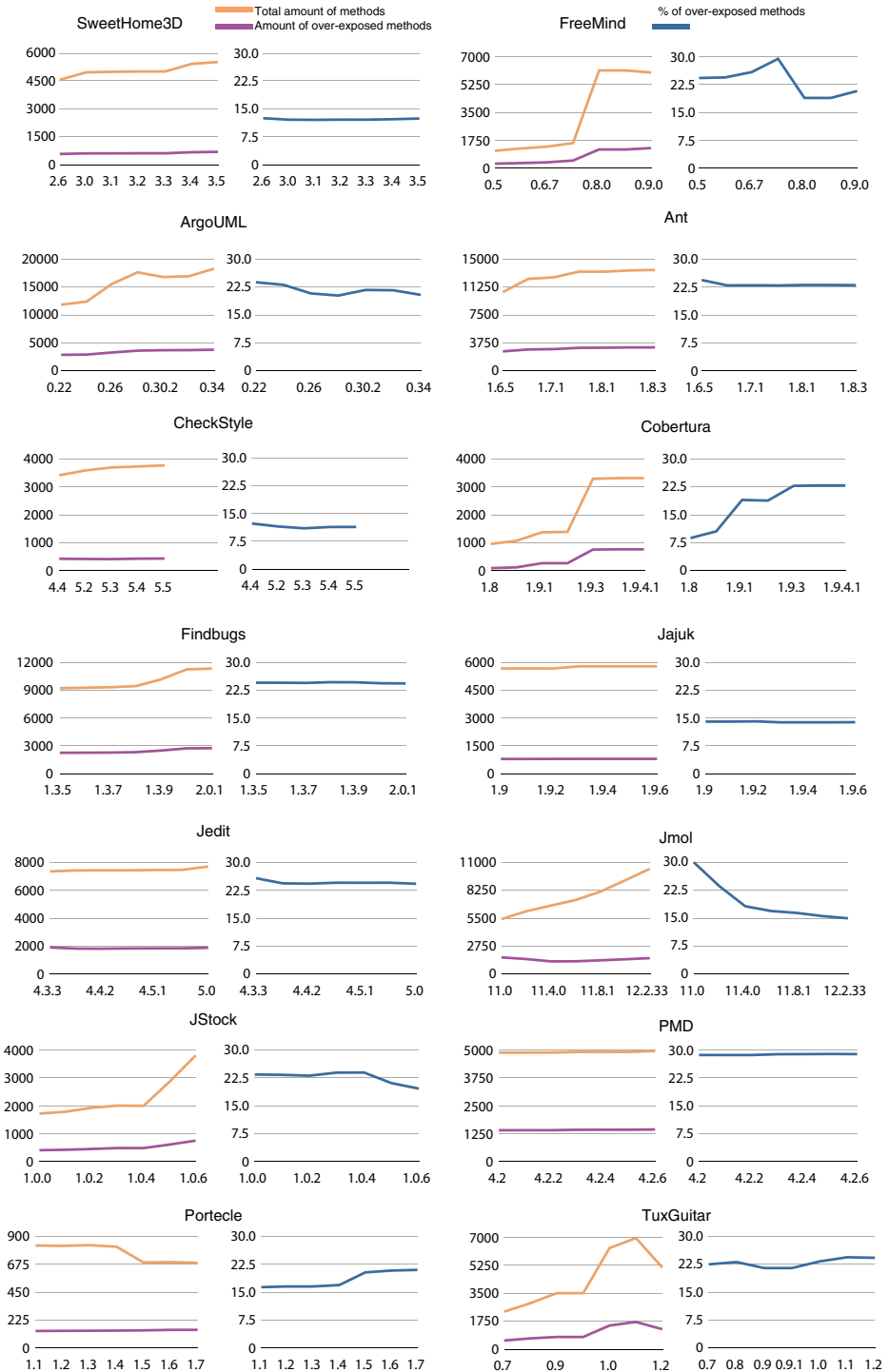
Fig. 7 Evolution of over-exposed methods
