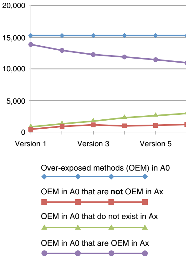
Fig. 4 Cumulative evolution of over-exposed methods
