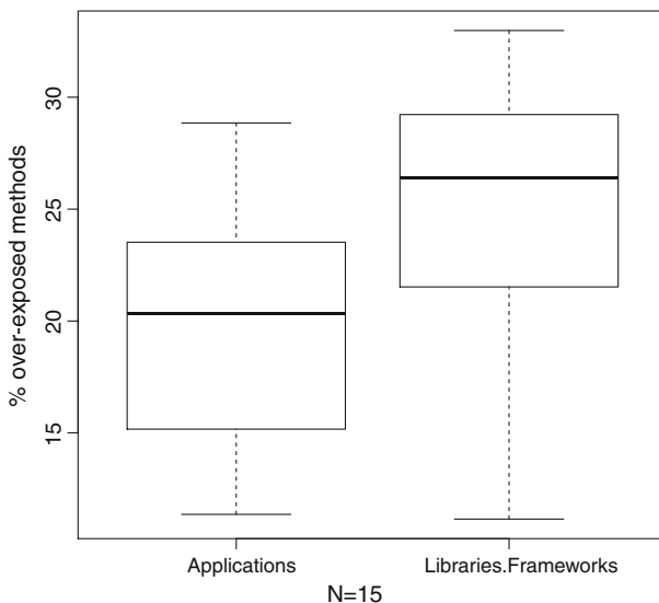
Fig. 3 Distribution of over-exposed methods in plain applications and libraries/frameworks
