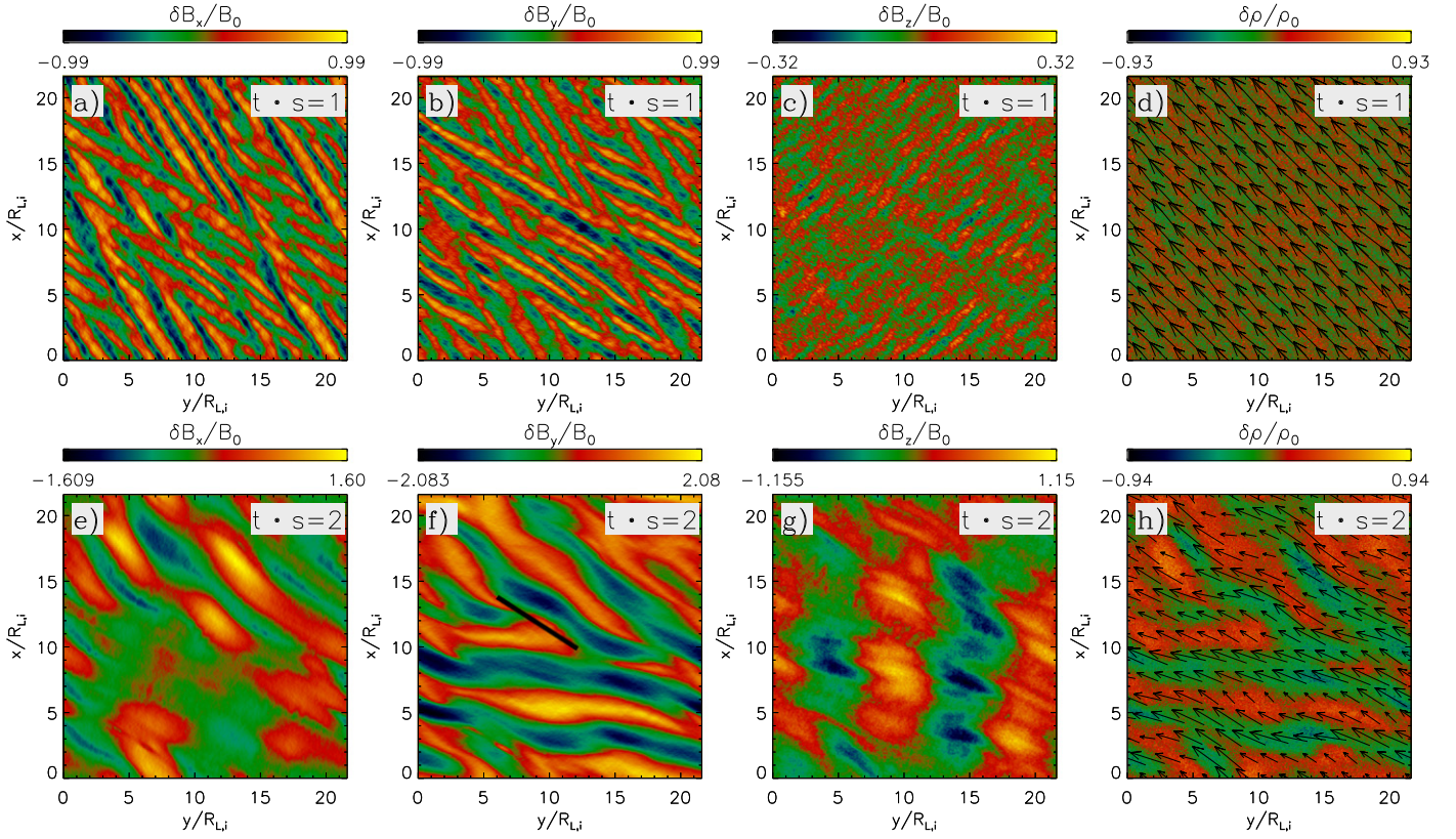
Figure 4. The three components of \delta B and plasma density fluctuations \delta \rho at two different times: t \cdot s = 1 (upper row) and t \cdot s = 2 (lower row), for run MW3 with m_i/m_e = 128 . Fields and density are normalized by B_0 and the initial density \rho_0 , respectively. Arrows in panels (d) and (h) show the mean magnetic field direction on the simulation x - y plane. At both times, the magnetic fluctuations are dominated by oblique mirror modes, especially \delta B_x and \delta B_y . Parallel propagating lower-amplitude IC modes are also apparent, particularly in \delta B_z , but are subdominant relative to the mirror modes. Significantly shorter wavelength parallel propagating whistler modes are also present in \delta B_z ; these have wavelengths shorter than that of the IC modes by a factor of R_{L,i}/R_{L,e} \approx (m_i/m_e)^{1/2} = 11 . The short black line in panel (f) shows a small region where the whistler modes are apparent. The corresponding fluctuations are shown in Figure 5(b).
