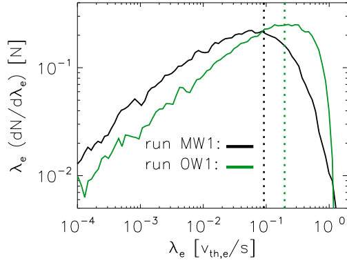
Figure 11. The distribution of electron mean free paths, \lambda_e(dN/d\lambda_e) , for electrons in runs OW1 (only whistlers; green line) and MW1 (whistlers and mirrors; black line), normalized by the total number of particles ( N ; (dN/d\lambda_e)d\lambda_e is the number of particles with mean free path between \lambda_e and \lambda_e + d\lambda_e ). \lambda_e for each particle is calculated measuring the distance d traveled by each electron along \mathbf{B} during an interval \Delta t = s^{-1} , from t \cdot s = 1.5 to 2.5 , and assuming d^2 = \lambda_e v_{th,e} \Delta t . The vertical-dotted green and black lines mark the average \langle \lambda_e \rangle for the OW1 and MW1 runs, respectively.
