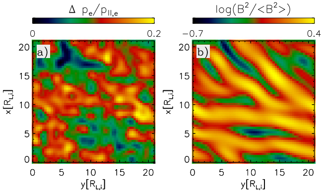
Figure 7. Comparison of the spatial distributions of \Delta p_e/p_{\parallel e} (panel (a)) and B^2 (panel (b)) for run MW3 at t \cdot s = 2 (same run and time shown in the lower row of Figure 4).
