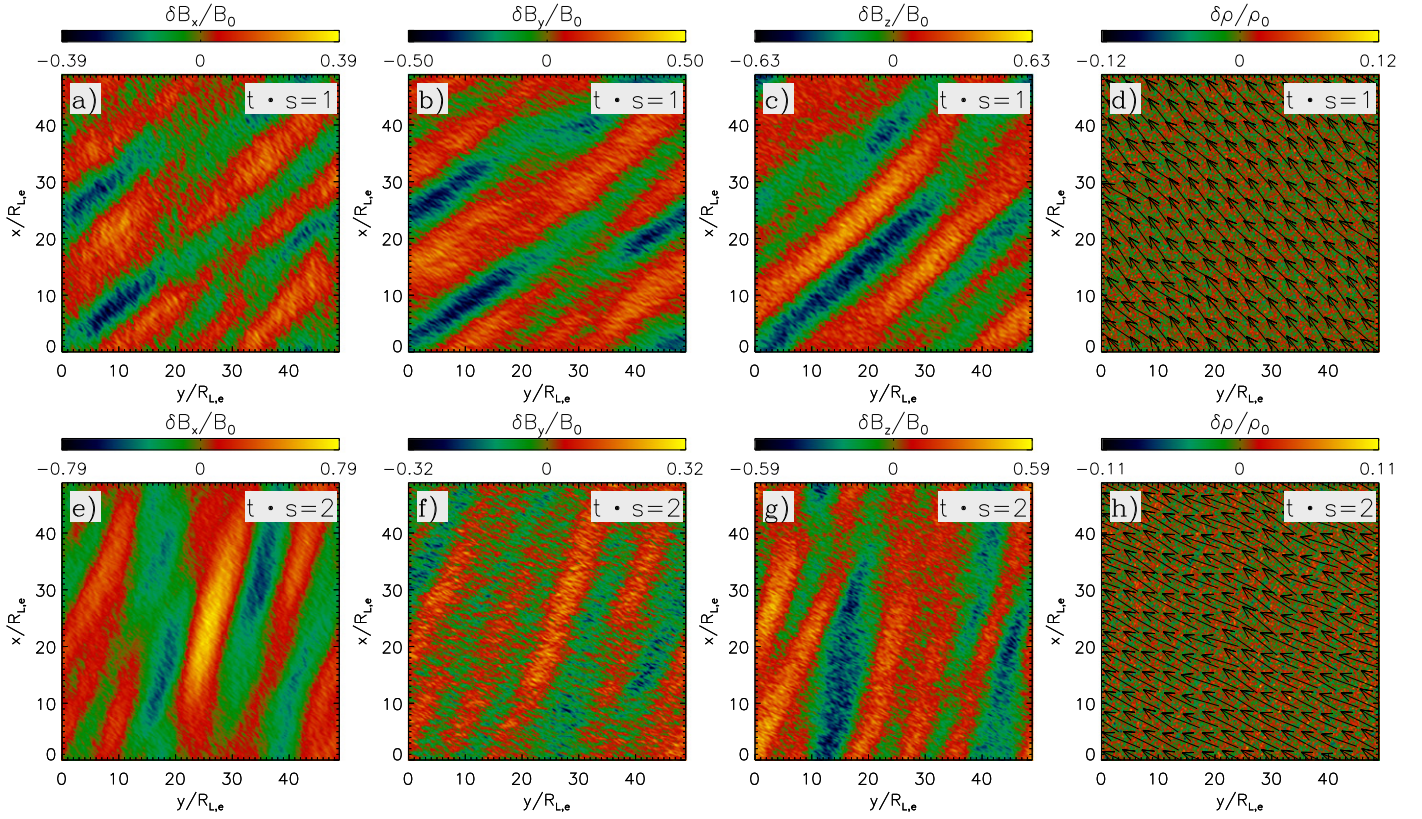
Figure 1. The three components of \delta\mathbf{B} and plasma density fluctuations \delta\rho at two different times: t \cdot s = 1 (upper row) and t \cdot s = 2 (lower row), for a simulation with only whistlers modes (run OW1 with m_i/m_e = \infty , so that the ions only provide a neutralizing charge). Fields and density are normalized by the initial magnetic field and density, B_0 and \rho_0 , respectively. Arrows in panels (d) and (h) show the mean magnetic field direction on the x - y simulation plane. For this m_i/m_e = \infty case, the magnetic fluctuations are dominated by nearly parallel whistler modes.
