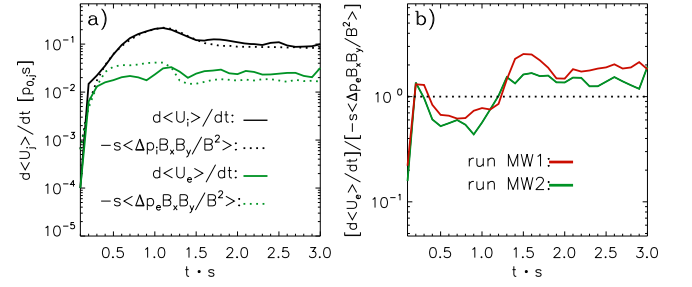
Figure 8. Panel (a): the ion and electron heating rates for run MW2, calculated directly via d\langle U_i \rangle/dt and d\langle U_e \rangle/dt (solid black and green, respectively), where U_j is the internal energy per unit volume of species j . For comparison, we also show that the numerically calculated heating rates are well explained by the theoretically predicted ion (dotted-black) and electron (dotted-green) energy gain via “anisotropic viscosity” tapping into the background velocity shear (see Equation (2)). Panel (b): the ratio between the electron heating, d\langle U_e \rangle/dt , and the expectation from viscous heating for runs MW1 (red) and MW2 (green), which only differ in their N_{\text{ppc}} ( =20 and 60 , respectively).
