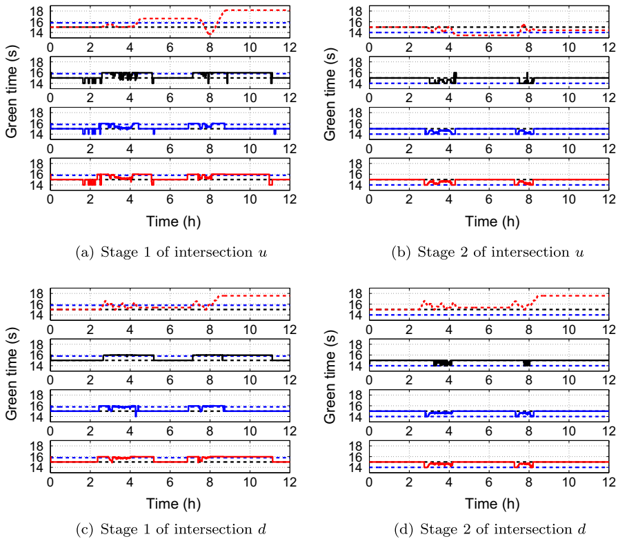
Fig. 16. Control actions stage 1 and stage 2, for the intersections u and d .
