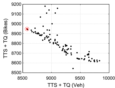
Fig. 11. MPC Case 2: Trade-off between vehicles and bicycles for different values of \alpha .
