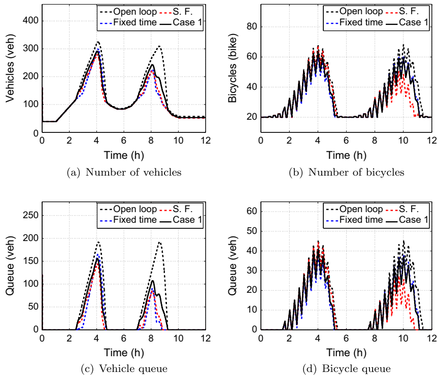
Fig. 10. Number of bicycles and vehicles for open loop, fixed time, state feedback (S.F.) and MPC Case 1 controllers. (a) Number of vehicles, (b) number of bicycles, (c) queue of vehicles, and (d) queue of bicycles.
