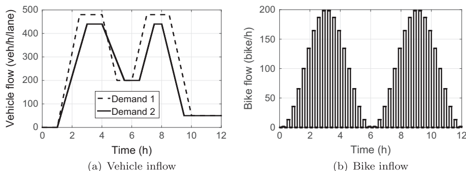
Fig. 4. Inlet flow profile to the intersections.
