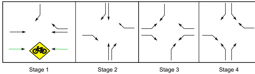
Fig. 5. Stages of the traffic lights.
