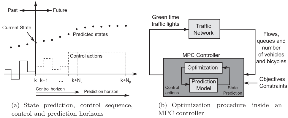
Fig. 3. Procedures carried out inside an MPC controller.
