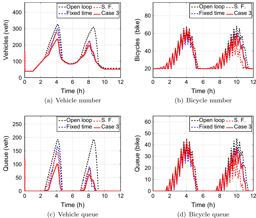
Fig. 14. Number of bicycles and vehicles for open loop, fixed time, state feedback (S.F.) and MPC Case 3 controllers. (a) Number of vehicles, (b) number of bicycles, (c) queue of vehicles, (d) queue of bicycles.
