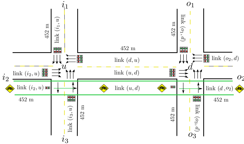
Fig. 2. Two interconnected intersections in an urban traffic network.
