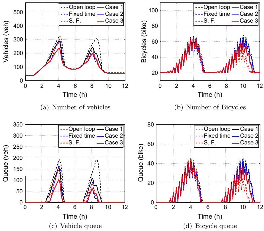
Fig. 15. Number of bicycles and vehicles.
