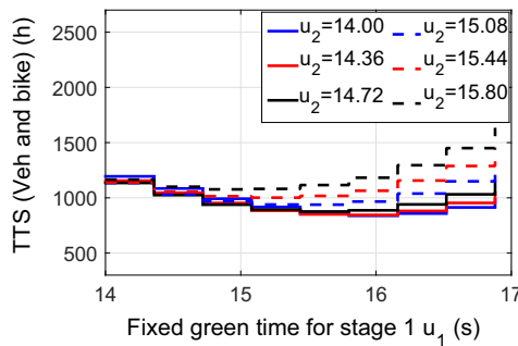
Fig. 7. TTS as function of a fixed green time of the stage 1 u_1 and 6 cases for the stage 2 u_2 .
