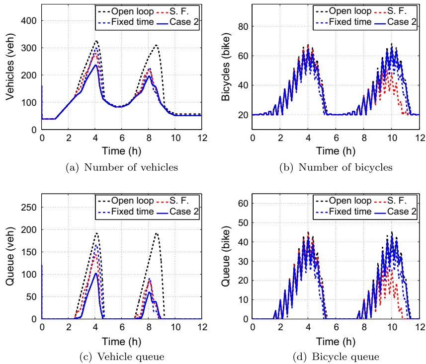
Fig. 12. Number of bicycles and vehicles for open loop, fixed time, state feedback (S.F.) and MPC Case 2 controllers. (a) Number of vehicles, (b) number of bicycles, (c) queue of vehicles, and (d) queue of bicycles.
