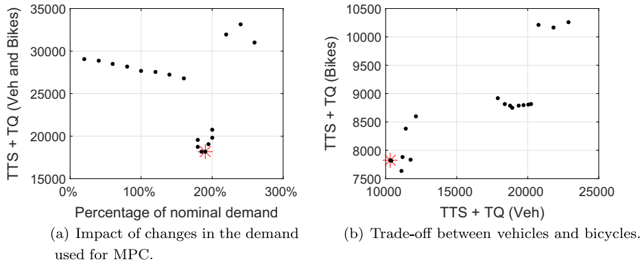
Fig. 8. Sensitivity of controller performance against changes in the demand value – MPC Case 1.
