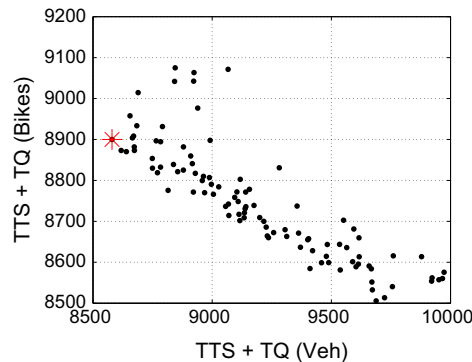
Fig. 13. MPC Case 3: Trade-off between vehicles and bicycles for different values of \alpha .
