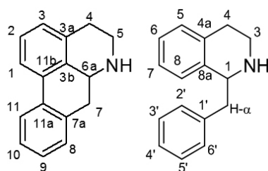
Figure 1. Numbering used for aporphines (left) and tetrahydroisoquinolines (right).
