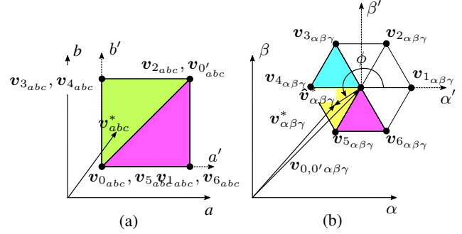
Fig. 4. Top view of (a) Fig. 3a and (b) Fig. 3b in a non-displaced origin.
