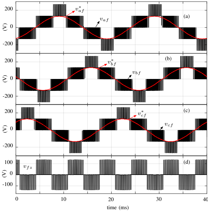
Fig. 7. Output voltages (a) v_{af} , (b) v_{bf} , (c) v_{cf} for a four-leg NPC converter with their respective references v_{af}^* , v_{bf}^* and v_{cf}^* in red. In (d) the modulated voltage of the fourth leg v_{fz} . Sampling frequency f_s=6kHz , dc-link voltage 270 V.
