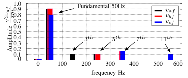
Fig. 10. FFT for the phase-to-neutral voltages v_{af} , v_{bf} and v_{cf} of Fig. 7. The amplitude has been normalized by \frac{270}{\sqrt{3}} .
