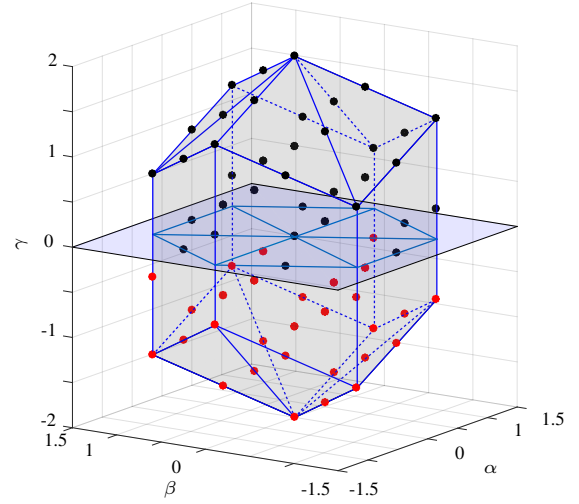
Fig. 2. Representation of the 65 different vectors in the \alpha\beta\gamma space for a four-leg NPC converter. The external surface is also shown. Black dots are on or over the \alpha\beta plane.
