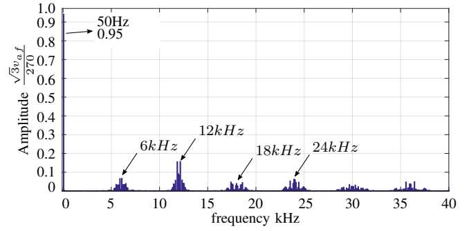
Fig. 8. FFT for v_{af} of Fig. 7. The amplitude has been normalized by \frac{270}{\sqrt{3}} .
