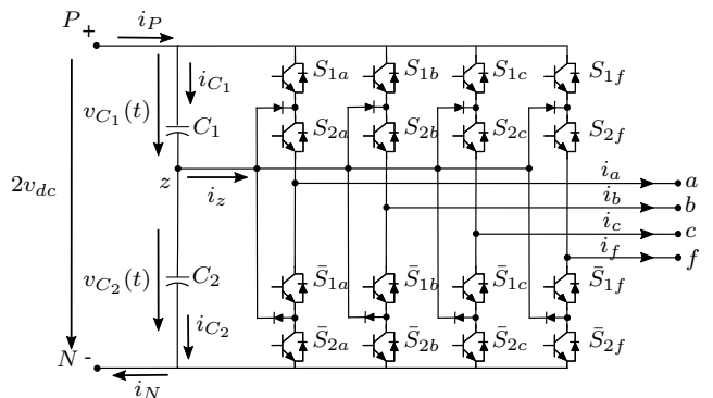
Fig. 1. Electrical diagram for a four-leg Neutral-Point-Clamped Inverter
