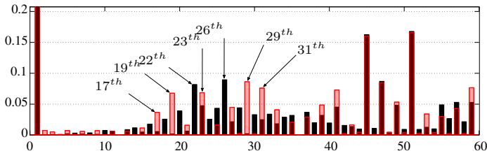
Fig. 12. FFT for the phase voltage V_{af} with and without even-harmonic elimination of Fig. 11.
