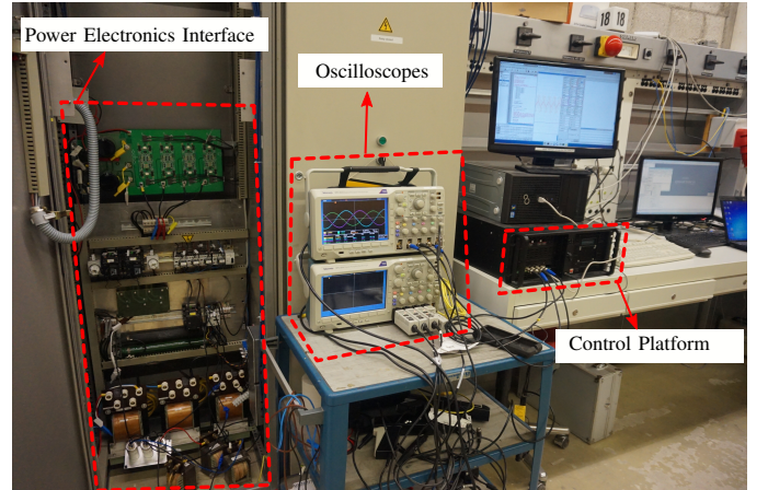
Fig. 6. Complete view of a 6kW experimental rig for a four-leg NPC converter.
