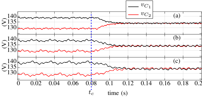
Fig. 13. Control impact over the dc-link voltages v_{C1} and v_{C2} under non-sinusoidal modulated voltages for (a) balanced three-phase load R=30\Omega , L=22mH and a three-phase rectifier with load R_{rec}=60 (in parallel)(b) RL load of phase c has been disconnected, (c) RL load of phase b and c has been disconnected.
