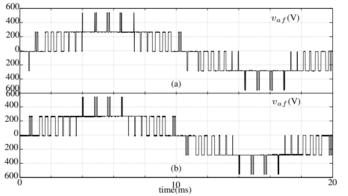
Fig. 11. Experimental assessment of the proposed SVM algorithm for a four-leg NPC (a) V_{af} without even-harmonic eliminations and (b) V_{af} with even-harmonic elimination. The implemented parameters are f_s = 1200Hz , V_{dc} = 545V .
