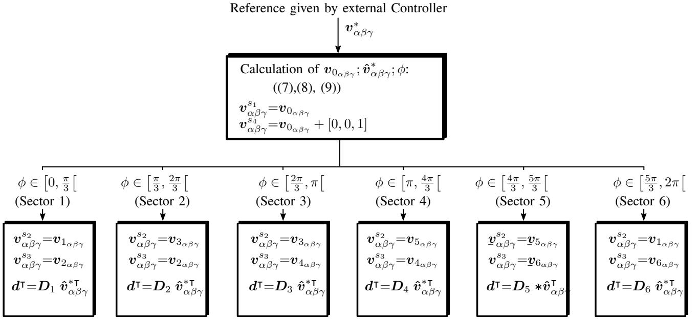
Fig. 5. General diagram for a three-dimensional SVM. d^T denotes the transpose of the vector d = [d_2, d_3, d_4] . The dwell time d_1 is obtained as d_1 = 1 - d_2 - d_3 - d_4; \forall \phi .
