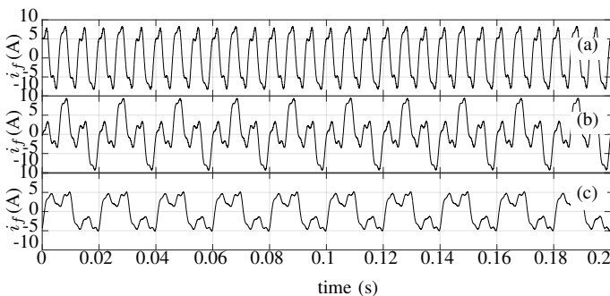
Fig. 14. Neutral current i_f under non-sinusoidal modulated voltages for (a) balanced three-phase load R=30\Omega , L=22mH and a three-phase rectifier with load R_{rec}=60 (connected in parallel) (b) RL load of phase c has been disconnected, (c) RL load of phase b and c has been disconnected.
