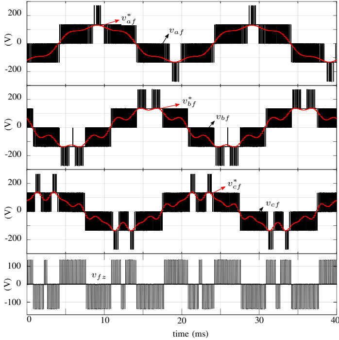
Fig. 9. Output voltages (a) v_{af} , (b) v_{bf} and (c) v_{cf} for a four-leg NPC converter with their respective references v_{af}^* , v_{bf}^* and v_{cf}^* in red for unbalanced and non-sinusoidal references. In (d) the modulated voltage of the fourth leg v_{fz} . Sampling frequency f_s=6kHz , dc-link voltage 270 V.
