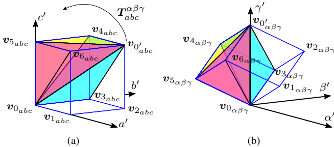
Fig. 3. Three-dimensional representation of the eight transitioning vectors that form the cube in the (a) abc and (b) \alpha\beta\gamma space respectively. The coordinate frames have been displaced to v_{0_{abc}} (or equivalently to v_{0_{\alpha\beta\gamma}} ), and are denoted as a'b'c' and \alpha'\beta'\gamma' respectively.
