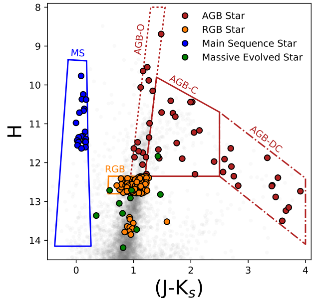
FIG. 4.— CMD of targets and target classes in a sample LMC field ( LMC-9 ). Red points indicate AGB stars, comprising AGB-O, AGB-C, and dusty AGB-C (AGB-DC) stars appearing in three different color-magnitude bins. Orange indicates RGB stars, which include both stars selected from the orange box and those with existing literature data. Blue are hot main sequence stars, selected from the drawn box, and green are other massive evolved stars selected from the literature. Gray points are other 2MASS sources in the field that were not targeted as LMC stars.
