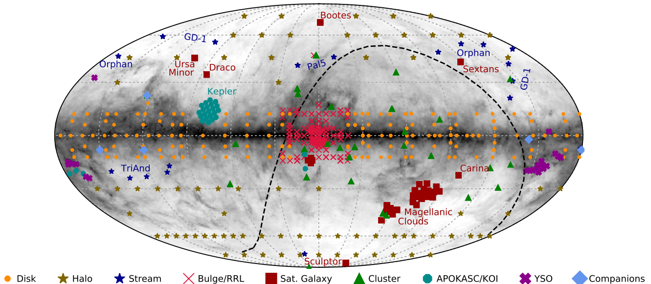
FIG. 1.— The current APOGEE-2 field plan in Galactic coordinates, with fields colored by the primary driver of their placement. The background grayscale is the integrated E(B - V) map from Schlegel et al. (1998); the concentration of APOGEE-2 observations in some of the dustiest parts of the Milky Way highlights the targeting advantage of NIR surveys compared to optical ones. The dashed line indicates the approximate declination limit of -10^\circ adopted for the Northern (upper, left) and Southern (lower, right) survey components; fields with declinations within \sim 15^\circ of this line may be observed from either hemisphere. The gray meridians and parallels are spaced every \Delta l, \Delta b = 30^\circ .
