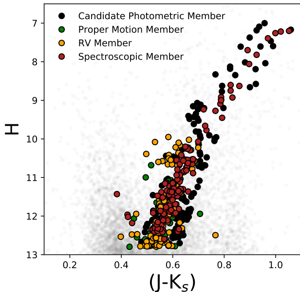
FIG. 3.— CMD of targets in the globular cluster NGC 6752 and their priority classes, from stars with 2MASS colors consistent with the cluster locus (lowest priority, black circles), through known members with previous spectroscopic information (highest priority, red circles). The faint gray points in the background are the rest of the 2MASS sources in the field that were not targeted as part of the cluster selection.
