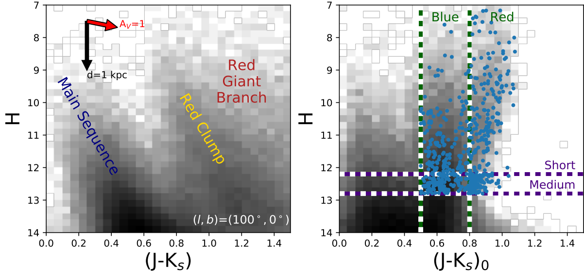
FIG. 2.— RJCE dereddening and target selection in the 6-visit disk field 100+00 . The left panel shows the observed (J - K_s, H) CMD, with the primary populations labeled. The right panel contains the same stars in the dereddened ([J - K_s]_0, H) CMD, overplotted with this field’s targets (blue points). As described in §4.1, targets are drawn from multiple bins in H magnitude and dereddened (J - K_s)_0 color.
