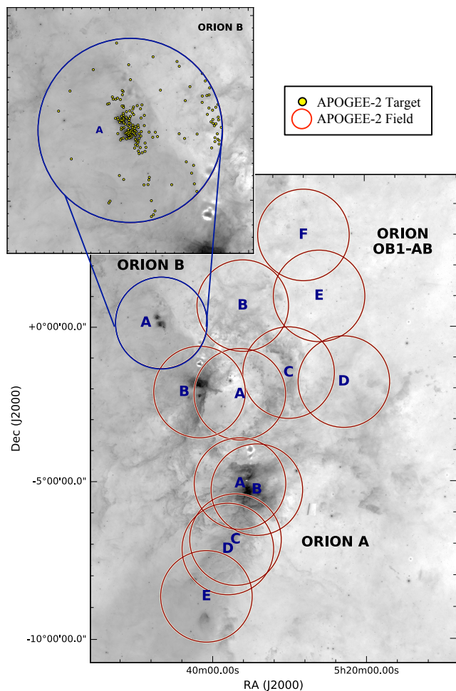
FIG. 6.— Example of targeting in embedded young clusters, here for the extended Orion fields: Orion A, Orion B, and Orion OB1-AB. The background grayscale is WISE 12\mu\text{m} emission, and the red circles indicate the location of APOGEE-2 fields. The letters in each field identify the field name — e.g., ORIONB-A and ORIONA-E . The inset shows targets in the ORIONB-A field.
