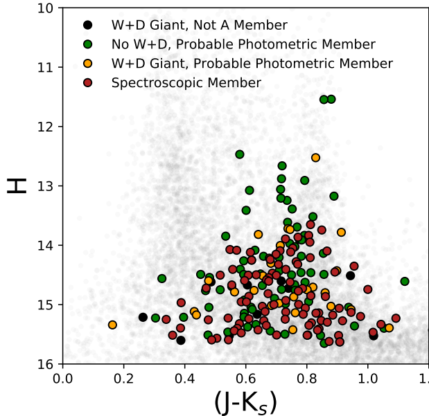
FIG. 5.— CMD of targets in the Ursa Minor dwarf galaxy and their priority classes, from W+D giants with broadband colors inconsistent with galaxy membership (lowest priority, black circles), through known members with previous spectroscopic information (highest priority, red circles). The faint gray points in the background are the rest of the 2MASS sources in the field that were not targeted as part of the dSph selection.
