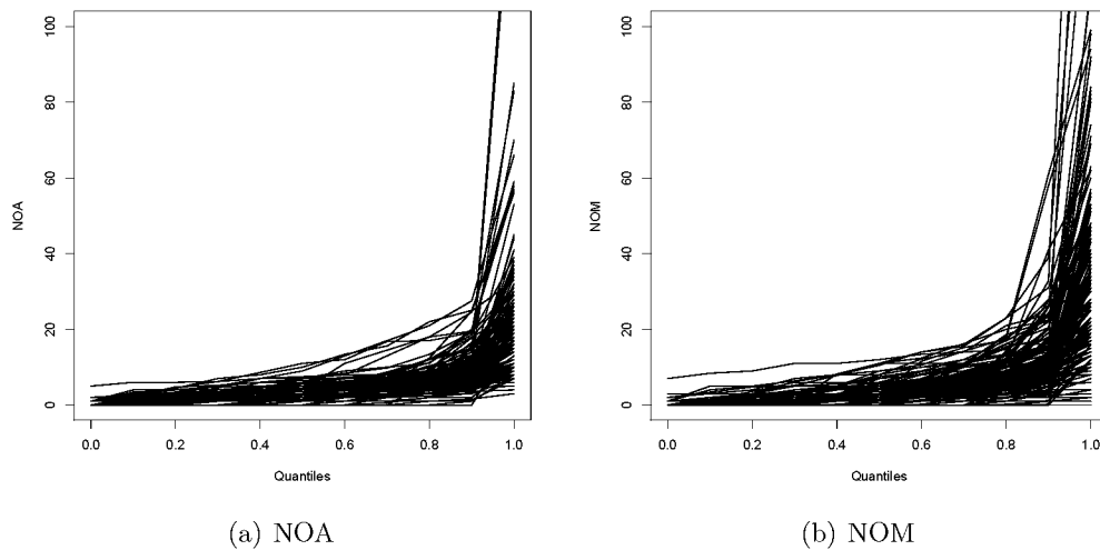
Figure 11: Quantile functions
