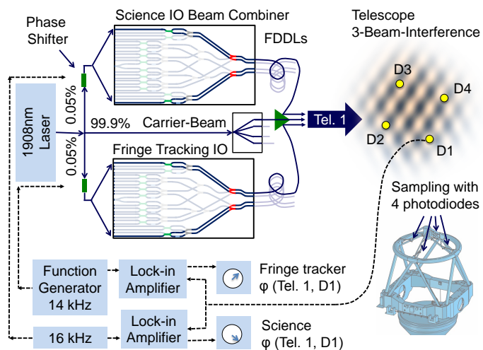
Fig. 9. Laser metrology: the schematic shows the working principle of measuring the optical path difference between the two beam combiners and the telescope. The metrology laser is launched from the spectrometers and is detected above the primary mirror at the telescope secondary mirror spider arms. To minimize the laser power in the spectrometer and optical fibers, we do not directly measure the interference between the laser coming from the two beam combiners, but measure separately for the fringe tracker and science beam combiner the phase relative to a very bright, third “carrier” beam. The actual phase measurement is implemented by modulating the phase of the fringe tracker and science metrology at different frequencies, and measuring the cosine and sine components of the respective interference with the third beam through lock-in amplifiers.
