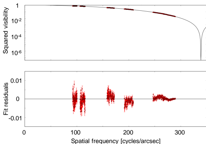
Fig. 15. Limb darkening in the K5 III giant \xi Tel: The top panel shows the observed squared visibility for \xi Tel. The solid line is the best fit limb darkening disc model. The fit residuals (bottom) are typically smaller than 0.005, corresponding to a visibility accuracy of better than 0.25 %.
