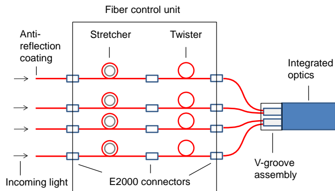
Fig. 4. Single-mode fibers and fiber control unit: the schematic shows the various fiber subsections and functions. The entrance of the fibers are anti-reflection coated. The optical path length is adjusted by piezo driven fiber coils. The direction of linear polarization is aligned by motorized fiber twisters. The fibers of these subsections are connected through optimized E2000 connectors. The integrated optics beam combiner - operated at 200K - is connected through a dedicated V-groove assembly.
