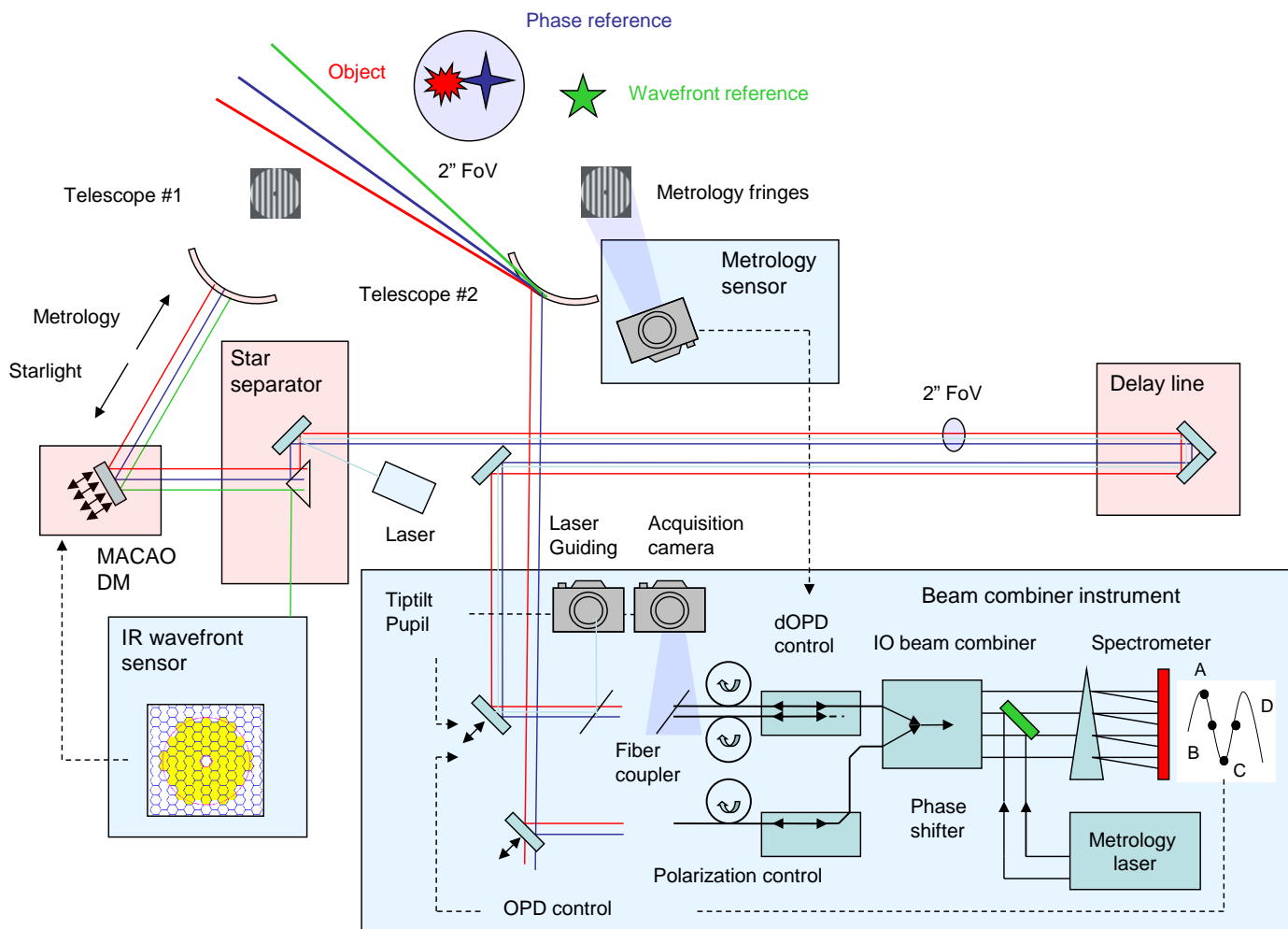
Fig. 1. Overview and working principle of GRAVITY: the instrument coherently combines the light of the four 8m UTs of the VLTI or the four 1.8m ATs. It provides infrared wavefront sensing to control the telescope adaptive optics, two interferometric beam combiners - one for fringe-tracking and one for the science object -, an acquisition camera and various laser guiding systems for beam stabilization, and a dedicated laser metrology to trace the optical path length differences for narrow angle astrometry. The overview illustrates the light path and location of the various subsystems. For clarity, we show only two telescopes, one beam combiner and one wavefront sensor. The wavefront sensor star (green) can be outside the VLTI field of view. Depending on the brightness of the science object (red), the fringe tracker is either fed by a beam splitter, or - as illustrated in this figure - by a bright off-axis phase reference star (blue). The GRAVITY subsystems (light blue boxes) are embedded and take advantage of the already existing VLTI infrastructure (light red boxes).
