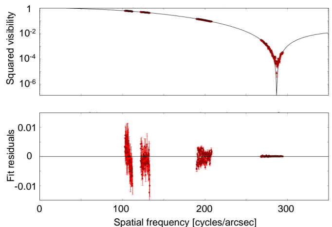
Fig. 16. Depth of the first null of the K5/M0 III giant 24 Cap: the top panel shows the observed squared visibility for 24 Cap. The depth of the null of the first minimum is 8 \times 10^{-6} , corresponding to a visibility modulus of 0.3 %. The non-zero visibility is likely caused by the granulation in the star's surface. The solid line is the best fit limb darkening disc model, the fit results are shown in the lower panel.
