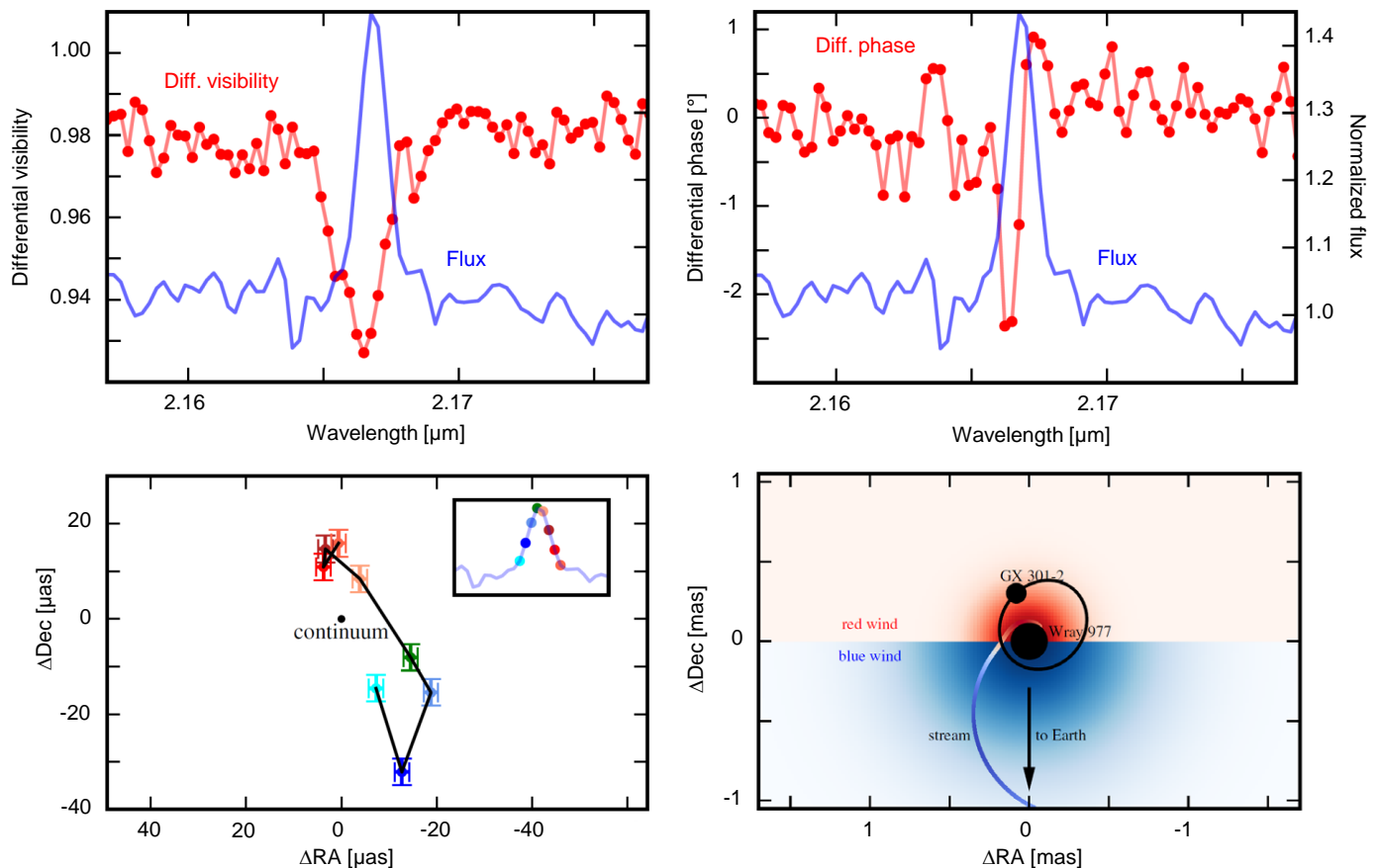
Fig. 19. Tracing the inner region of the HMXB BP Cru: the top figures display the differential visibility amplitudes (left) and phases (right) across the Bry line (red) and the continuum normalized spectrum (blue) exemplary for one of the six observed baselines. The lower left panel shows the model-independent centroid positions for each wavelength across the Bry line. The image on the blue side of the line has a larger centroid shift than the image on the red side. Note the \mu\text{as} scale on the lower left panel. The schematic on the lower right panel shows the BP Cru system as inferred from simple geometric model fits to the interferometric signatures. The donor star, the X-ray pulsar and its binary orbit are shown in black. An extended wind could explain the visibility amplitude drops across the emission line. A size asymmetry between the blue and red shifted sides of the wind could be related to the X-ray illumination by the compact object. Non-zero visibility phases, also asymmetric between blue and red wavelengths, could be explained by the presence of a gas stream. A simple stream model following Leahy & Kostka (2008) is shown in the bottom right, with the colors along the stream corresponding to the radial velocity measured at Earth ( i = 60^\circ ).
