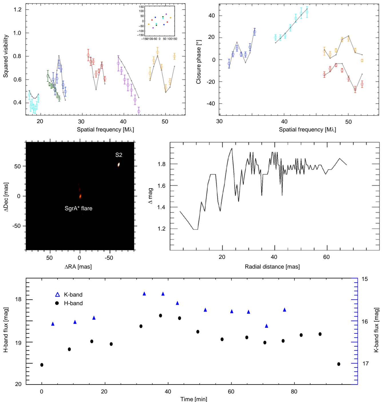
Fig. 22. First detection of Sgr A* in infrared interferometry: the top panels show the observed squared visibilities and closure phases for a 5 minute exposure centered on Sgr A* during a flare with a peak brightness of about m_K \approx 15 mag. The prominent modulation in the two quantities results from the two brightest objects in the field, the flaring Sgr A* and the star S2. The black line is the best fit “binary” model. The middle left panel displays the reconstructed image from the combination of three exposures around the peak of the flare. The middle right panel plots the 3\sigma detection limits for a third source in the full data set, for which the average flare brightness was m_K \approx 15.5 mag. We can exclude a third source brighter than m_K = 17.1 mag for 90 % of the area. The lower panel shows the H-band (black) and K-band (blue) lightcurve of Sgr A* during the flare, as measured from the acquisition camera images and derived from the best fit to the interferometric visibilities and closure phases, respectively.
