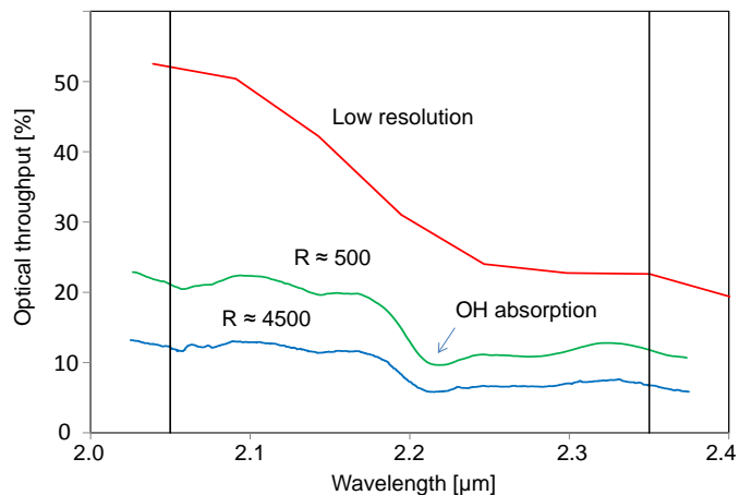
Fig. 7. Optical throughput of the beam combiner instrument – excluding telescopes, VLTI beam relay, and detector quantum efficiency: low (red), R \approx 500 (green) and R \approx 4500 (blue) spectral resolution. The fringe tracker throughput is comparable to the science spectrometer at low resolution. The lower throughput of the R \approx 500 and R \approx 4500 spectral resolution is dominated by losses from the gratings.
