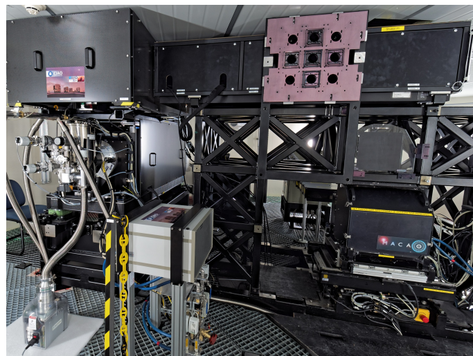
Fig. 11. Coudé Infrared Adaptive Optics: the photograph shows the Coudé room of UT4 in June 2016. The big central structure is the star separator. The CIAO wavefront sensor comprises the tower structure on the left side, with the cryostat connected to a pump on the floor, and the readout electronics located next to it (light gray box connected to blue cooling pipes). The visual wavefront sensor MACAO is located at the lower right.
