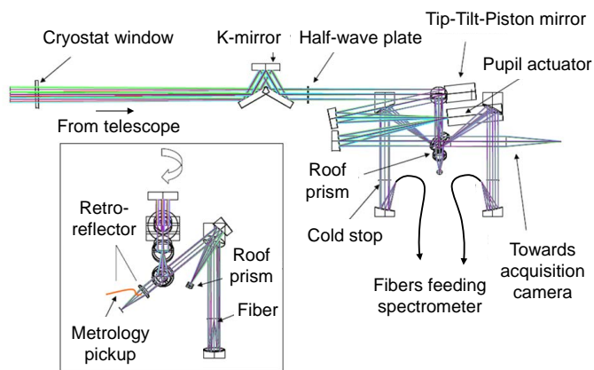
Fig. 3. Fiber coupler: the schematic shows the side and front views of the optical design for one of the four fiber couplers. The fiber couplers provide all optics and actuators to rotate and stabilize the beam, to split the light of the fringe tracker and science objects, and to optimally couple the light into the single-mode fibers. In addition, the fiber coupler contains several supplementary functions, including a metrology pickup to servo the fiber differential delay lines, a retro-reflector to image the fiber input on the acquisition camera, and motorized half-wave plates for co-aligning the polarization.
