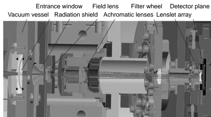
Fig. 12. CIAO cryostat: the 3D CAD drawing depicts the CIAO cryostat with its cold optics and actuators. The movable field lens, which is located behind the entrance window, controls the lateral pupil position (Dai et al. 2017) as seen by the lenslet array. The achromatic lenses image the deformable mirror (pupil) onto the lenslet array. The filter wheel houses an H+K-band filter, two neutral density filters, a closed position, and an open position.
