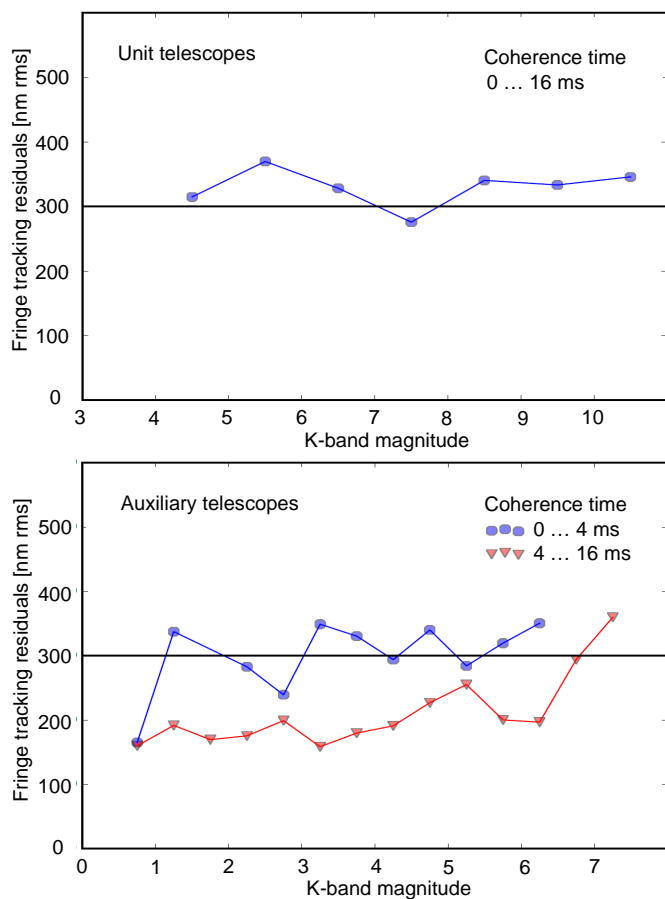
Fig. 10. Fringe-tracking performance: the figures show the fringe-tracking residuals as a function of the reference stars’s K-band correlated magnitude for UTs (top) and ATs (bottom), respectively. The horizontal lines indicate residuals of 300 nm rms, for which the fringe contrast in long exposures is reduced by \sim 30\% in the K-band. For the ATs, we plot the fringe-tracking residuals separately for good seeing with long atmospheric coherence times \tau_0 > 4 ms (red), and for short coherence times \tau_0 < 4 ms (blue). We do not have enough statistics to make this distinction for the UTs. The OPD residuals for long coherence times are typically 200 nm and 300 nm rms, the limiting magnitudes around m_K \approx 7 mag and m_K \approx 10 mag for the ATs and UTs, respectively.
