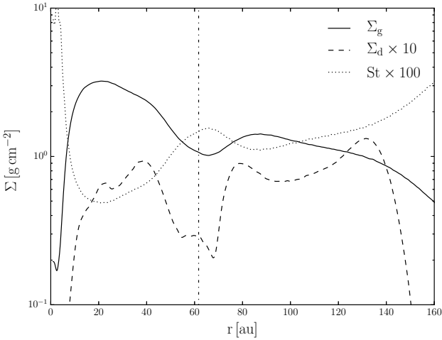
Figure 4. Azimuthally averaged dust (dashed) and gas (solid) surface density for our best disc hosting a planet with an initial mass of 0.15 M_{\text{J}} , initially located at 65 au from the central star. The dust surface density is scaled by a factor of 10 at the end of the simulation, for direct comparison with the gas phase. After 85 orbits (measured at 65 au), the planet is at 61.7 au from the central star and its mass is 0.7 M_{\text{J}} . The dotted line indicates the Stokes number multiplied by 100. The vertical line indicates the planet orbit.
