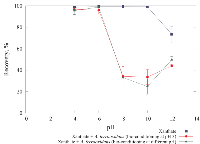
Fig. 3. Effect of A. ferrooxidans on pyrite recovery in saline water, 35 g/l NaCl. The concentration of A. ferrooxidans and xanthate in the conditioning was 3 \times 10^8 bacteria/ml and 4.74 \times 10^{-5} M, respectively.
