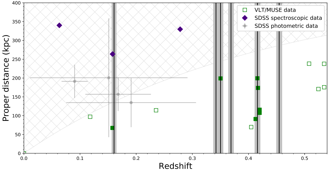
Figure 3. Distribution of impact parameter to the Q1410 sight-line as a function of redshift. Our VLT/MUSE sample of galaxies is shown in green squares. SDSS galaxies are shown in violet diamonds and gray circles (See Sect. 3.4 for details). We only show here galaxies in the SDSS photometric catalog that are outside the MUSE FoV. The vertical black lines surrounded by a shaded region mark the redshift of the inter-cluster axes \pm 1000 km s -1 from its rest frame. Filled squares mark sources in the VLT/MUSE sample that are located within \pm 1000 km s -1 of an inter-cluster axis and will be the subject of further analysis. The hatched area in the upper left corner is outside the MUSE FoV and shows the approximate edges of our spectroscopic survey.
