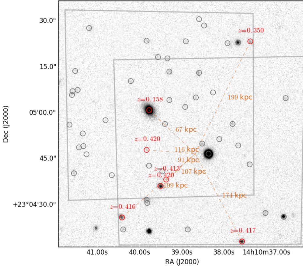
Figure 1. VLT/VIMOS image of our full MUSE field of view. The VLT/MUSE exposures are centered on the bright galaxy (upper left of the center) and the QSO Q1410 (lower right of the center) respectively (see Table 1). The gray contours mark the field of view of each individual VLT/MUSE exposure. We have characterized and measured redshifts for most sources brighter than r = 25 mag (see Table 2)). Red circles show galaxies at redshifts within \Delta v = \pm 1000 km s^{-1} of any BLA. Grey circles mark the rest of the sources characterized with a redshift.
