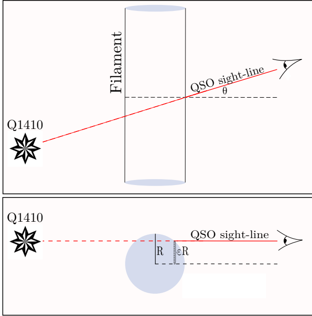
Figure 6. Schematic representation along the sight-line (in red) of the geometry assumed for deriving WHIM density. A filamentary structure is represented by a cylinder. \theta is the angle between the sight-line and the perpendicular axis to the filament. The impact parameter of the sight-line respect to the center is parametrized by the fraction \epsilon .
