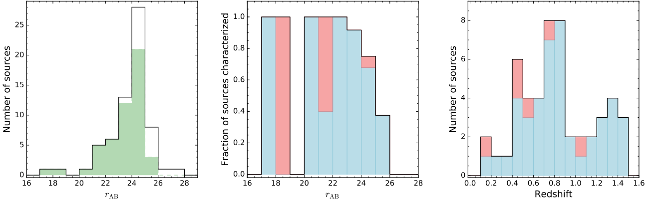
Figure 2. Left: Survey histogram colored in green for our sample with measured redshifts. The black line shows the distribution for the whole sample detected by SExtractor. Our detection threshold is at r \sim 25 mag. Center shows the completeness fraction of the redshift survey. The star forming galaxies are shown in blue and the non-star forming galaxies in red. The black contour marks our full sample. We reach to \sim 75\% successful characterization fraction at an apparent magnitude r_{AB} = 25 mag. Right: shows the redshift distribution of our full characterized sample colored by star forming and non-star forming fraction same as the central panel. The LAE candidate at z \approx 3.15 is not shown here.
