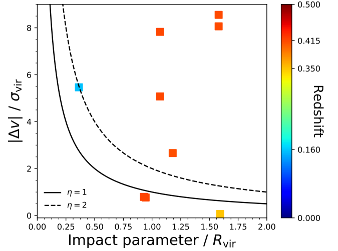
Figure 4. Each square represents a single galaxy-BLA combination identified from our sample, representing a total of 7 galaxies and 4 absorbers across three separate intra-cluster axes. The panel shows the relationship between potential host galaxies and absorbers in terms of a velocity difference and impact parameter to the QSO sight-line in units of \sigma_{\text{vir}} and R_{\text{vir}} respectively. The \eta is defined as \frac{R_{\text{projected}} |\Delta v|}{R_{\text{vir}} \sigma_{\text{vir}}} and is used to quantify the global environment. \eta < 2 should mark the limit for a gravitationally bounded system ( Shen et al. 2017 ).
