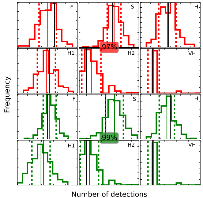
Figure 7. Distribution of detections within the simulations. The six upper panels, in red, refer to the six bands at the 97% reliability threshold. The six lower panels, in green, refer to six bands at the 99% reliability threshold. From top left to bottom right, the bands are F, S, H, H1, H2, and VH. In each panel, the dashed lines mark the \pm 1\sigma interval from the average, while the black solid line marks the position of the detections in the data mosaic, which are always within \pm 1\sigma from the mean of the simulations, shown by the solid red or green line. Numerical values for the average number of detections in the simulations in each band and the number of detections in the data mosaics are explicitly addressed in the last four rows of Table 5.
