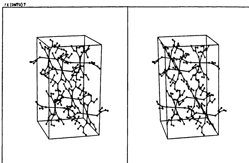
Figure 6. SHELXTL drawing of the unit cell for [\text{Fe}(\text{SC}(\text{NHCH}_3)_2)_6](\text{BF}_4)_2 \cdot \text{SC}(\text{NHCH}_3)_2 .
