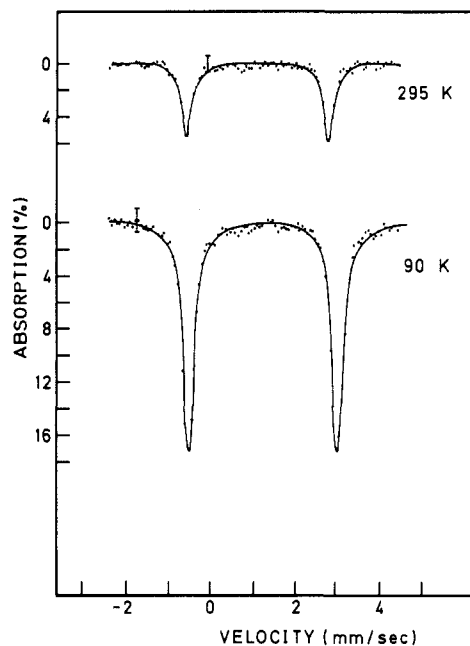
Figure 1. Mössbauer spectra for [Fe(NETU) 6 ](ClO 4 ) 2 at two temperatures. Isomer shift is referenced to Na 2 Fe(CN) 5 NO·2H 2 O (I: error bar).
