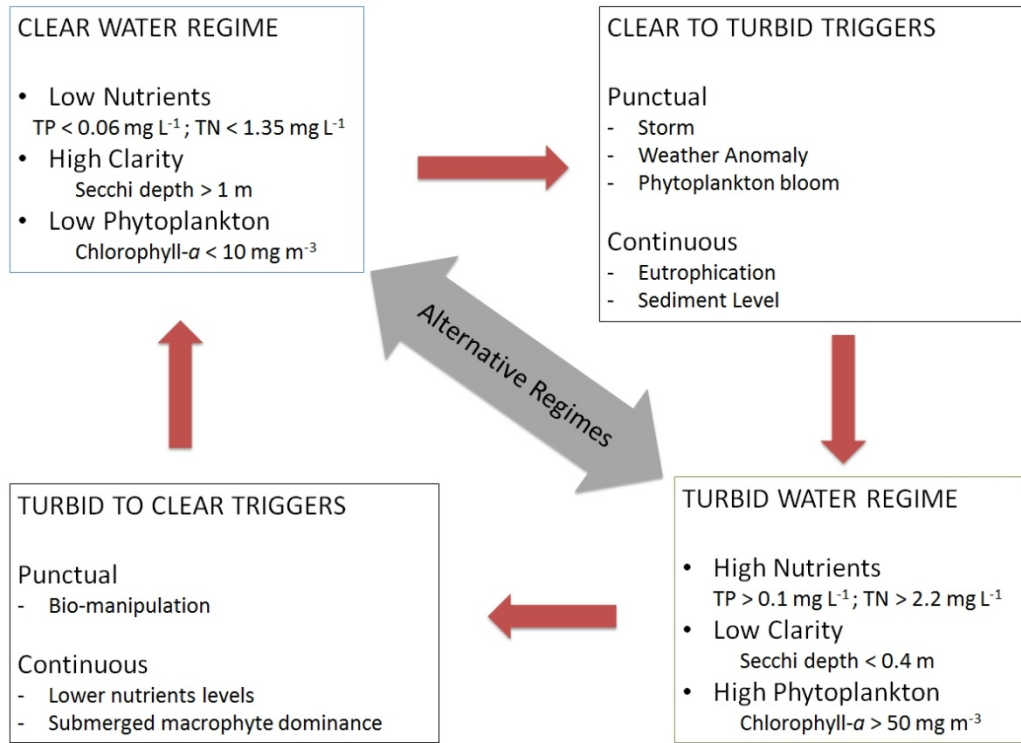
Figure 1. Simplified conceptual model of regime shifts in shallow lakes. Triggers and threshold values were taken from the literature. TP: total phosphorus, TN: total nitrogen. (modified from Tironi, 2012).
