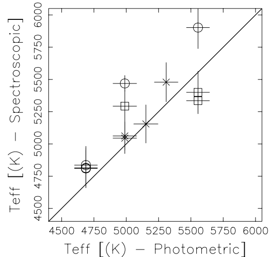
Fig. 9. A comparison between the temperature scales derived for the photometric (lithium abundance) analysis and the spectroscopic (metallicity) analysis is presented. The symbols for the SFR data source are the same as those presented in Fig. 4. The solid line is indicative of equality between the two temperature systems, and is not a fit to the data.
