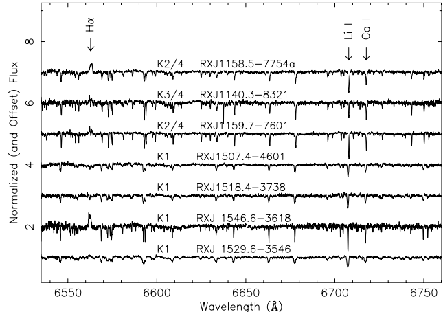
Fig. 1. Example normalized FEROS spectra are presented for a subset of the WTT candidates in the SFRs under study. The spectra are offset for clarity. Several lines of astrophysical interest are annotated, such as the Balmer H\alpha line at 6562.8 \text{\AA} as well as the Li I (6707.8 \text{\AA} ) and Ca I (6717.7 \text{\AA} ) lines.
