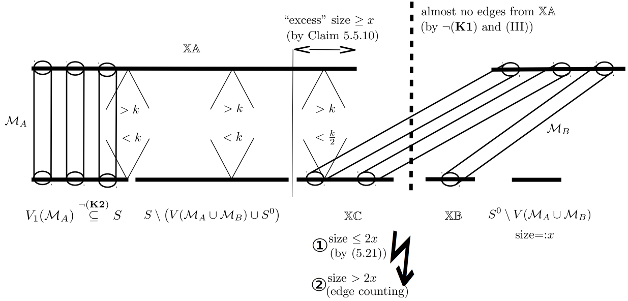
Figure 5.4: A simplified computation showing that \neg(\mathbf{K1}) , \neg(\mathbf{K2}) leads to a contradiction. Denoting by x the size of S^0 \setminus V(\mathcal{M}_A \cup \mathcal{M}_B) we get \textcircled{1} |\mathbb{X}\mathbb{C}| \leq 2x . On the other hand, each vertex of \mathbb{X}\mathbb{A} emanates \gtrsim k edges which are absorbed by the sets V_1(\mathcal{M}_A) , S \setminus (V(\mathcal{M}_A \cup \mathcal{M}_B) \cup S^0) , and \mathbb{X}\mathbb{C} . The vertices of V_1(\mathcal{M}_A) and S \setminus (V(\mathcal{M}_A \cup \mathcal{M}_B) \cup S^0) can absorb \lesssim k edges. The vertices of \mathbb{X}\mathbb{C} receive \lesssim \frac{k}{2} edges of \mathbb{X}\mathbb{A} by (5.24). This leads to \textcircled{2} |\mathbb{X}\mathbb{C}| > 2x , doubling the size of the “excess” vertices of \mathbb{X}\mathbb{A} .
