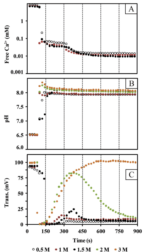
Fig. 1. Graphs showing the variations in free calcium (A), pH (B) and turbidity (C) of the gypsum-saturated solutions due to the addition of DAP at concentrations of 0.5, 1, 1.5, 2 and 3 M.
