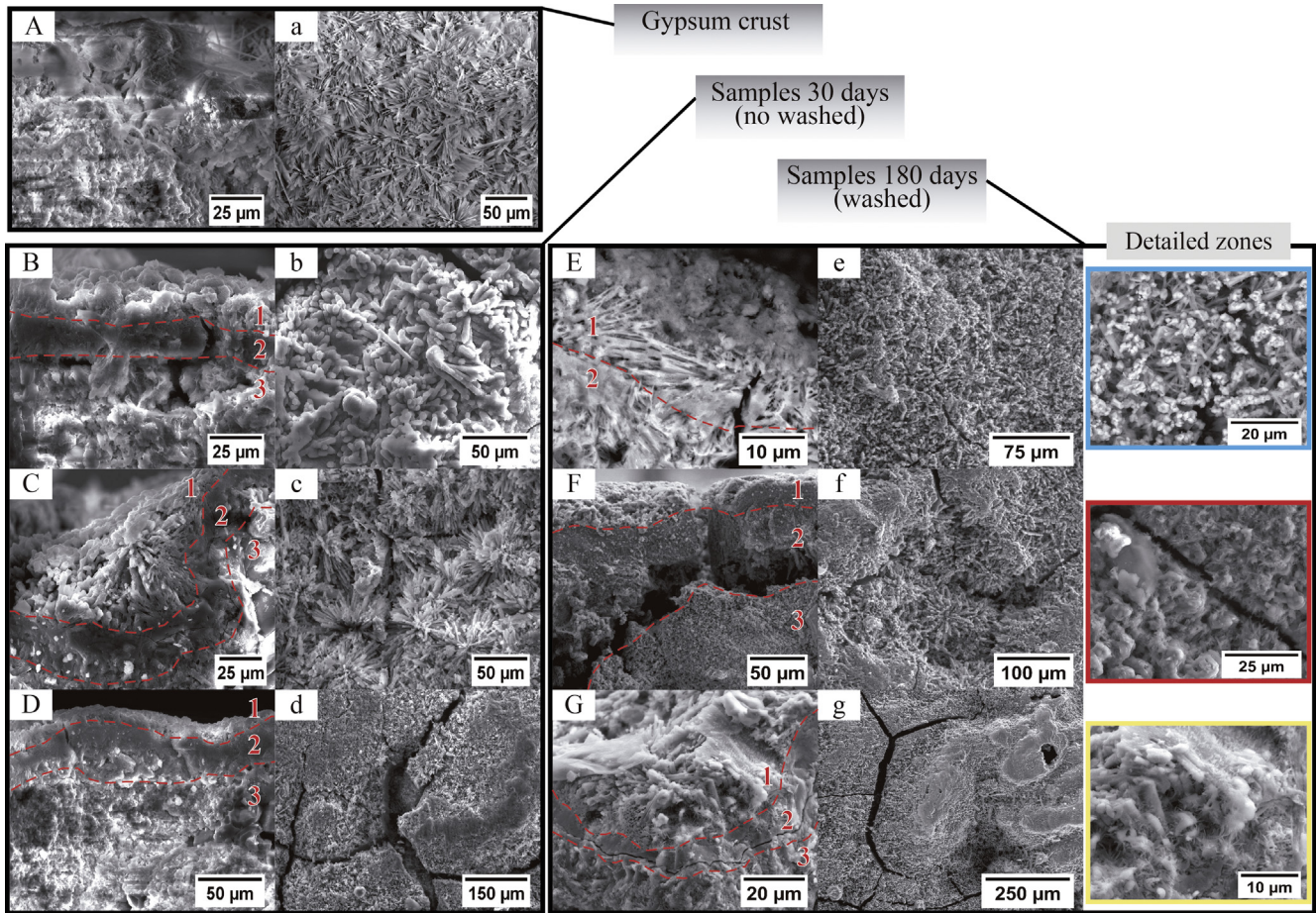
Fig. 9. ESEM microphotographs of the profile (uppercase letters) and of the surface (lowercase letters) of the gypsum crust (A-a), of the samples treated after 30 days, before being washed (B-b, C-c and D-d) and after being washed after 180 days of treatment (E-e, F-f and G-g). The images are of the 30 m (B-b and E-e), 60 m (C-c and F-f) and 240 m (D-d and G-g) samples. Legend: 1, replacement crust; 2, massive level of CaPs; 3, carbonate substrate.
