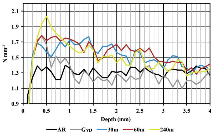
Fig. 10. Average values for resistance to microdrilling ( R_p , in N/mm ) of the healthy sample (AR), the altered sample with the gypsum crust (Gyp) and the samples treated for 30, 60 and 240 min (30 m, 60 m and 240 m, respectively).
