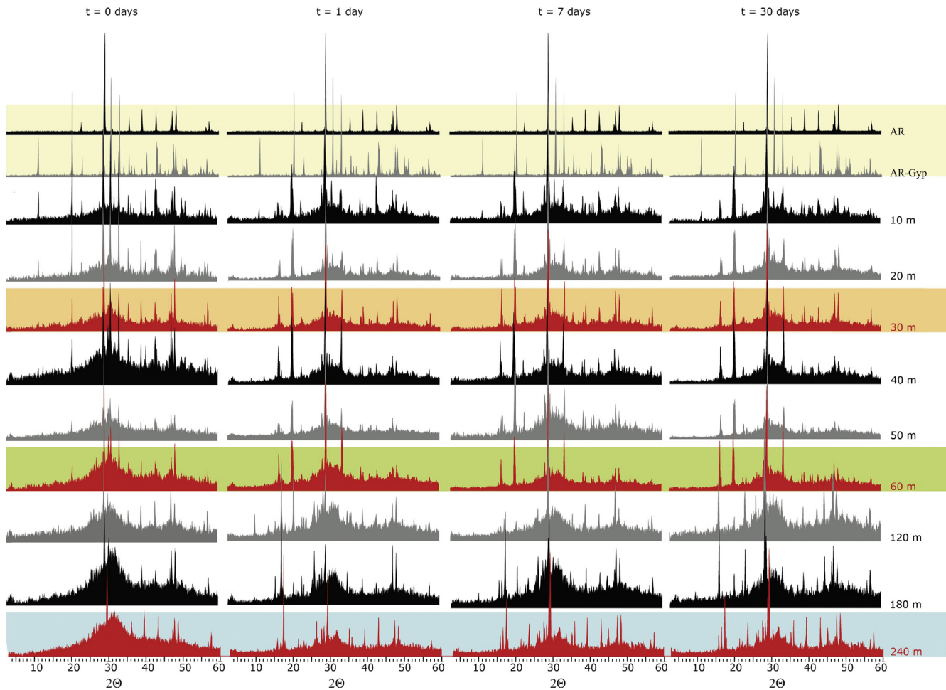
Fig. 2. Evolution of the consolidant assessed using XRD over the first 30 days after application of DAP using a poultice at different application times (10 m, 20 m, 30 m, 40 m, 50 m, 60 m, 120 m, 180 m and 240 m) and compared to the healthy sample (AR) and the altered sample with the gypsum crust (AR-Gyp).
