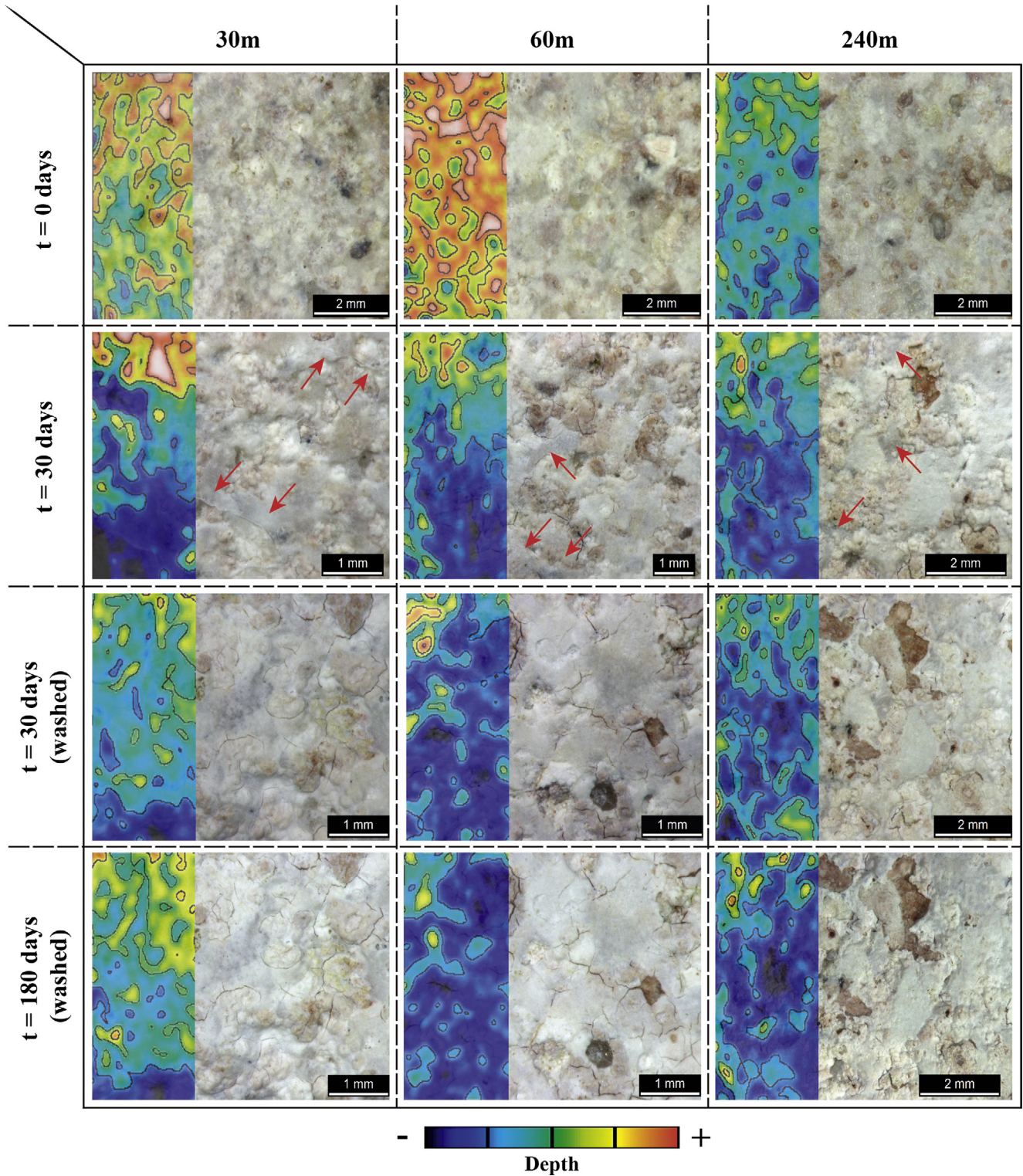
Fig. 8. Images of the surface and the roughness obtained using VDM of the 30 m, 60 m and 240 m samples when the poultice with DAP was removed ( t = 0 days), after a month before ( t = 30 days) and after ( t = 30 days (washed)) washing and finally after six months ( t = 180 days (washed)). The color scale indicates in relative values the homogeneity of the roughness registered on the surface.
