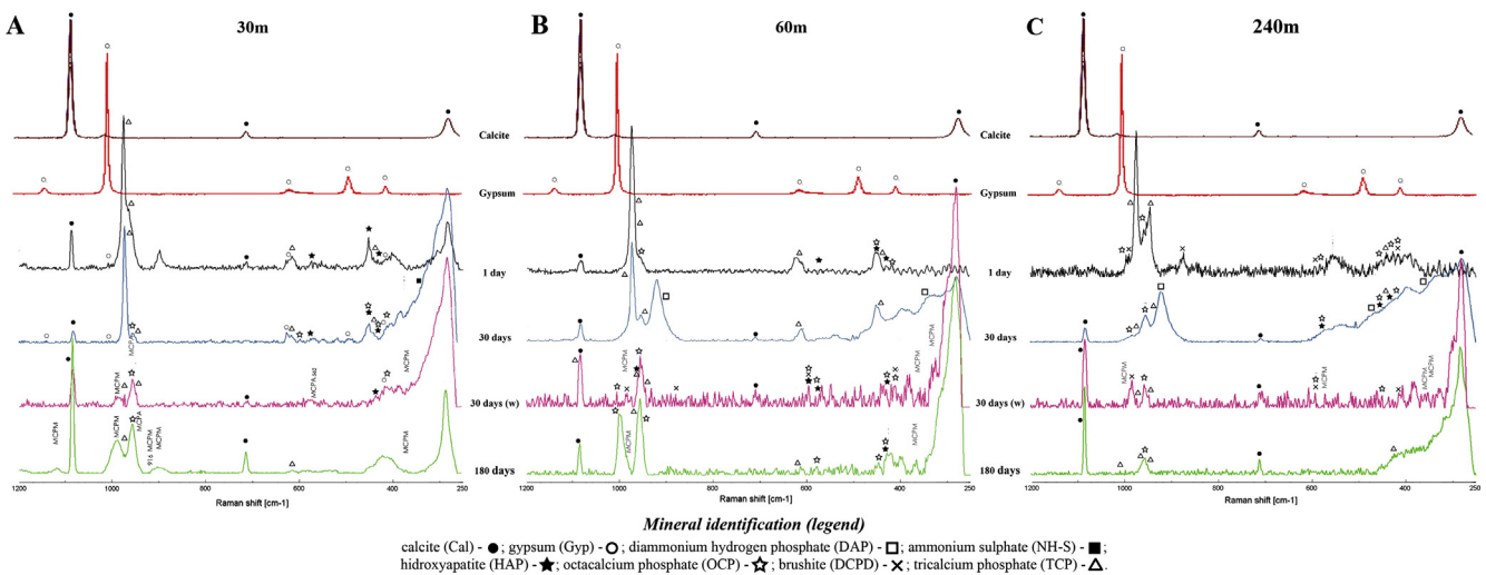
Fig. 5. Raman spectra of the calcite and gypsum standards (RRUFF) of the 30 m, 60 m and 240 m samples (A, B and C, respectively) after one day (1 day), one month before (30 days) and after (30 days (w)) washing and finally after six months (180 days). The mineral legend is indicated in the figure.
