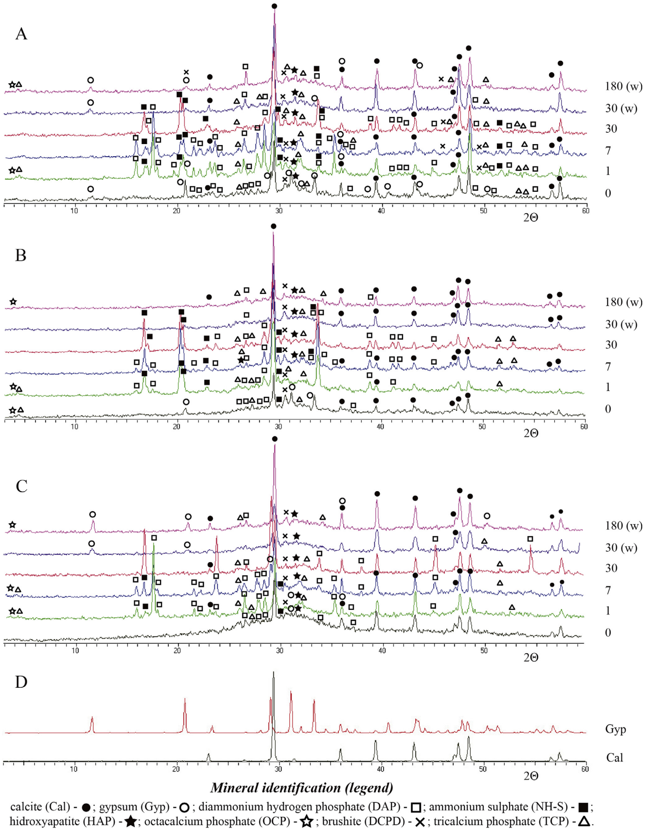
Fig. 3. Evolution of the consolidant (DAP 3 M) assessed using XRD in the 30 m (A), 60 m (B) and 240 m (C) samples and the standards for gypsum and calcite (Gyp and Cal, D). The measurements were taken immediately after removing the poultice (0), one day later (1), one week later (7), one month later before and after washing the samples (30 and 30 (w), respectively) and six months later (180 (w)). The following mineral identification cards were used: calcite “5-586”, gypsum “21-816”, phosphammite (dibasic ammonium phosphate) “29-111”, hydroxylapatite “9-432”, tricalcium phosphate (V) and whitlockite “86-1585 and 9-169, respectively”, calcium hydrogen phosphate hydrate and calcium hydrogen phosphate (octacalcium phosphate “26-1056 and 79-423, respectively”, brushite “4-740” and ammonium sulphate “1-343”.
