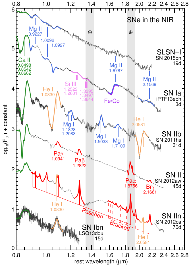
Figure 4. Atlas of NIR spectra of various SN types. The dominant ion species are labeled for reference and comparison. The laboratory wavelengths are labeled in microns for reference and also marked on the figure as vertical lines. The supernova name and phase are labeled for each spectrum. The phases are relative to maximum light, except for that of SN 2012aw, which is relative to explosion. The gray vertical bands mark the regions of the strongest telluric absorptions. All spectra shown were taken with FIRE as part of the CSP-II NIR spectroscopy program. Spectra of iPTF13ebh (Hsiao et al. 2015), SN 2011hs (Bufano et al. 2014), SN 2012aw (Dall’Ora et al. 2014), and SN 2012ca (Fox et al. 2015) were published previously. FIRE spectra of the SLSN-I SN 2015bn and the Type Ibn LSQ13ddu are shown for the first time.
