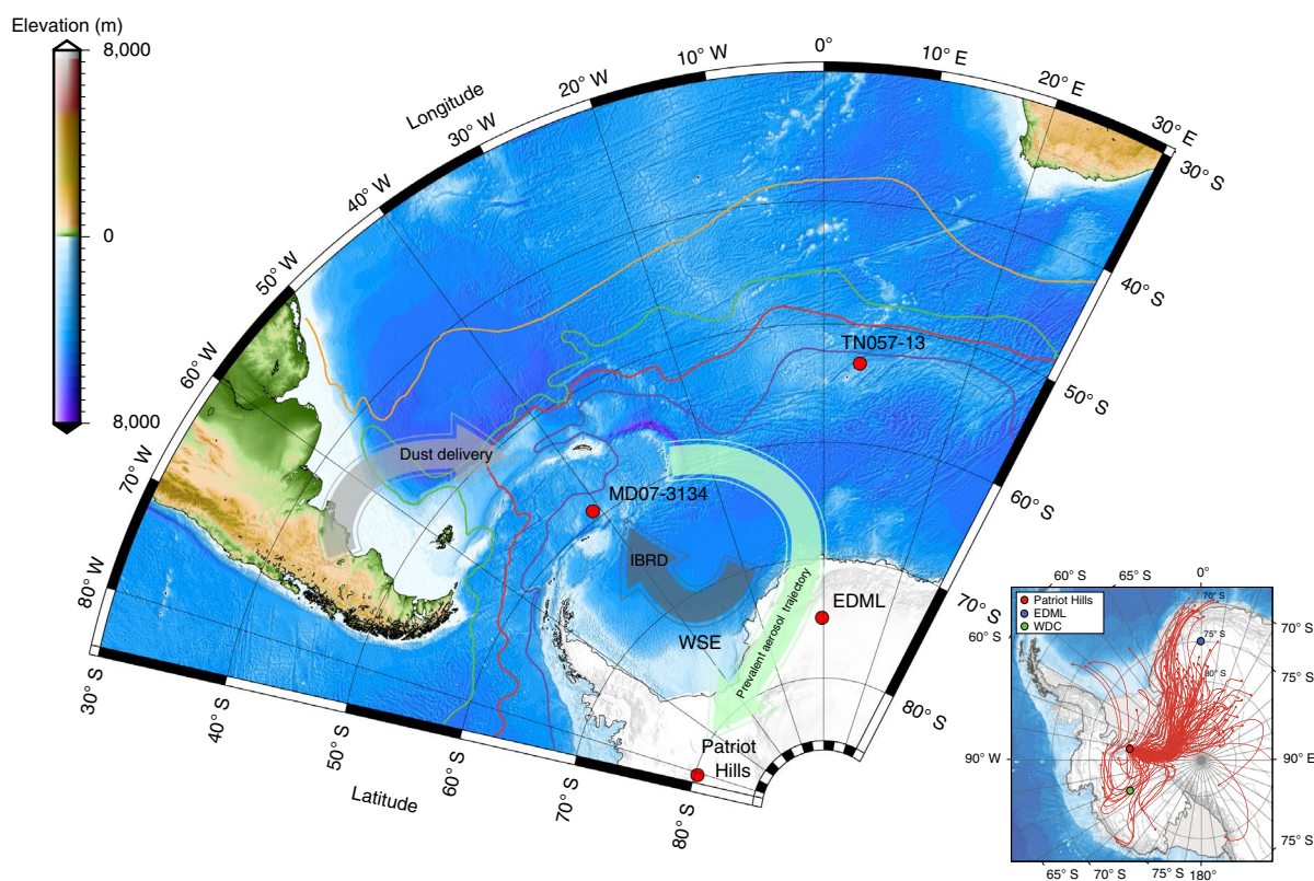
Fig. 2 | The South Atlantic sector of the Southern Ocean with the locations of the Patriot Hills in the Ellsworth Mountains, the EDML ice core and marine cores MD07-313421 and TN057-134. Positions of the southern limb of the Antarctic Circumpolar Current (purple line), the Polar Front (red), Subantarctic Front (green) and the Subtropical Front (yellow) 53 . The grey arrow denotes the primary route of iceberg-rafted debris (IBRD) in the Weddell Sea Embayment (WSE), and the green arrow depicts the prevalent aerosol trajectory to the Patriot Hills site. Inset, monthly grouped 72 h atmospheric back-trajectories for the Patriot Hills (November 2009), from the NOAA HySPLIT 54 , with WDC and EDML 52 ice cores. South Pole stereographic basemap produced in Generic Mapping Tools v5.4.5 (ref. 55 ) with the NOAA ETOPO1 Ice Surface dataset.
