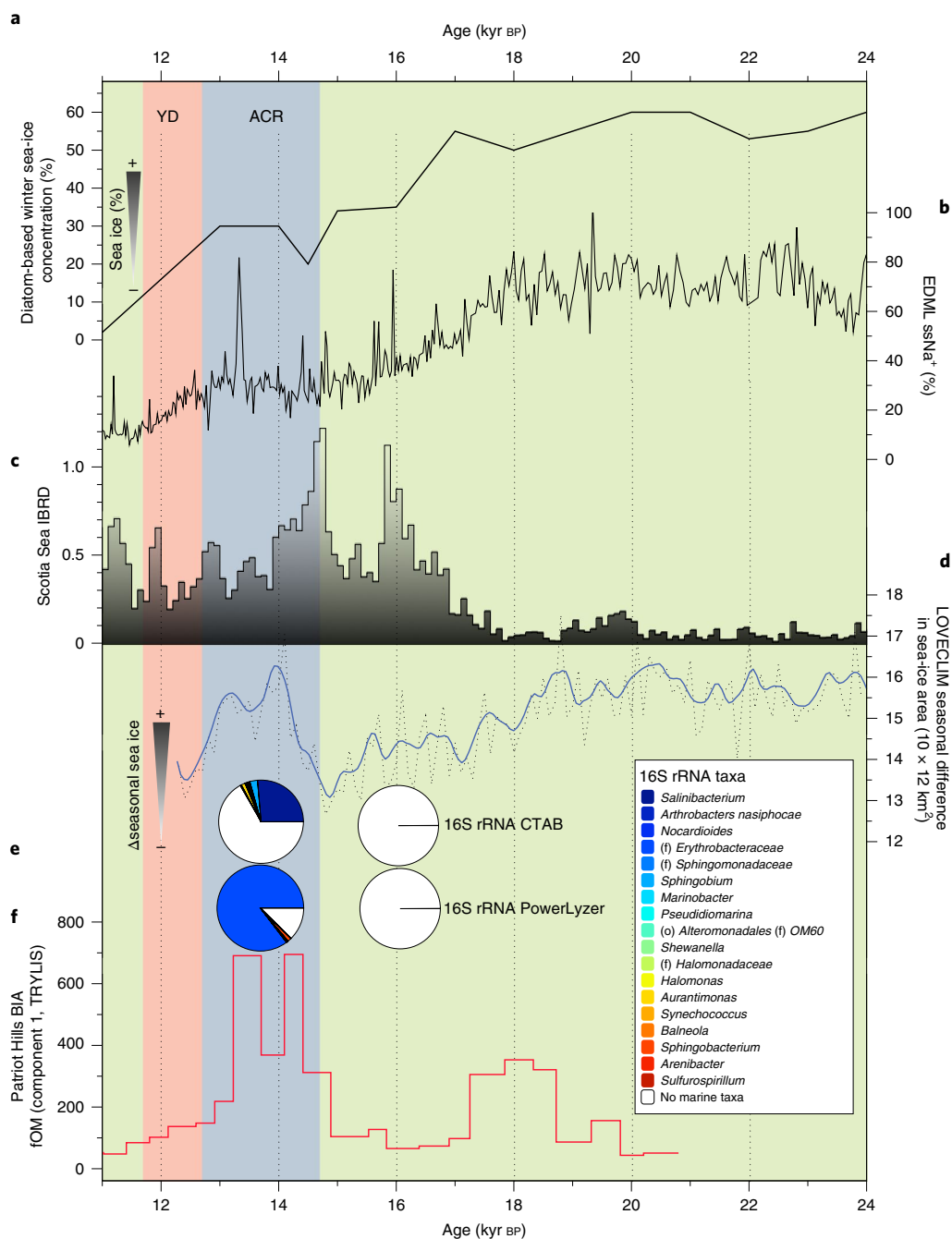
Fig. 5 | Regional climate proxy and model intercomparisons with the Patriot Hills record. a , Diatom transfer function-based winter sea-ice concentration 41 . b , Sea salt (ssNa + ) from EDML 52 . c , Iceberg-rafted debris (IBRD) from MD07-3134 21 (normalized 100 yr, relative to the Holocene). d , Modelled seasonal difference in Antarctic sea-ice area (LOVECLIM 42 ). e , Percentage marine microorganisms from 16S rRNA CTAB extraction (top) and PowerLyzer (bottom). f , FOM concentration (component 1; TRY LIS). Vertical boxes indicate the ACR (blue) and YD chronozones (11.7–12.7 kyr BP).
