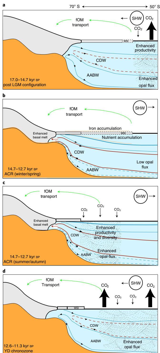
Fig. 6 | Schematic depicting events across mid- to high-latitude Southern Ocean during the LGT. a, Post-Last Glacial Maximum (LGM). Displacement of the Southern Hemisphere westerlies (SHW) enhances overturning of mid-latitude Southern Ocean between ~17 and 14.7 kyr BP evidenced by opal flux 4 . b, ACR. Enhanced intrusion of Circumpolar Deepwater (CDW) and winter sea-ice (WSI) expansion (winter/spring winter). Increased stratification, mixed layer deepening and reduction in AABW 40 . c, ACR (summer/autumn) during which the WSI breakup enhances CO 2 drawdown at high latitudes. d, YD chronozone, with reinvigorated mid-latitude overturning and degassing of old CO 2 enhancing opal flux.
