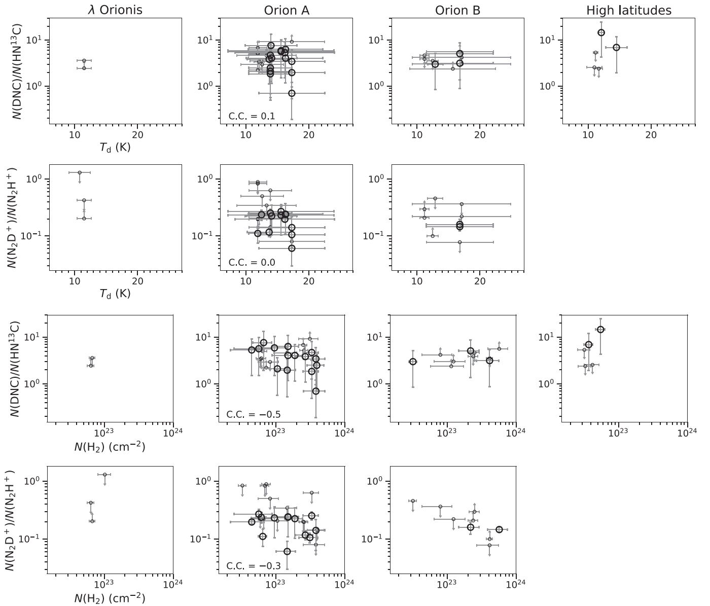
Figure 7. Column density ratios of DNC/HN 13 C and N 2 D + /N 2 H + are plotted against the dust temperature and H 2 column density for local (<1 kpc) starless cores in different environments. The meanings of the symbols and C.C. are the same as those used in Figure 6.
