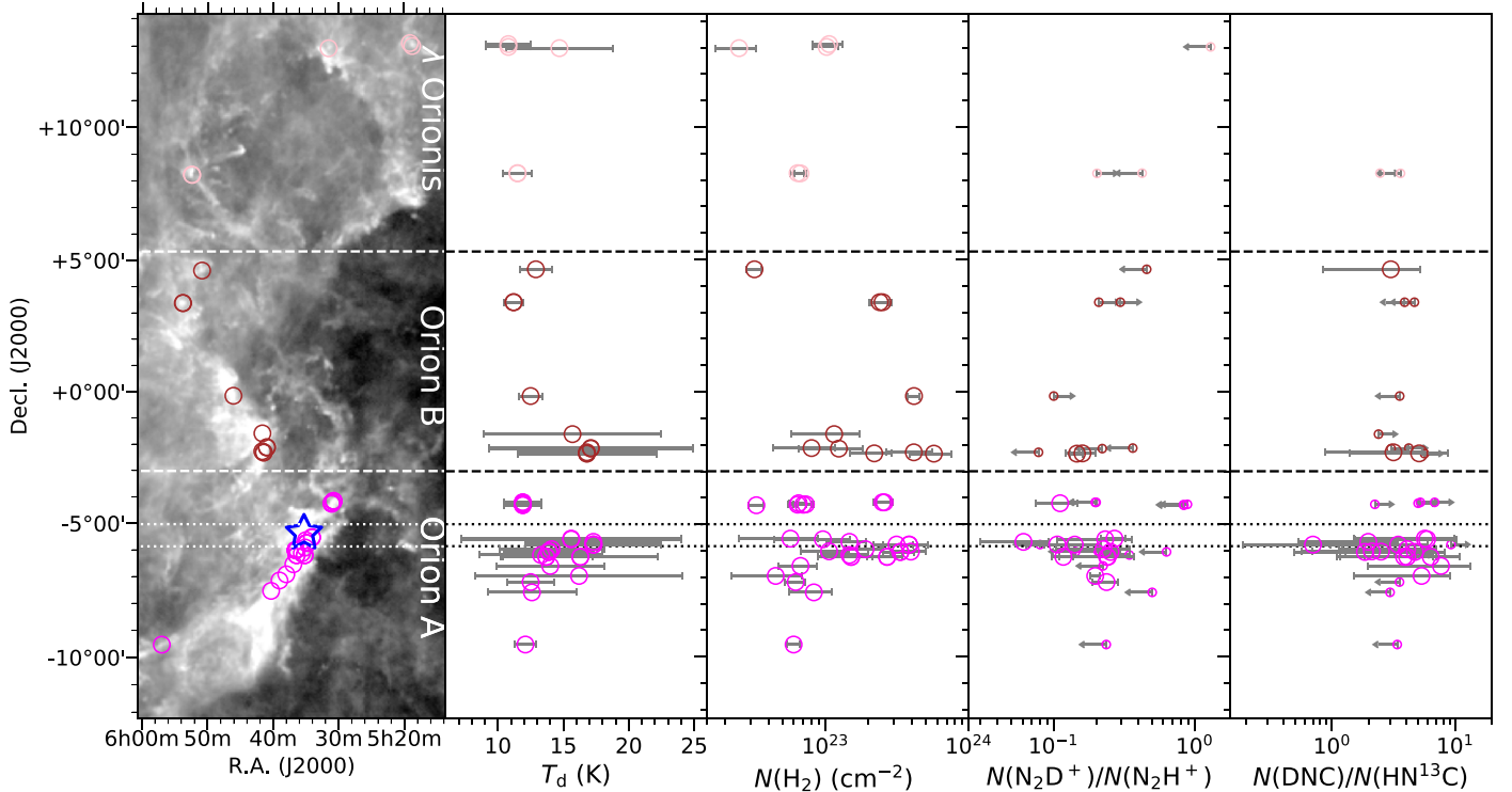
Figure 9. Spatial distribution, dust temperature, H_2 column density, N(N_2D^+)/N(N_2H^+) , and N(DNC)/N(HN^{13}C) against declination for starless cores in the Orion region. The large symbol with an error bar and the small symbol with an arrow are the same as those used in Figure 6. The background image in the left panel is the Planck 850 \mu m dust continuum map. The blue star symbol in the left panel represents the position of the Orion Nebula (R.A., decl. = 05^h35^m17^s.3 , -05^\circ23'28'' ). The dashed horizontal lines represent the boundaries of \lambda Orionis, Orion B, and Orion A. The dotted horizontal lines represent the boundaries of the potential impact zone of the Orion Nebula on the declination.
