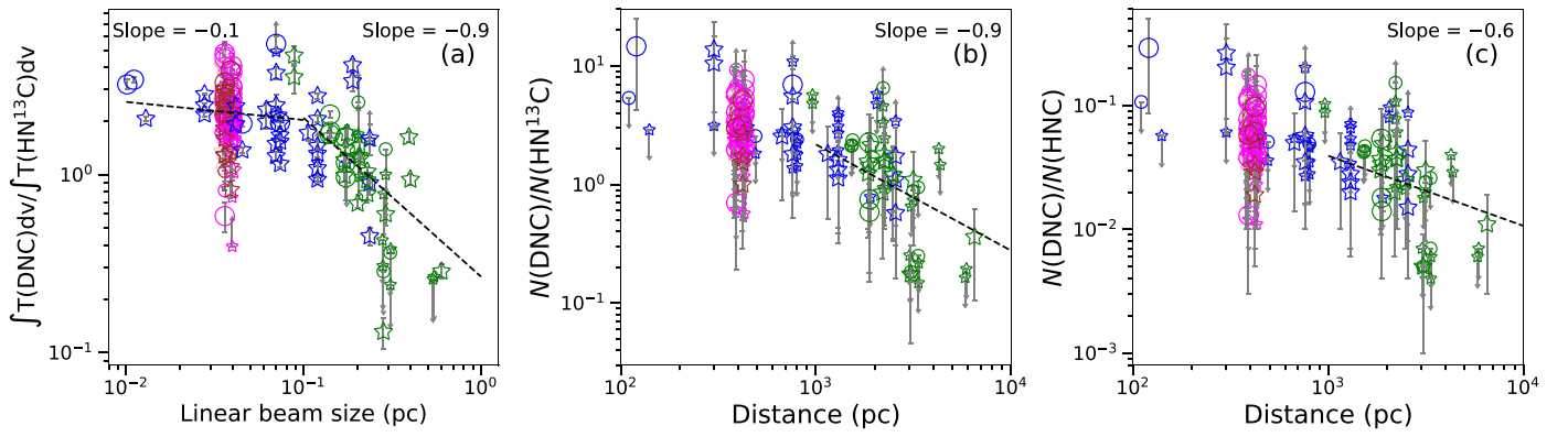
Figure 5. (a) Integrated intensity ratio of DNC to \text{HN}^{13}\text{C} plotted against the linear beam size. (b) Column density ratio of \text{DNC}/\text{HN}^{13}\text{C} plotted against distance. (c) Same as panel (b), but for \text{DNC}/\text{HNC} . The color symbols represent SCUBA-2 cores in \lambda Orionis (pink), Orion A (magenta), Orion B (brown), the Galactic plane (green), and at high latitudes (blue). The circle and star symbols represent the starless and protostellar core, respectively. The large symbol with the error bar represents the dense core where both values in the ratio are successfully estimated. The small symbol with the arrow represents the dense core with upper or lower limits. The dashed line with the slope value represents the least-squares fitting to the cores detected in both molecular lines. In panel (a), the fittings are made for linear beam sizes of \leq 0.1 pc and of > 0.1 pc separately. In panels (b) and (c), the fittings are made for distances of > 1 kpc.
