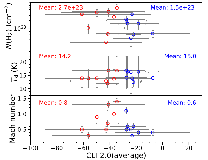
Figure 12. H 2 column density, dust temperature, and Mach number against average CEF2.0 for starless cores in the Orion region. Red and blue represent starless cores with average CEF2.0 of < -33 and \geq -33 , respectively.
