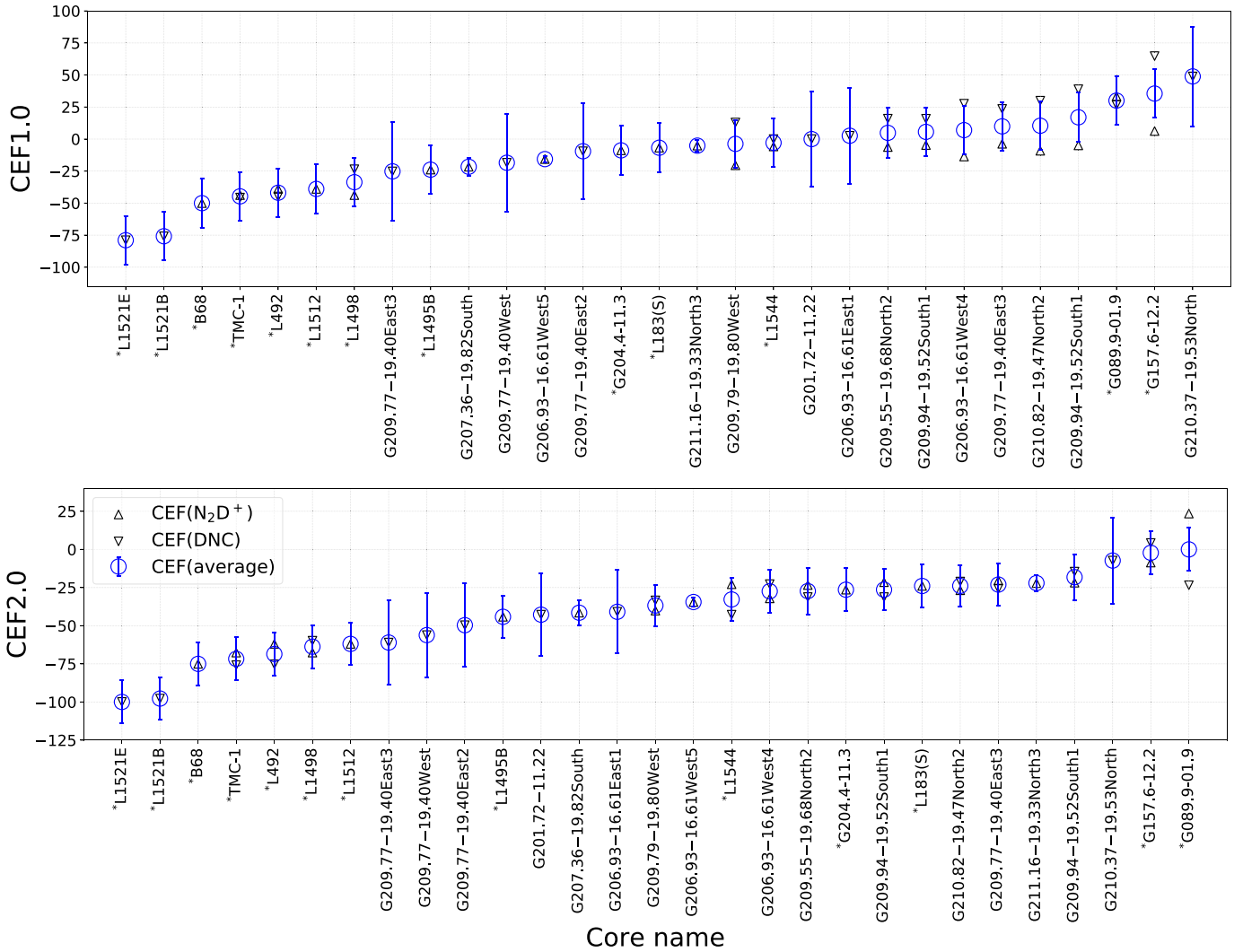
Figure 10. CEF for starless cores in the Orion region and for local (<1 kpc) starless cores studied in Tatematsu et al. (2017) in ascending numeric order of the average CEF. The top and bottom panels show CEF1.0 derived by the equations in Tatematsu et al. (2017) and CEF2.0 by our study, respectively. The source name with the asterisk represents the cores taken from Tatematsu et al. (2017).
