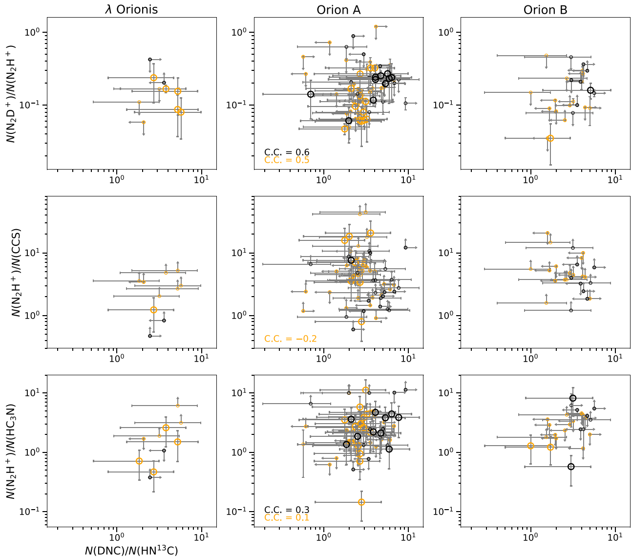
Figure 6. Column density ratios of N_2D^+/N_2H^+ , N_2H^+/CCS , and N_2H^+/HC_3N plotted against that of DNC/HN^{13}C for SCUBA-2 cores in \lambda Orionis, Orion A, and Orion B. Black and orange represent starless and protostellar cores, respectively. The large symbol with the error bar represents the dense core where both column densities in the ratio are successfully estimated. The small symbol with the arrow represents the dense core with either upper or lower limits. C.C. represents the correlation coefficient; we show the C.C. only when both the pairing column densities are successfully estimated for seven or more dense cores. C.C. does not take into account outliers in the sample.
