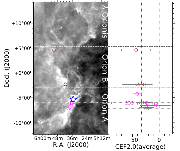
Figure 11. Same as Figure 9, but for the spatial distribution and average CEF2.0 against declination for starless cores in the Orion region. The vertical lines represent CEF2.0 of -33 and 0 . The horizontal dotted lines represent declination of -7^\circ 2 and -5^\circ 9 .
