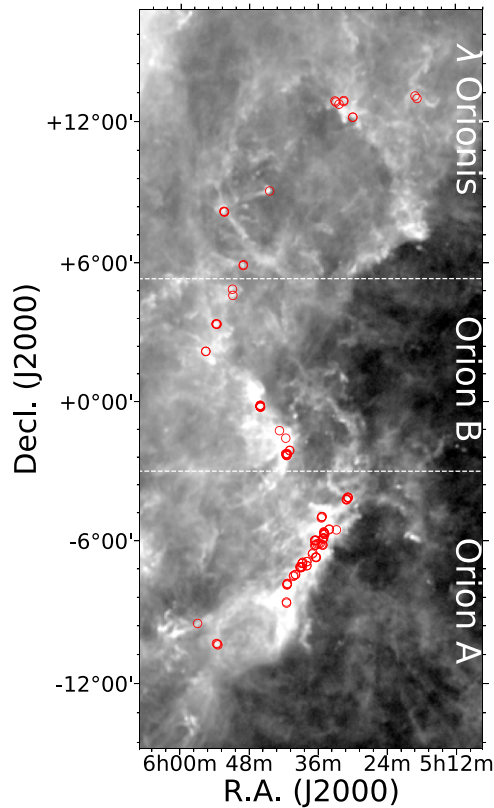
Figure 2. Spatial distribution of SCUBA-2 cores in the Orion region. The background image is the Planck dust continuum map at 850 \mu\text{m} with a size of 15^\circ \times 30^\circ . The symbol is the same as those used in Figure 1. The horizontal lines represent the boundaries for three subregions ( \lambda Orionis, Orion A, and Orion B).
