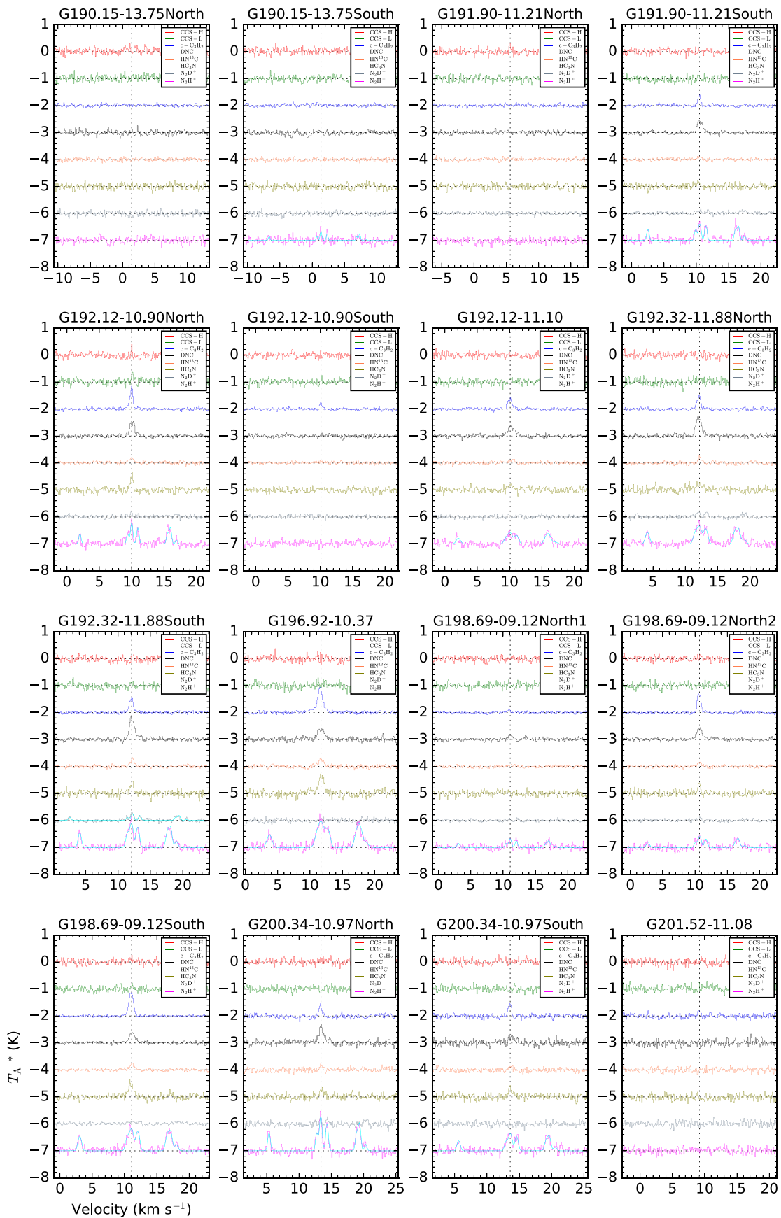
Figure 3. Spectra of 207 SCUBA-2 cores in PGCC cores in eight molecular lines. A vertical line indicates a systemic velocity. A horizontal line represents 0 K in T_A^* scale. For the N_2H^+ and N_2D^+ emission, the cyan line represents the hyperfine structure fitting result.
