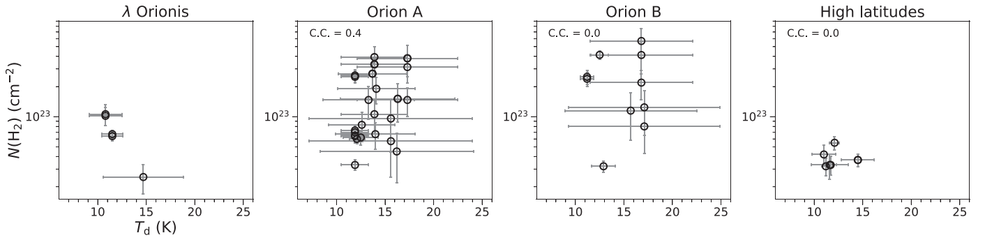
Figure 8. H_2 column density plotted against dust temperature for local ( <1 kpc) starless cores in different environments. The meanings of the symbols and C.C. are the same as those used in Figure 6.
