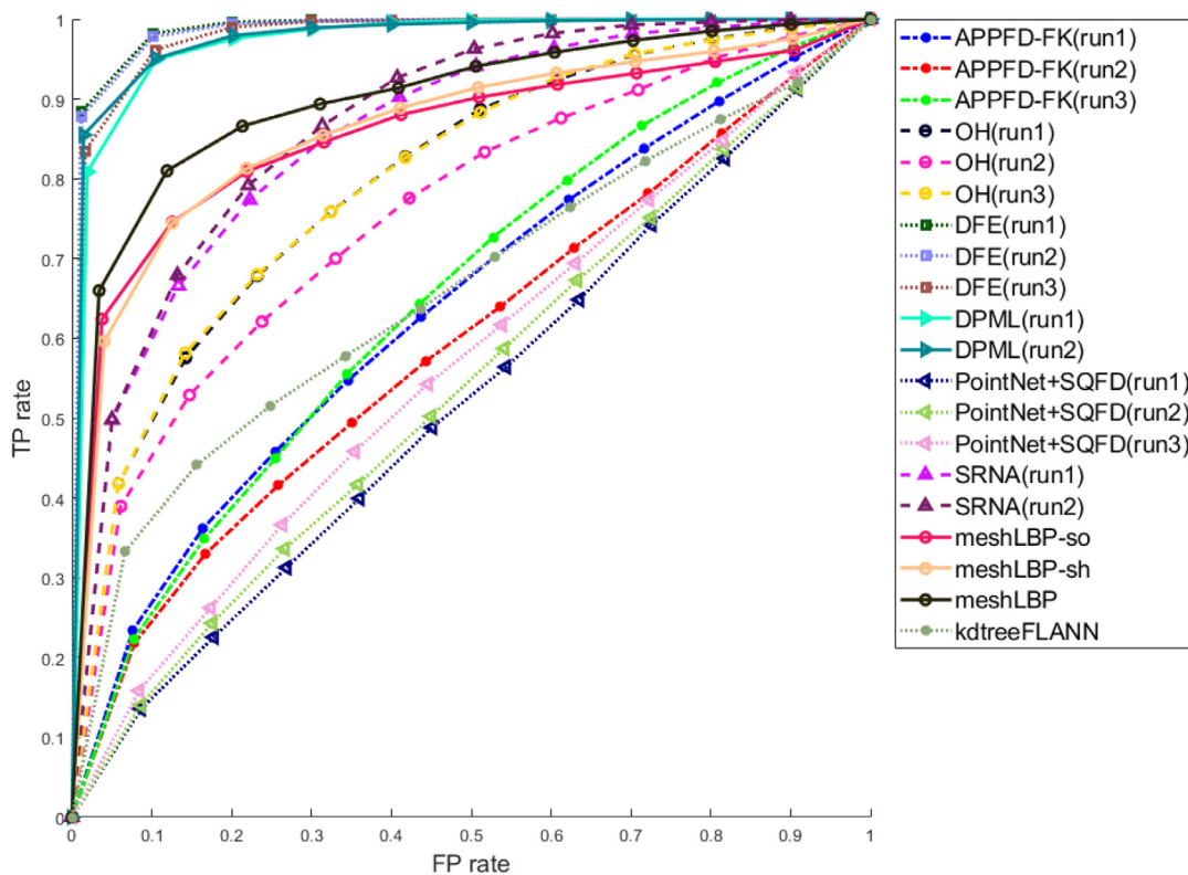
ROC curves
