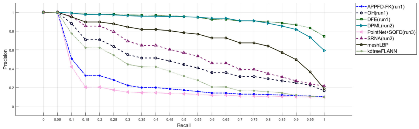
Fig. 17. Overview of Precision-Recall plots of the best run for each method.
