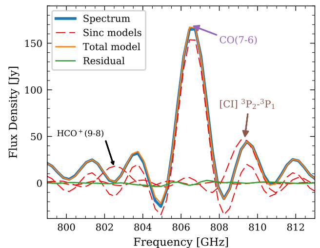
Figure 9. Sample NGC 7027 spectrum demonstrating the close proximity of the ^{12}\text{CO}(7-6) and [\text{C}]\ ^3\text{P}_2 - ^3\text{P}_1 features.
