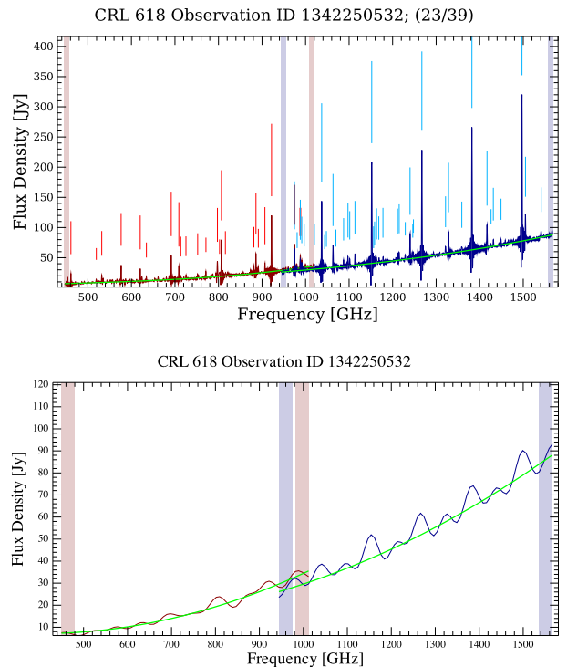
Figure 4. An example of an HR sparse FF postcard (top) and a LR postcard (bottom) for an observation taken in H+LR mode. The HR spectrum shows a rich compliment of spectral features, heavily smoothed out in the LR version. The SLW and SSW band edge regions are outlined by full-height vertical bars. The polynomial continuum fit is shown in green. The vertical sticks in the upper figure represent features identified by the FF, with height proportional to the SNR of the identified feature.
