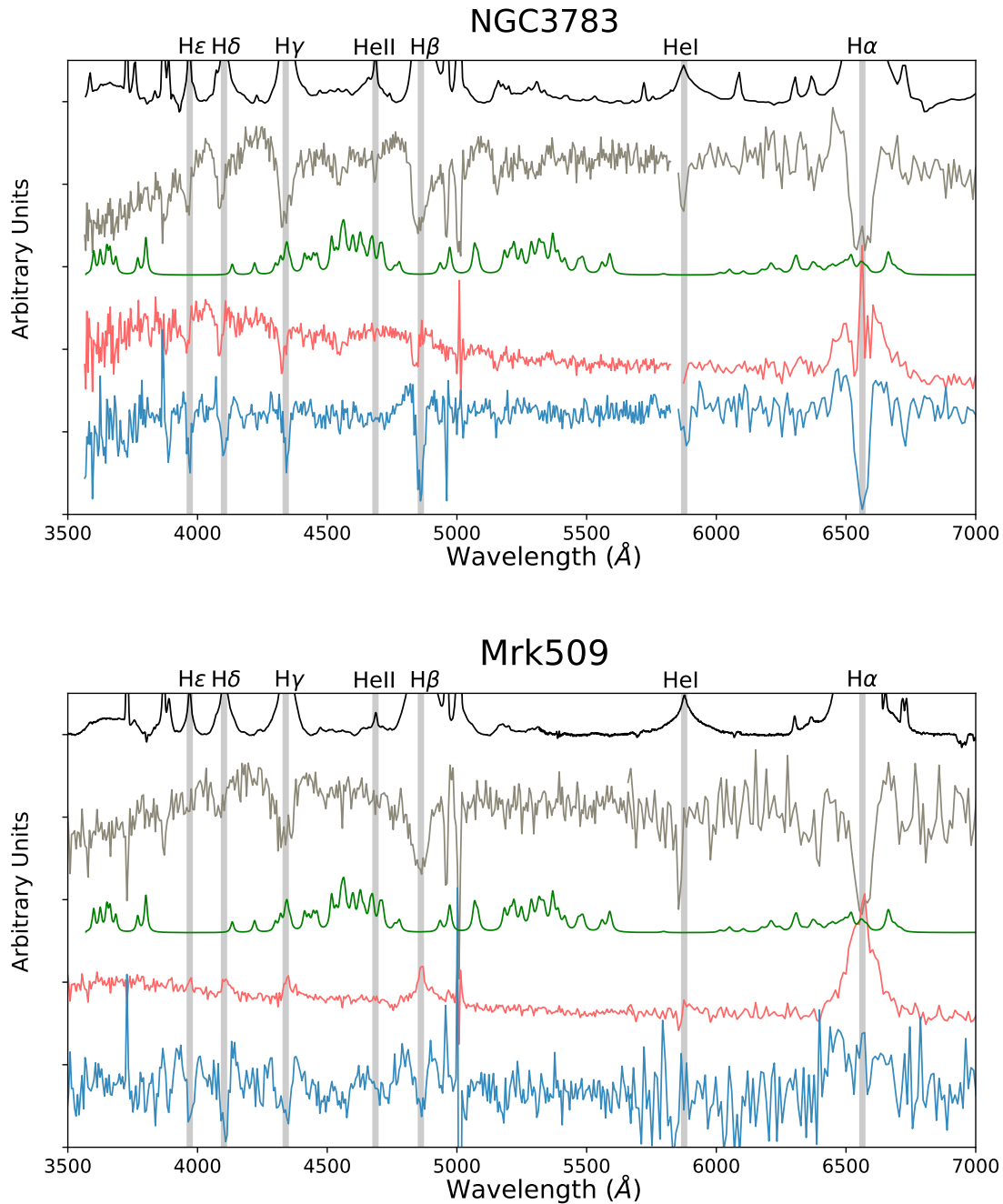
Figure 4. I (black), p (grey), p \times I (red), and PA (blue) spectra for NGC3783 (top) and Mrk509 (bottom). A FeII template has also been included (green). The I spectra have been continuum subtracted to allow for a better inspection of the line positions. The FeII flux template is based on I Zw 1 (kindly provided by M. Vestergaard; for more details see Vestergaard & Peterson 2005). Vertical lines have been drawn to coincide with the central wavelength of the Balmer and He emission lines.
