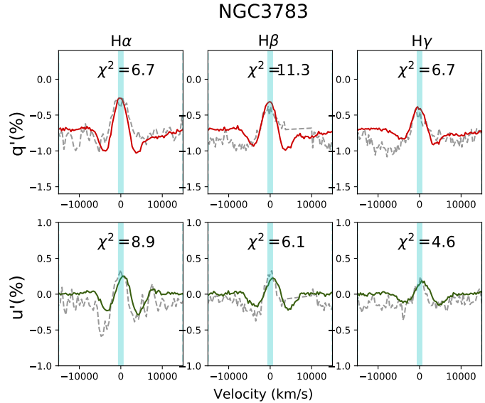
Figure A1. Best fit model for NGC 3783 q' and u' spectra (top and bottom row, respectively). Data are shown with gray dashed lines and errors are presented as a gray region around the data. A best fit model corresponds to the model with the best sum of \chi^2 from all fits to H \alpha , H \beta and H \gamma . Data between -15000 and +15000 km/s from the line centers were considered in the fits, with the OIII lines masked out bluewards of H \beta .
