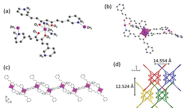
Fig. 3 Crystal structure of 1 : (a) Representation of the coordination sphere of a Zn II centre and the coordination modes of 3pyCCMoid molecules; (b) representation of two loops connected through the intermediate Zn(II) centre; (c) extended view of one chain; (d) arrangement of four chains in the crystal. Colour legend: Zn, pink; C, grey; O, red; N, blue; H atoms are omitted for clarity.
