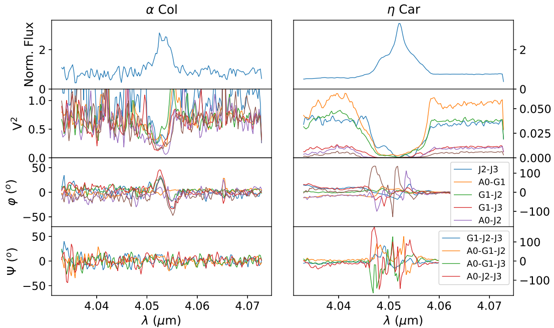
Fig. 30. MATISSE VHR ( R = 3370 ) observation of the classical Be star \alpha Col ( left ) and LBV \eta Car ( right ). From top to bottom : normalised flux in the Br \alpha line, square visibilities, differential phases and closure phases.
