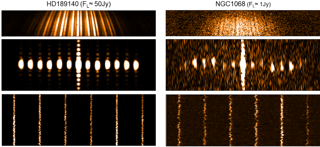
Fig. 10. Images from MATISSE’s NRTS processing for the calibrator HD 189140 and the AGN NGC 1068, both observed during MATISSE ATs commissioning on July 11, 2018. From top to bottom: clean fringes frame the mean sky removed, with FFT2D showing the fringe peaks in x as a function of the optical path difference in y , and the waterfall of the six fringe-peak vectors as a function of time (in y ) for a 1 min exposure.
