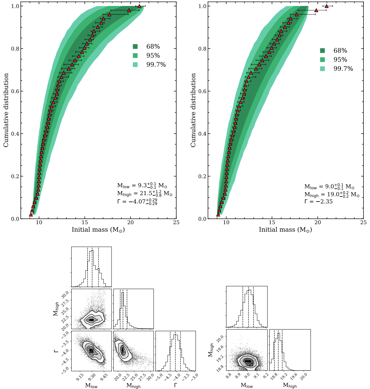
Fig. 8. Fits to the CD of M_{ZAMS} of SN II progenitors in the full sample. Top left: CD of M_{ZAMS} derived in our work for the full sample (red triangles and the error bars), corresponding to the median and the 68% confidence limit of the distribution presented in Fig. 5 as shaded contours, in comparison with the model CD constructed with the median values of the marginal distributions of the parameters (shaded contours). Bottom left: corner plot of the joint posterior probability distribution of the parameters. Dashed lines indicate the 16th, 50th, and 84th percentiles of the distributions. The right panels show the same as the left panels but when the power-law slope is fixed to \Gamma = -2.35 .
