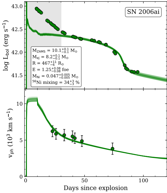
Fig. 1. Observed bolometric LC ( top panel ) and Fe II \lambda 5169 line velocities ( bottom panel ) of SN 2006ai (filled markers) with models randomly sampled from the posterior distribution of the parameters (solid lines). The median value and 68% confidence range for every physical parameter are also shown. The grey shaded region shows the early data removed from the fitting (first 30 days after explosion).
