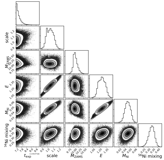
Fig. B.5. Corner plot of the joint posterior probability distribution of the parameters for SN 2006ai.
