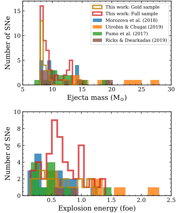
Fig. 9. Comparison of ejecta masses ( top panel ) and explosion energies ( bottom panel ) derived in the current work to those from previous studies containing large samples of SNe II.
