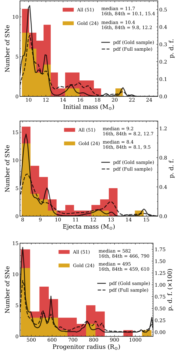
Fig. 2. Histograms of three progenitor parameters: M_{\text{ZAMS}} ( top panel ), M_{\text{ej}} ( middle panel ), and R ( bottom panel ). The gold sample is represented by yellow bars, and the red bars are the histograms for the full sample. In each panel, the number of SNe II is listed, together with the median and the 16th and 84th percentiles. Probability density functions of the physical parameters for the gold and full samples are represented by solid and dashed lines, respectively.
