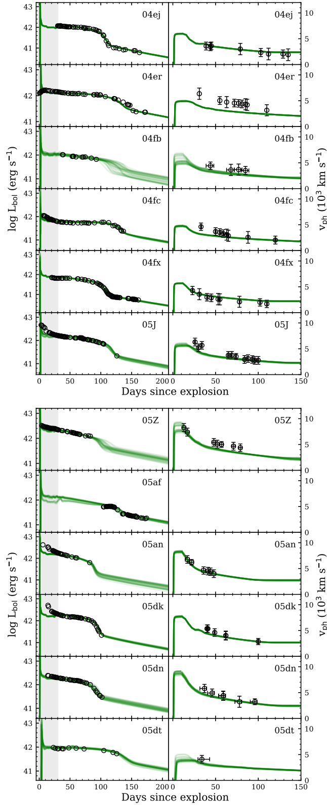
Fig. B.1. Comparison between models and observations. The open circles show the observed bolometric LCs ( left ) and Fe II velocities ( right ). Solid lines represent 30 models randomly chosen from the probability distribution. The panels present SNe in order of their discovery dates, from SN 2004ej to SN 2005dt. Grey shaded regions show the early data we removed from the fitting. The errors in the observed bolometric LCs are not plotted, for better visualisation.
