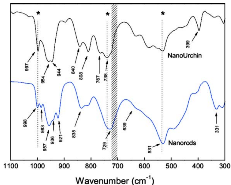
Fig. 3 (online colour at: www.pss-b.com ) Infrared spectra of the nano-urchin and nanorods of vanadium oxide. The (*) signals correspond to the bands of V_2O_5 xerogel and the shaded area corresponds to the spectral range of the surfactant vibrational modes.
